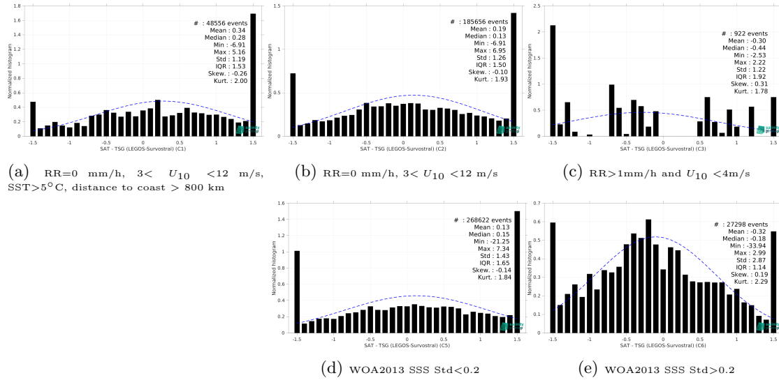
Figure 13: Normalized histogram of \Delta SSS (SMAP SSS L2 v5.0 (JPL) - TSG (LEGOS-Survostral)) for 5 different subdatasets corresponding to: RR=0 mm/h, 3 < U_{10} < 12 m/s, SST>5°C, distance to coast > 800 km (a), RR=0 mm/h, 3 < U_{10} < 12 m/s (b), RR>1mm/h and U_{10} < 4 m/s (c), WOA2013 SSS Std<0.2 (d), WOA2013 SSS Std>0.2 (e).
