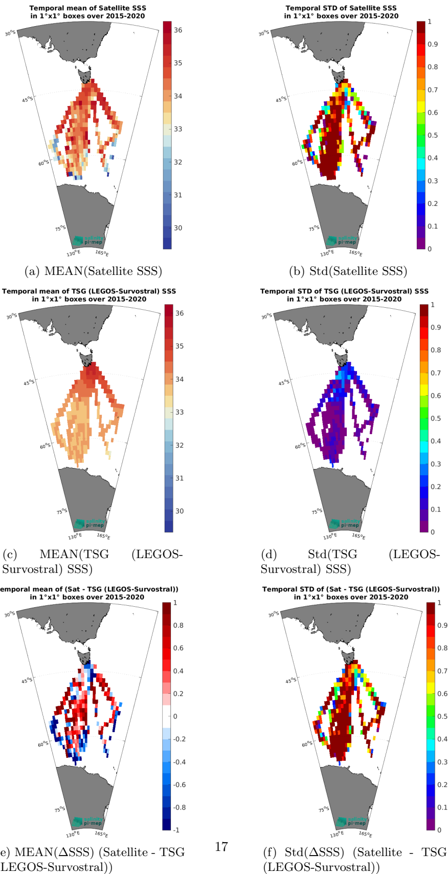
Figure 6: Temporal mean (left) and Std (right) of SSS from SMAP SSS L2 v5.0 (JPL) (top), TSG (LEGOS-Survostral) (middle), and of \Delta SSS (Satellite - TSG (LEGOS-Survostral)). Only match-up pairs are used to generate these maps.
