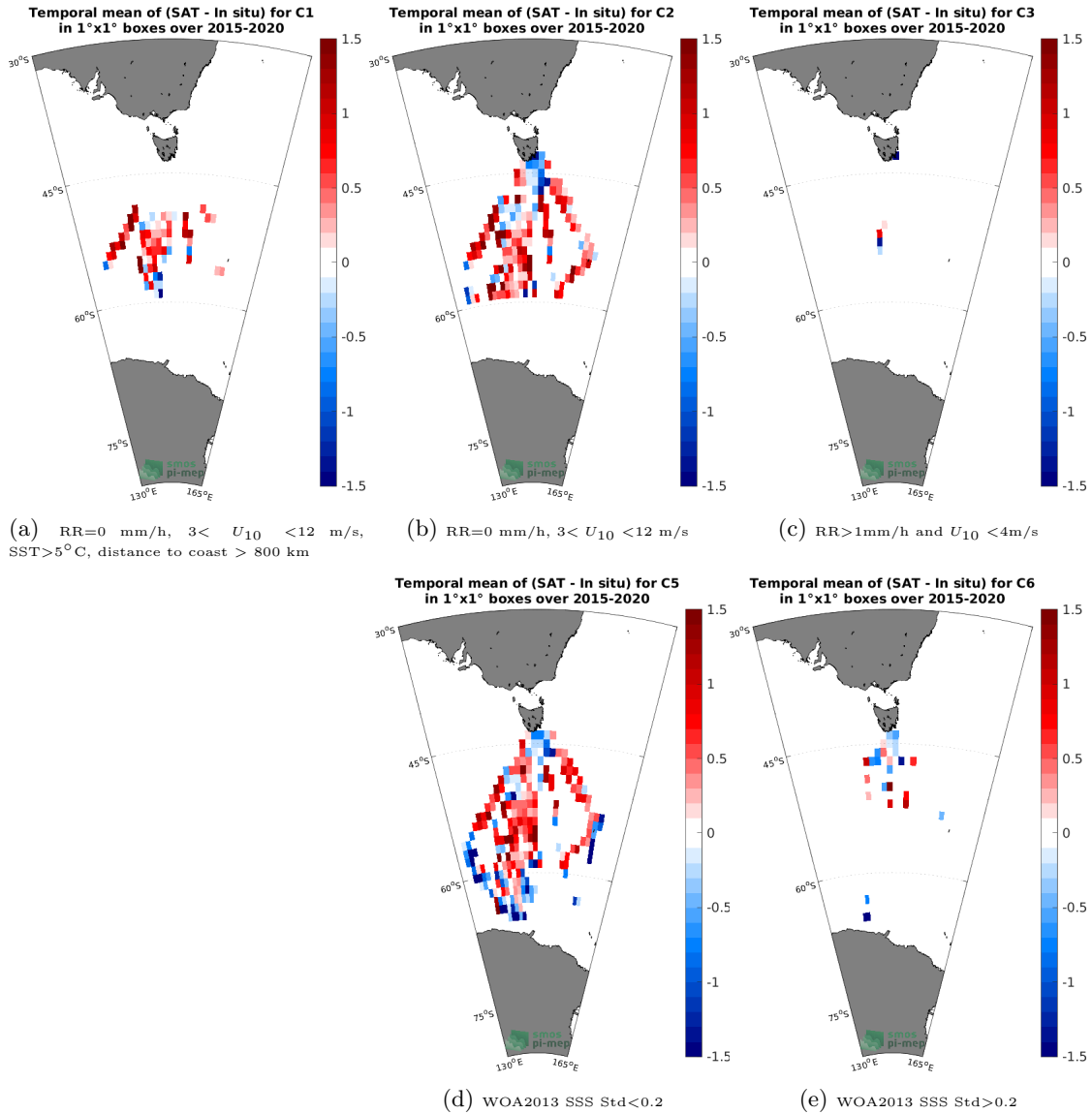
Figure 12: Temporal mean gridded over spatial boxes of size 1^\circ \times 1^\circ of \Delta\text{SSS} (SMAP SSS L2 v5.0 (JPL) - TSG (LEGOS-Survostral)) for 5 different subdatasets corresponding to: RR=0 mm/h, 3 < U_{10} < 12 m/s, SST > 5^\circ\text{C} , distance to coast > 800 km (a), RR=0 mm/h, 3 < U_{10} < 12 m/s (b), RR > 1 mm/h and U_{10} < 4 m/s (c), WOA2013 SSS Std < 0.2 (d), WOA2013 SSS Std > 0.2 (e).
