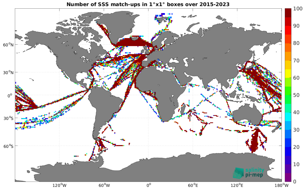
Figure 5: Number of SSS match-ups between TSG (LEGOS-DM) SSS and the SMAP SSS L2 v5.0 (JPL) SSS product for the Global Ocean Pi-MEP region over 1^\circ \times 1^\circ boxes and for the full satellite product period.
