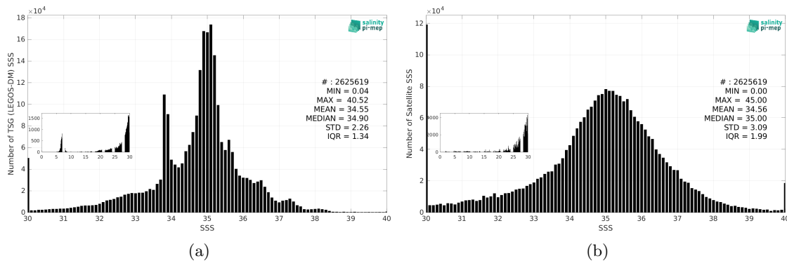
Figure 3: Histograms of SSS from TSG (LEGOS-DM) (a) and SMAP SSS L2 v5.0 (JPL) (b) considering all match-up pairs per bins of 0.1 over the Global Ocean Pi-MEP region and for the full satellite product period.
