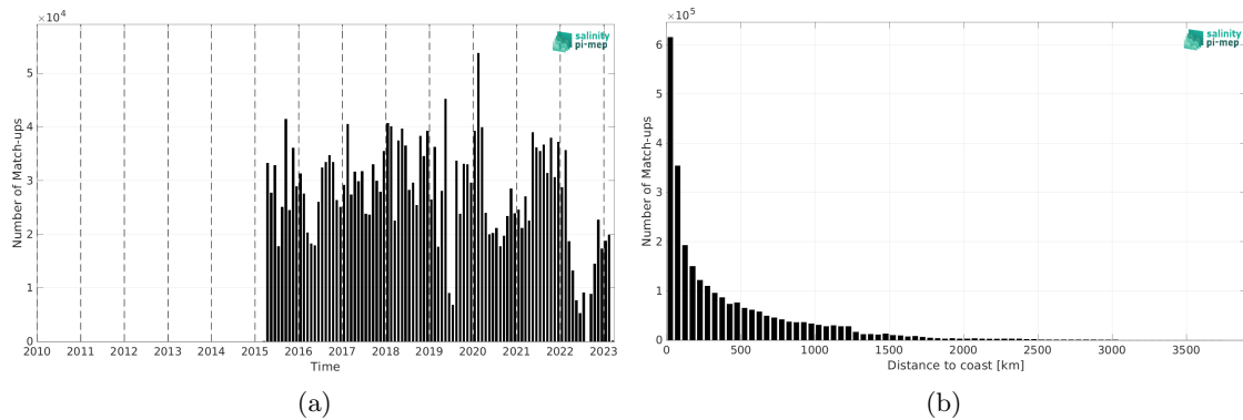
Figure 2: Number of match-ups between TSG (LEGOS-DM) and SMAP SSS L2 v5.0 (JPL) SSS as a function of time (a) and as function of the distance to coast (b) over the Global Ocean Pi-MEP region and for the full satellite product period.
