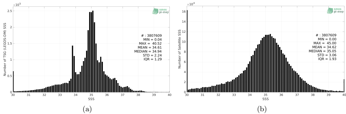
Figure 2: Histograms of SSS from TSG (LEGOS-DM) (a) and SMAP SSS L2 v5.0 (JPL) (b) considering all match-up pairs per bins of 0.1 over the Global Ocean Pi-MEP region and for the full satellite product period.
