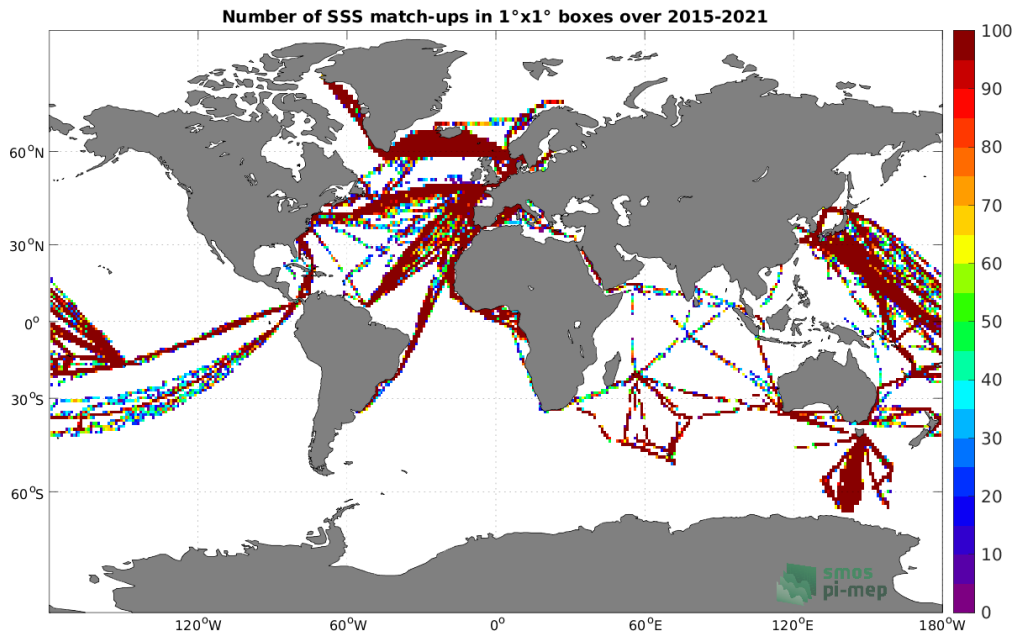
Figure 4: Number of SSS match-ups between TSG (LEGOS-DM) SSS and the SMAP SSS L2 v5.0 (JPL) SSS product for the Global Ocean Pi-MEP region over 1^\circ \times 1^\circ boxes and for the full satellite product period.
