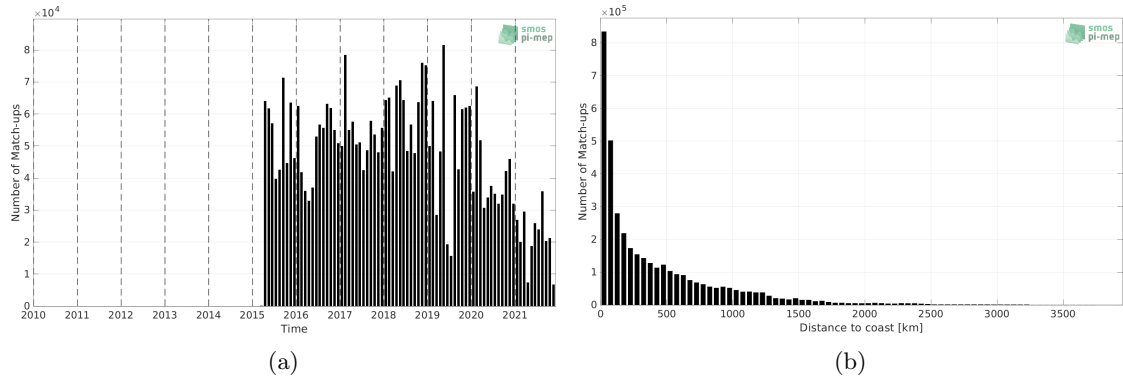
Figure 1: Number of match-ups between TSG (LEGOS-DM) and SMAP SSS L2 v5.0 (JPL) SSS as a function of time (a) and as function of the distance to coast (b) over the Global Ocean Pi-MEP region and for the full satellite product period.
