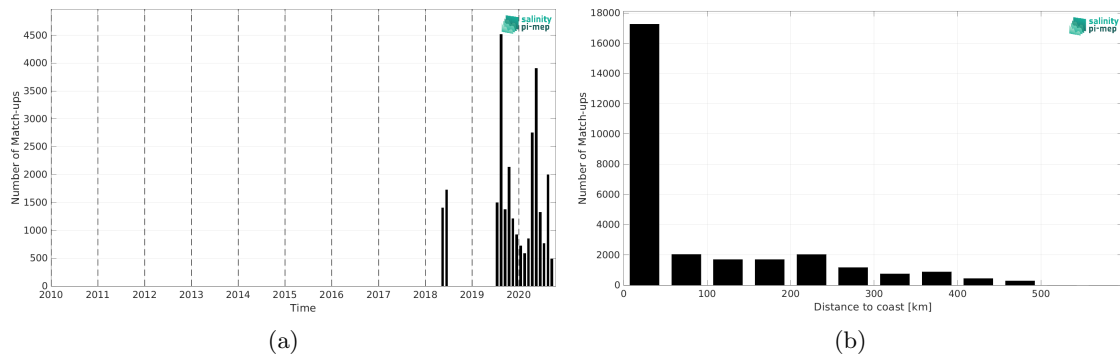
Figure 2: Number of match-ups between TSG (Lauge-Koch) and SMAP SSS L2 v5.0 (JPL) SSS as a function of time (a) and as function of the distance to coast (b) over the Global Ocean Pi-MEP region and for the full satellite product period.
