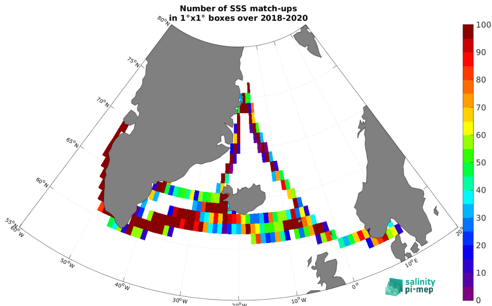
Figure 5: Number of SSS match-ups between TSG (Lauge-Koch) SSS and the SMAP SSS L2 v5.0 (JPL) SSS product for the Global Ocean Pi-MEP region over 1°x1° boxes and for the full satellite product period.
