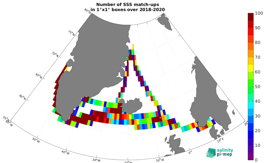
Figure 4: Number of SSS match-ups between TSG (Lauge-Koch) SSS and the SMAP SSS L2 v5.0 (JPL) SSS product for the Global Ocean Pi-MEP region over 1^\circ \times 1^\circ boxes and for the full satellite product period.
