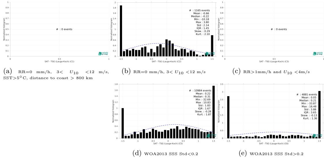
Figure 13: Normalized histogram of \Delta SSS (SMAP SSS L2 v5.0 (JPL) - TSG (Lauge-Koch)) for 5 different subdatasets corresponding to: RR=0 mm/h, 3 < U_{10} < 12 m/s, SST > 5°C, distance to coast > 800 km (a), RR=0 mm/h, 3 < U_{10} < 12 m/s (b), RR > 1mm/h and U_{10} < 4 m/s (c), WOA2013 SSS Std < 0.2 (d), WOA2013 SSS Std > 0.2 (e).
