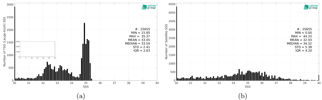
Figure 2: Histograms of SSS from TSG (Lauge-Koch) (a) and SMAP SSS L2 v5.0 (JPL) (b) considering all match-up pairs per bins of 0.1 over the Global Ocean Pi-MEP region and for the full satellite product period.
