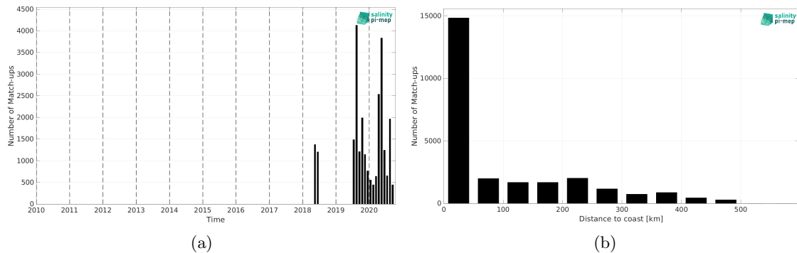
Figure 1: Number of match-ups between TSG (Lauge-Koch) and SMAP SSS L2 v5.0 (JPL) SSS as a function of time (a) and as function of the distance to coast (b) over the Global Ocean Pi-MEP region and for the full satellite product period.
