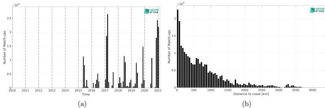
Figure 2: Number of match-ups between TSG (GOSUD-Sailing-ship) and SMAP SSS L2 v5.0 (JPL) SSS as a function of time (a) and as function of the distance to coast (b) over the Global Ocean Pi-MEP region and for the full satellite product period.
