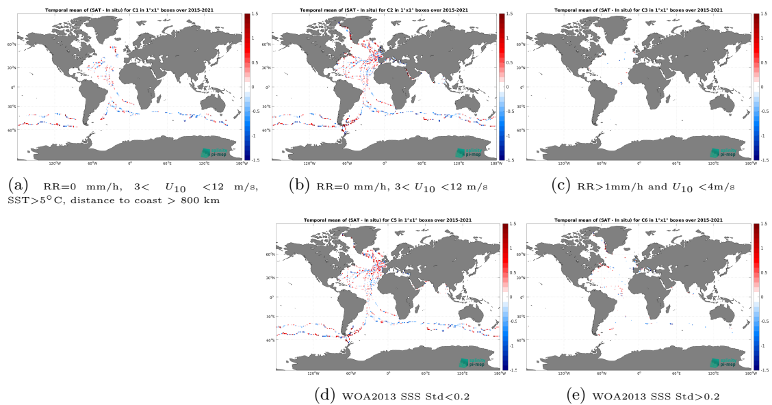
Figure 14: Temporal mean gridded over spatial boxes of size 1^\circ \times 1^\circ of \Delta SSS (SMAP SSS L2 v5.0 (JPL) - TSG (GOSUD-Sailing-ship)) for 5 different subdatasets corresponding to:RR=0 mm/h, 3 < U_{10} < 12 m/s, SST > 5^\circ\text{C} , distance to coast > 800 km (a), RR=0 mm/h, 3 < U_{10} < 12 m/s (b), RR > 1 mm/h and U_{10} < 4 m/s (c), WOA2013 SSS Std < 0.2 (d), WOA2013 SSS Std > 0.2 (e).
