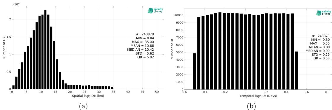
Figure 6: Histograms of the spatial (a) and temporal (b) lags between the location/time of the TSG (GOSUD-Sailing-ship) measurement and the date of the corresponding SMAP SSS L2 v5.0 (JPL) SSS pixel.
