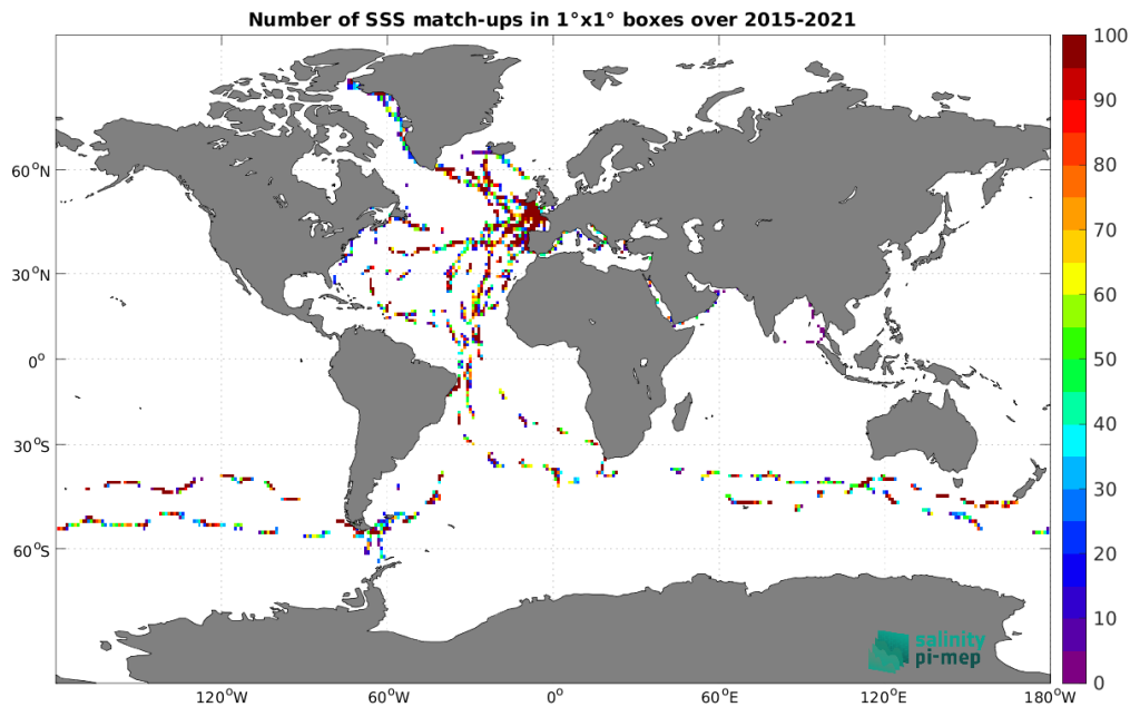
Figure 5: Number of SSS match-ups between TSG (GOSUD-Sailing-ship) SSS and the SMAP SSS L2 v5.0 (JPL) SSS product for the Global Ocean Pi-MEP region over 1^\circ \times 1^\circ boxes and for the full satellite product period.
