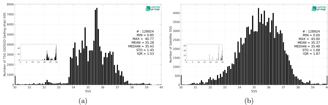
Figure 3: Histograms of SSS from TSG (GOSUD-Sailing-ship) (a) and SMAP SSS L2 v5.0 (JPL) (b) considering all match-up pairs per bins of 0.1 over the Global Ocean Pi-MEP region and for the full satellite product period.
