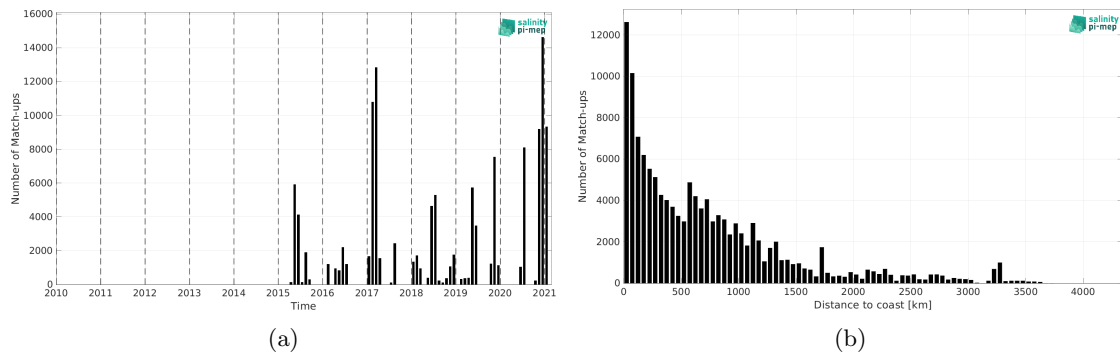
Figure 2: Number of match-ups between TSG (GOSUD-Sailing-ship) and SMAP SSS L2 v5.0 (JPL) SSS as a function of time (a) and as function of the distance to coast (b) over the Global Ocean Pi-MEP region and for the full satellite product period.
