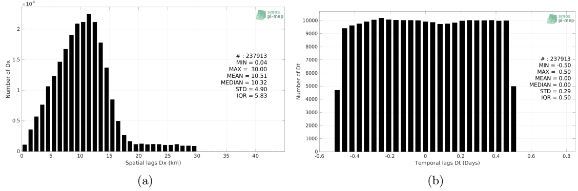
Figure 5: Histograms of the spatial (a) and temporal (b) lags between the location/time of the TSG (GOSUD-Sailing-ship) measurement and the date of the corresponding SMAP SSS L2 v5.0 (JPL) SSS pixel.
