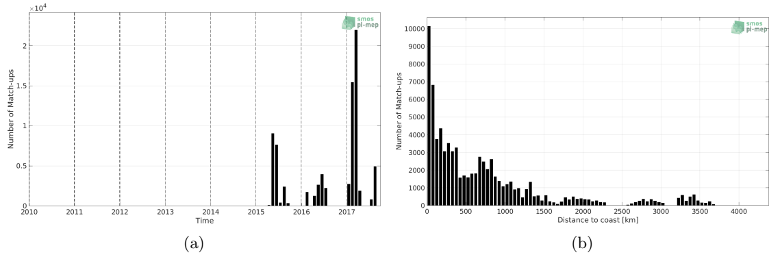
Figure 1: Number of match-ups between TSG (GOSUD-Sailing-ship) and SMAP SSS L2 v5.0 (JPL) SSS as a function of time (a) and as function of the distance to coast (b) over the Global Ocean Pi-MEP region and for the full satellite product period.
