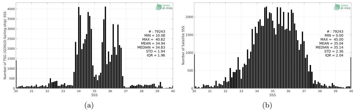
Figure 2: Histograms of SSS from TSG (GOSUD-Sailing-ship) (a) and SMAP SSS L2 v5.0 (JPL) (b) considering all match-up pairs per bins of 0.1 over the Global Ocean Pi-MEP region and for the full satellite product period.
