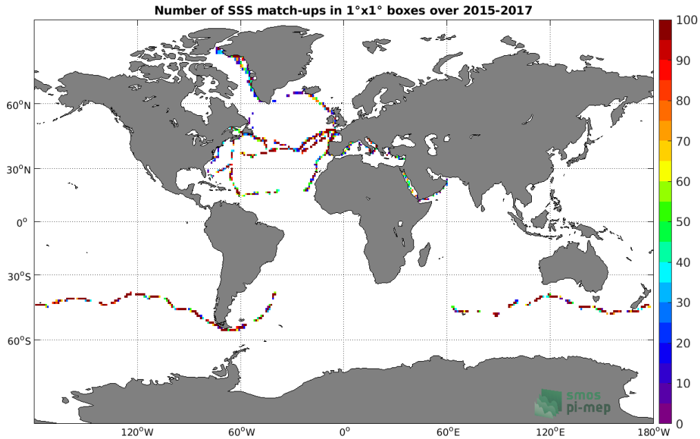
Figure 4: Number of SSS match-ups between TSG (GOSUD-Sailing-ship) SSS and the SMAP SSS L2 v5.0 (JPL) SSS product for the Global Ocean Pi-MEP region over 1^\circ \times 1^\circ boxes and for the full satellite product period.
