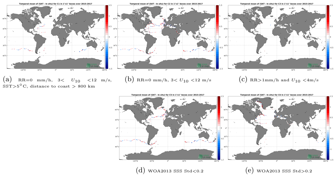
Figure 12: Temporal mean gridded over spatial boxes of size 1^\circ \times 1^\circ of \Delta SSS (SMAP SSS L2 v5.0 (JPL) - TSG (GOSUD-Sailing-ship)) for 5 different subdatasets corresponding to:RR=0 mm/h, 3 < U_{10} < 12 m/s, SST>5°C, distance to coast > 800 km (a), RR=0 mm/h, 3 < U_{10} < 12 m/s (b), RR>1mm/h and U_{10} < 4 m/s (c), WOA2013 SSS Std<0.2 (d), WOA2013 SSS Std>0.2 (e).
