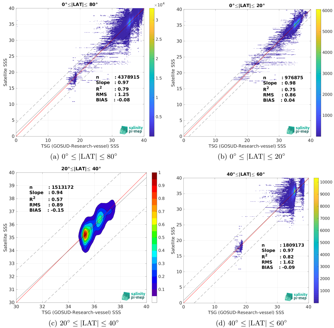
Figure 10: Contour maps of the concentration of SMAP SSS L2 v5.0 (JPL) SSS (y-axis) versus TSG (GOSUD-Research-vessel) SSS (x-axis) at match-up pairs for different latitude bands. For each plot, the red line shows x=y . The black thin and dashed lines indicate a linear fit through the data cloud and the \pm 95\% confidence levels, respectively. The number match-up pairs n , the slope and R^2 coefficient of the linear fit, the root mean square (RMS) and the mean bias between satellite and in situ data are indicated for each latitude band in each plots.
