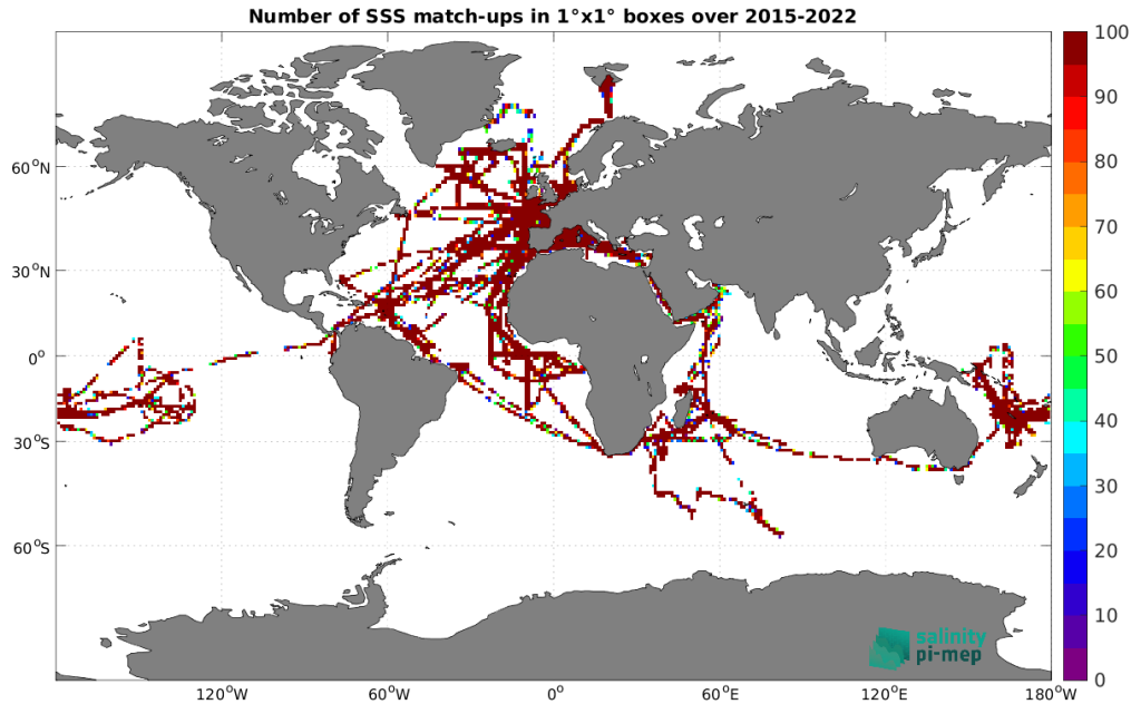
Figure 5: Number of SSS match-ups between TSG (GOSUD-Research-vessel) SSS and the SMAP SSS L2 v5.0 (JPL) SSS product for the Global Ocean Pi-MEP region over 1^\circ \times 1^\circ boxes and for the full satellite product period.
