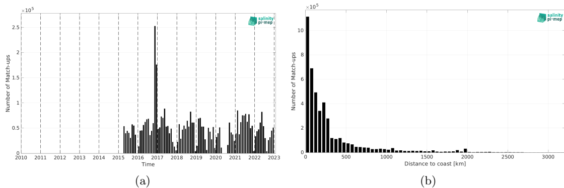
Figure 2: Number of match-ups between TSG (GOSUD-Research-vessel) and SMAP SSS L2 v5.0 (JPL) SSS as a function of time (a) and as function of the distance to coast (b) over the Global Ocean Pi-MEP region and for the full satellite product period.
