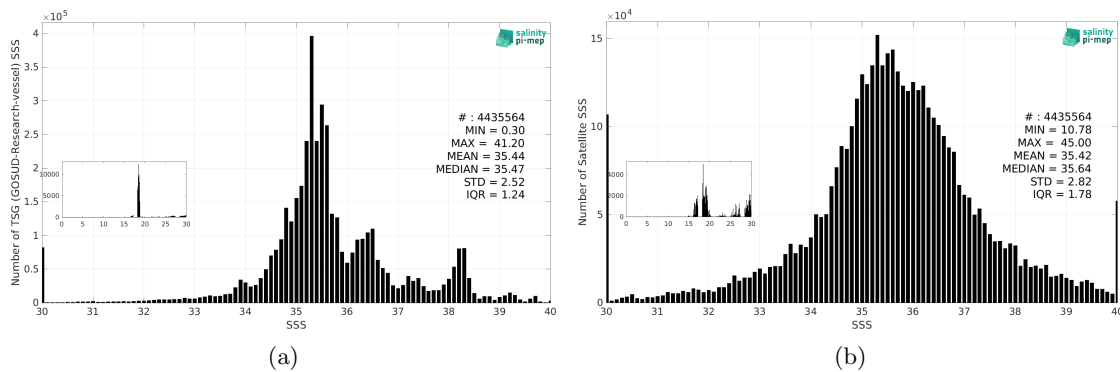
Figure 3: Histograms of SSS from TSG (GOSUD-Research-vessel) (a) and SMAP SSS L2 v5.0 (JPL) (b) considering all match-up pairs per bins of 0.1 over the Global Ocean Pi-MEP region and for the full satellite product period.
