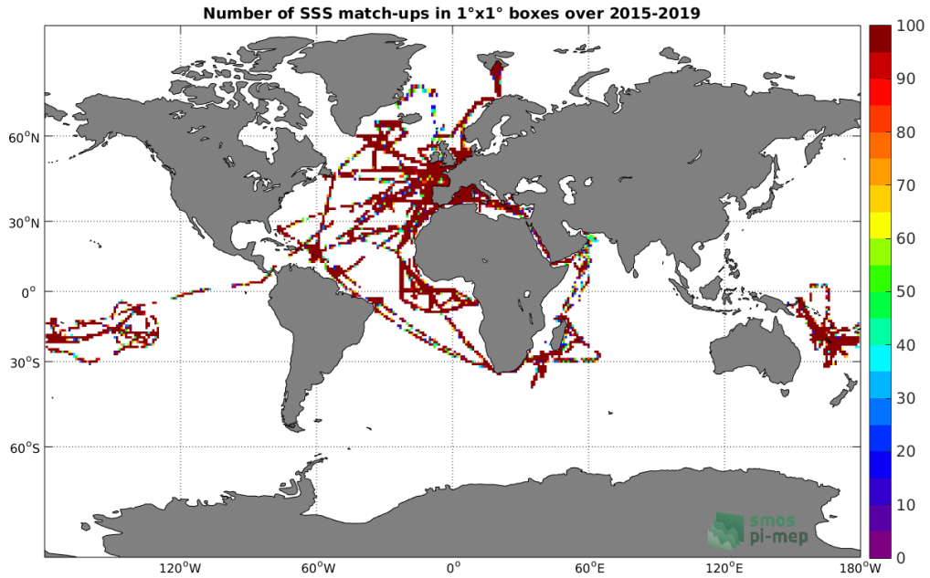
Figure 4: Number of SSS match-ups between TSG (GOSUD-Research-vessel) SSS and the SMAP SSS L2 v5.0 (JPL) SSS product for the Global Ocean Pi-MEP region over 1°x1° boxes and for the full satellite product period.
