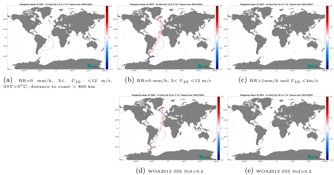
Figure 14: Temporal mean gridded over spatial boxes of size 1^\circ \times 1^\circ of \Delta SSS (SMAP SSS L2 v5.0 (JPL) - TSG (CSIC-UTM)) for 5 different subdatasets corresponding to:RR=0 mm/h, 3 < U_{10} < 12 m/s, SST > 5^\circ\text{C} , distance to coast > 800 km (a), RR=0 mm/h, 3 < U_{10} < 12 m/s (b), RR > 1 mm/h and U_{10} < 4 m/s (c), WOA2013 SSS Std < 0.2 (d), WOA2013 SSS Std > 0.2 (e).
