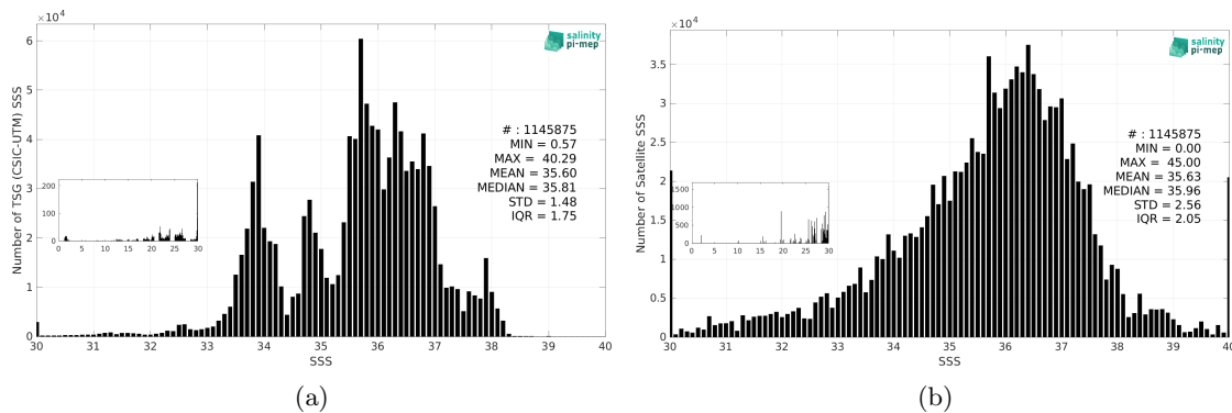
Figure 3: Histograms of SSS from TSG (CSIC-UTM) (a) and SMAP SSS L2 v5.0 (JPL) (b) considering all match-up pairs per bins of 0.1 over the Global Ocean Pi-MEP region and for the full satellite product period.
