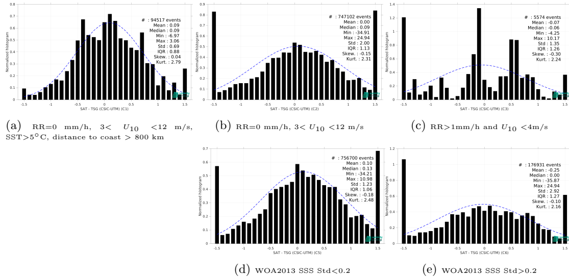
Figure 15: Normalized histogram of \Delta\text{SSS} (SMAP SSS L2 v5.0 (JPL) - TSG (CSIC-UTM)) for 5 different subdatasets corresponding to: RR=0 mm/h, 3 < U_{10} < 12 m/s, SST>5°C, distance to coast > 800 km (a), RR=0 mm/h, 3 < U_{10} < 12 m/s (b), RR>1mm/h and U_{10} < 4 m/s (c), WOA2013 SSS Std<0.2 (d), WOA2013 SSS Std>0.2 (e).
