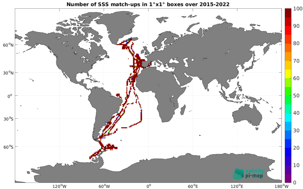
Figure 5: Number of SSS match-ups between TSG (CSIC-UTM) SSS and the SMAP SSS L2 v5.0 (JPL) SSS product for the Global Ocean Pi-MEP region over 1^\circ \times 1^\circ boxes and for the full satellite product period.
