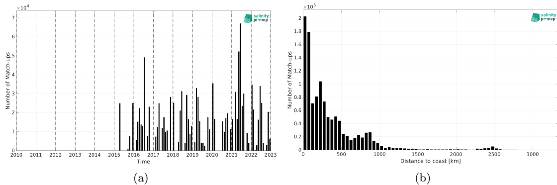
Figure 2: Number of match-ups between TSG (CSIC-UTM) and SMAP SSS L2 v5.0 (JPL) SSS as a function of time (a) and as function of the distance to coast (b) over the Global Ocean Pi-MEP region and for the full satellite product period.
