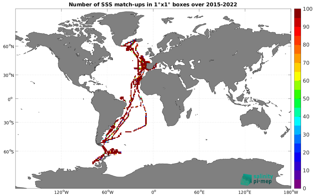
Figure 4: Number of SSS match-ups between TSG (CSIC-UTM) SSS and the SMAP SSS L2 v5.0 (JPL) SSS product for the Global Ocean Pi-MEP region over 1°x1° boxes and for the full satellite product period.
