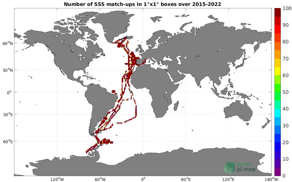
Figure 4: Number of SSS match-ups between TSG (CSIC-UTM) SSS and the SMAP SSS L2 v5.0 (JPL) SSS product for the Global Ocean Pi-MEP region over 1^\circ \times 1^\circ boxes and for the full satellite product period.
