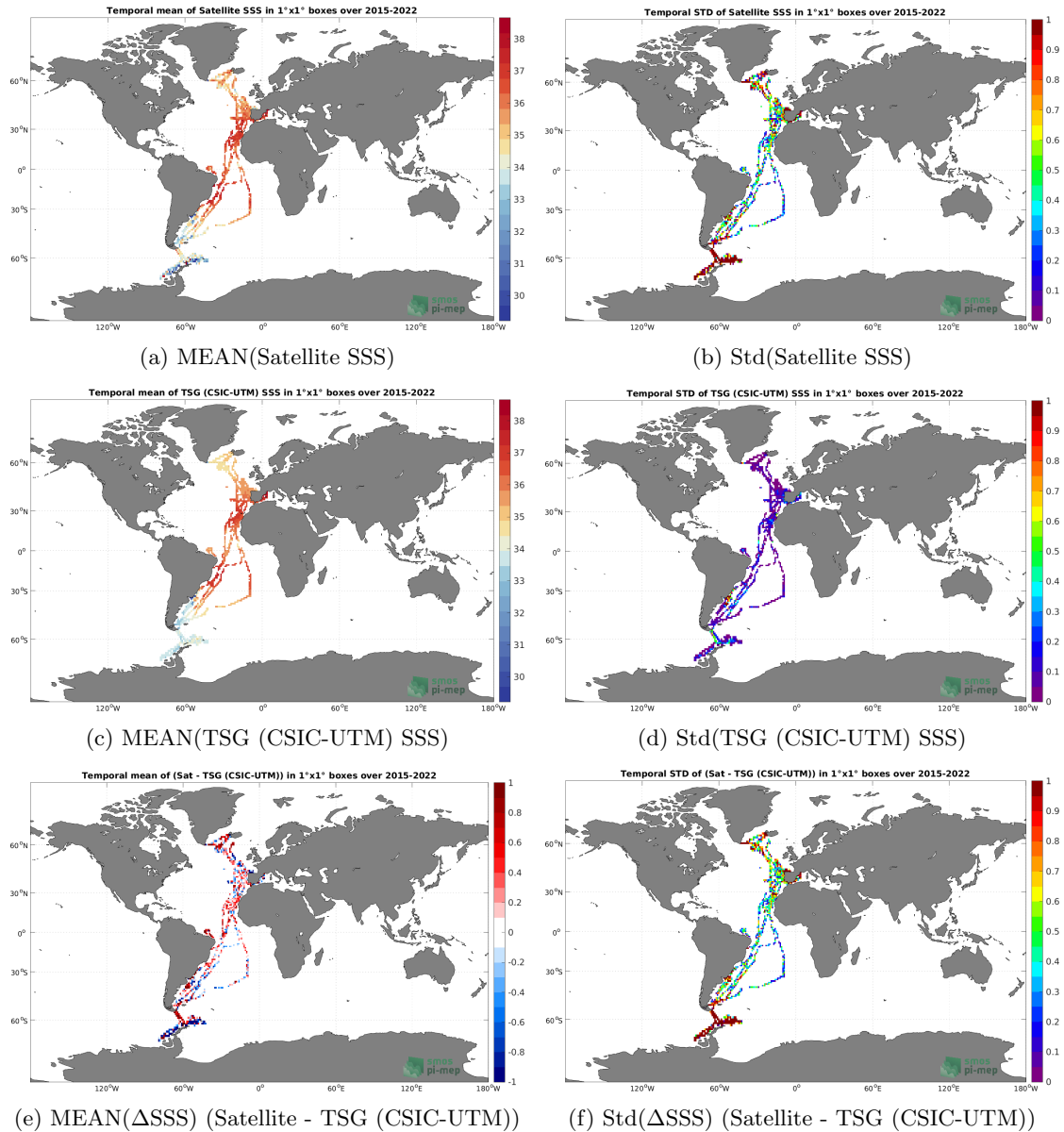
Figure 6: Temporal mean (left) and Std (right) of SSS from SMAP SSS L2 v5.0 (JPL) (top), TSG (CSIC-UTM) (middle), and of \Delta SSS (Satellite - TSG (CSIC-UTM)). Only match-up pairs are used to generate these maps.
