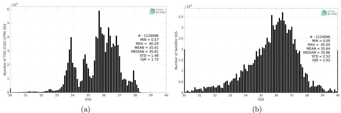
Figure 2: Histograms of SSS from TSG (CSIC-UTM) (a) and SMAP SSS L2 v5.0 (JPL) (b) considering all match-up pairs per bins of 0.1 over the Global Ocean Pi-MEP region and for the full satellite product period.
