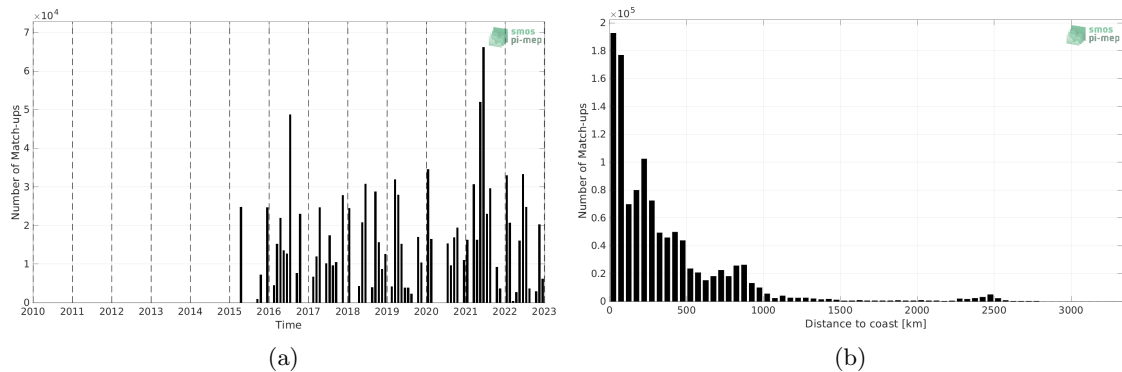
Figure 1: Number of match-ups between TSG (CSIC-UTM) and SMAP SSS L2 v5.0 (JPL) SSS as a function of time (a) and as function of the distance to coast (b) over the Global Ocean Pi-MEP region and for the full satellite product period.
