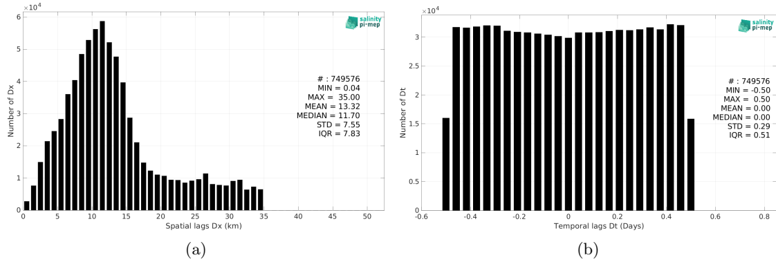
Figure 6: Histograms of the spatial (a) and temporal (b) lags between the location/time of the TSG (Amundsen) measurement and the date of the corresponding SMAP SSS L2 v5.0 (JPL) SSS pixel.
