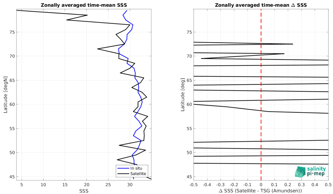
Figure 9: Left panel: Zonal mean SSS from SMAP SSS L2 v5.0 (JPL) satellite product (black) and from TSG (Amundsen) (blue). Right panel: Zonal mean of \Delta SSS (Satellite - TSG (Amundsen)) for all the collected Pi-MEP match-up pairs estimated over the full satellite product period.
