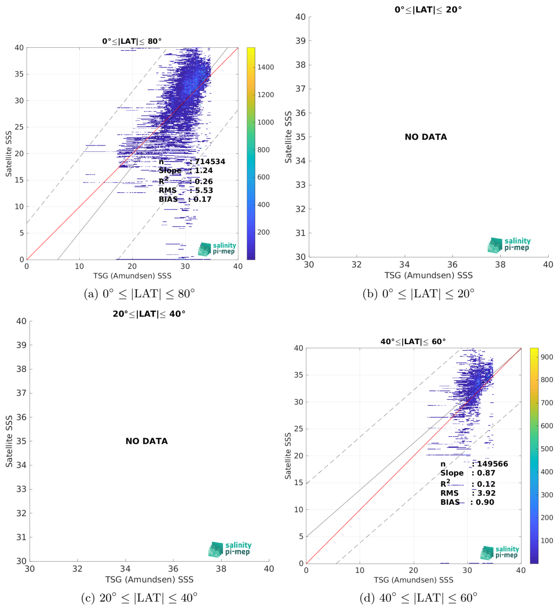
Figure 10: Contour maps of the concentration of SMAP SSS L2 v5.0 (JPL) SSS (y-axis) versus TSG (Amundsen) SSS (x-axis) at match-up pairs for different latitude bands. For each plot, the red line shows x=y . The black thin and dashed lines indicate a linear fit through the data cloud and the \pm 95\% confidence levels, respectively. The number match-up pairs n , the slope and R^2 coefficient of the linear fit, the root mean square (RMS) and the mean bias between satellite and in situ data are indicated for each latitude band in each plots.
