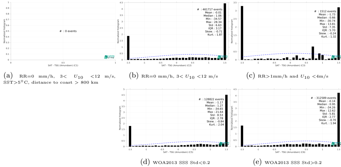
Figure 15: Normalized histogram of \Delta SSS (SMAP SSS L2 v5.0 (JPL) - TSG (Amundsen)) for 5 different subdatasets corresponding to: RR=0 mm/h, 3 < U_{10} < 12 m/s, SST > 5°C, distance to coast > 800 km (a), RR=0 mm/h, 3 < U_{10} < 12 m/s (b), RR > 1mm/h and U_{10} < 4 m/s (c), WOA2013 SSS Std < 0.2 (d), WOA2013 SSS Std > 0.2 (e).
