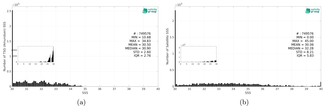
Figure 3: Histograms of SSS from TSG (Amundsen) (a) and SMAP SSS L2 v5.0 (JPL) (b) considering all match-up pairs per bins of 0.1 over the Global Ocean Pi-MEP region and for the full satellite product period.
