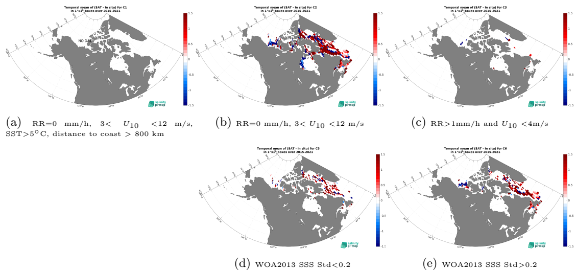
Figure 14: Temporal mean gridded over spatial boxes of size 1^\circ \times 1^\circ of \Delta SSS (SMAP SSS L2 v5.0 (JPL) - TSG (Amundsen)) for 5 different subdatasets corresponding to:RR=0 mm/h, 3 < U_{10} < 12 m/s, SST > 5°C, distance to coast > 800 km (a), RR=0 mm/h, 3 < U_{10} < 12 m/s (b), RR > 1mm/h and U_{10} < 4 m/s (c), WOA2013 SSS Std < 0.2 (d), WOA2013 SSS Std > 0.2 (e).
