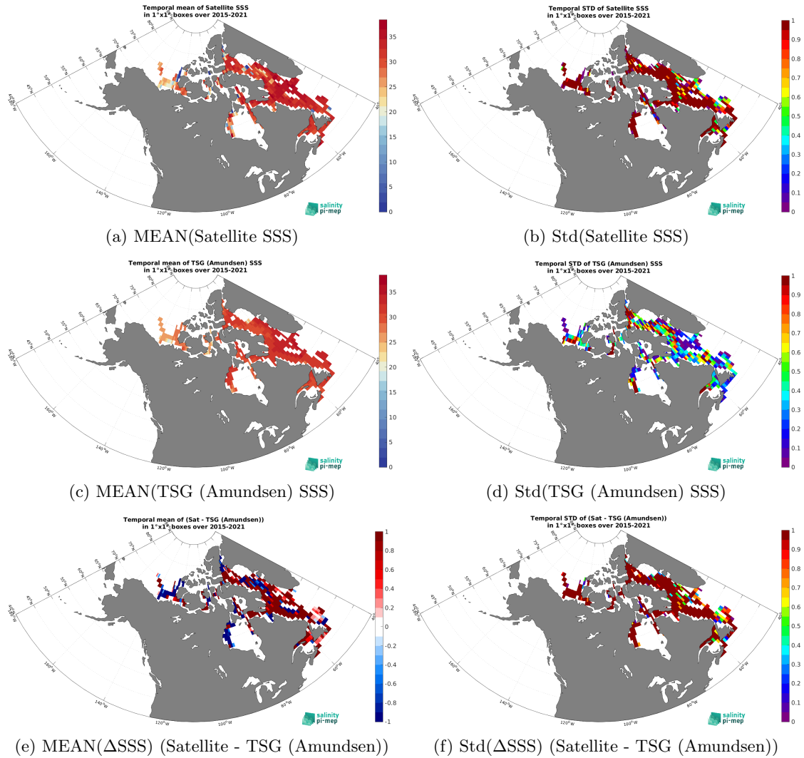
Figure 7: Temporal mean (left) and Std (right) of SSS from SMAP SSS L2 v5.0 (JPL) (top), TSG (Amundsen) (middle), and of \Delta SSS (Satellite - TSG (Amundsen)). Only match-up pairs are used to generate these maps.
