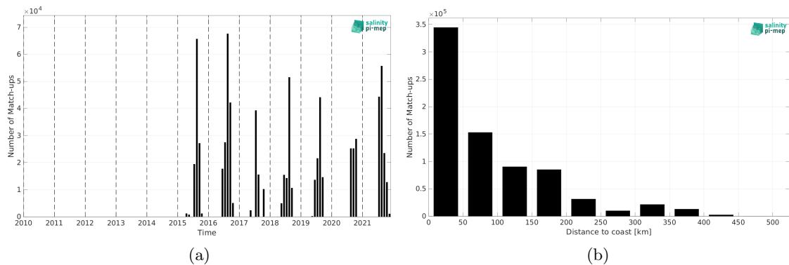
Figure 2: Number of match-ups between TSG (Amundsen) and SMAP SSS L2 v5.0 (JPL) SSS as a function of time (a) and as function of the distance to coast (b) over the Global Ocean Pi-MEP region and for the full satellite product period.
