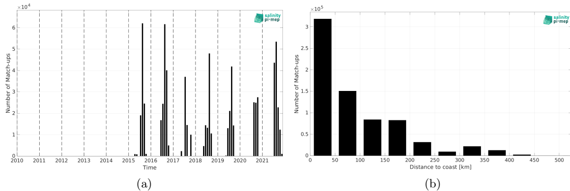
Figure 1: Number of match-ups between TSG (Amundsen) and SMAP SSS L2 v5.0 (JPL) SSS as a function of time (a) and as function of the distance to coast (b) over the Global Ocean Pi-MEP region and for the full satellite product period.
