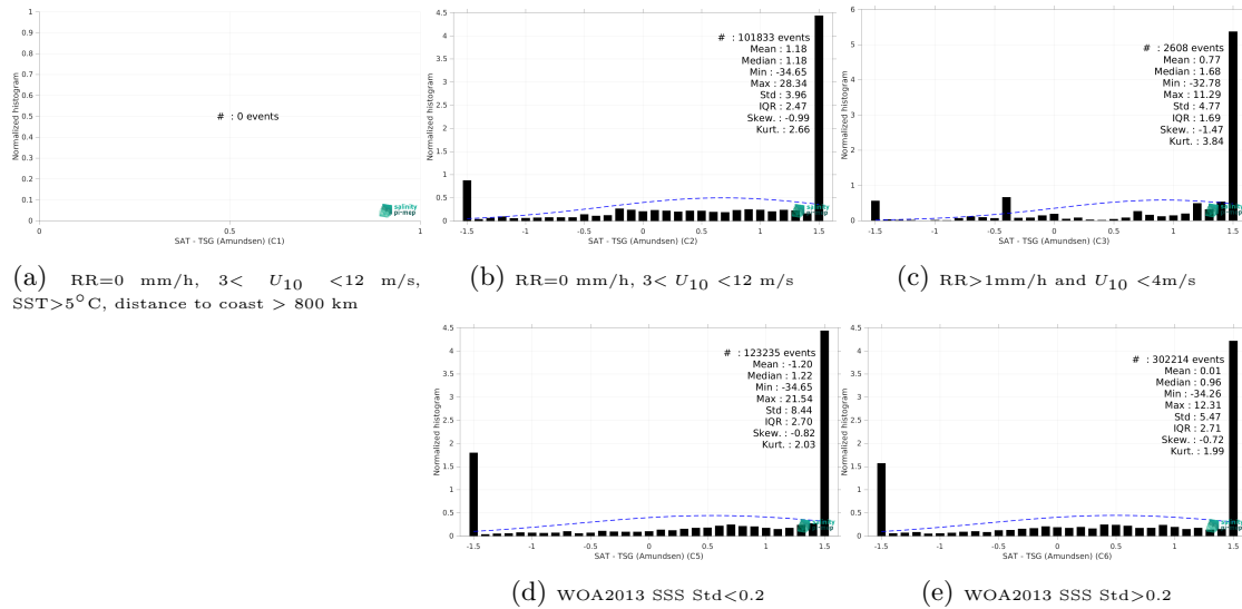
Figure 13: Normalized histogram of \Delta SSS (SMAP SSS L2 v5.0 (JPL) - TSG (Amundsen)) for 5 different subdatasets corresponding to: RR=0 mm/h, 3 < U_{10} < 12 m/s, SST > 5°C, distance to coast > 800 km (a), RR=0 mm/h, 3 < U_{10} < 12 m/s (b), RR > 1mm/h and U_{10} < 4 m/s (c), WOA2013 SSS Std < 0.2 (d), WOA2013 SSS Std > 0.2 (e).
