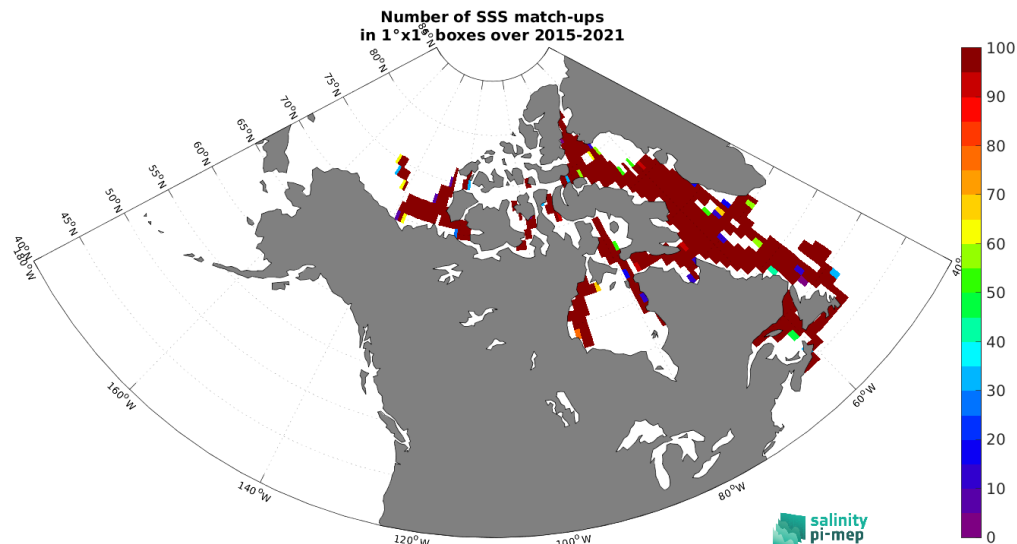
Figure 4: Number of SSS match-ups between TSG (Amundsen) SSS and the SMAP SSS L2 v5.0 (JPL) SSS product for the Global Ocean Pi-MEP region over 1^\circ \times 1^\circ boxes and for the full satellite product period.
