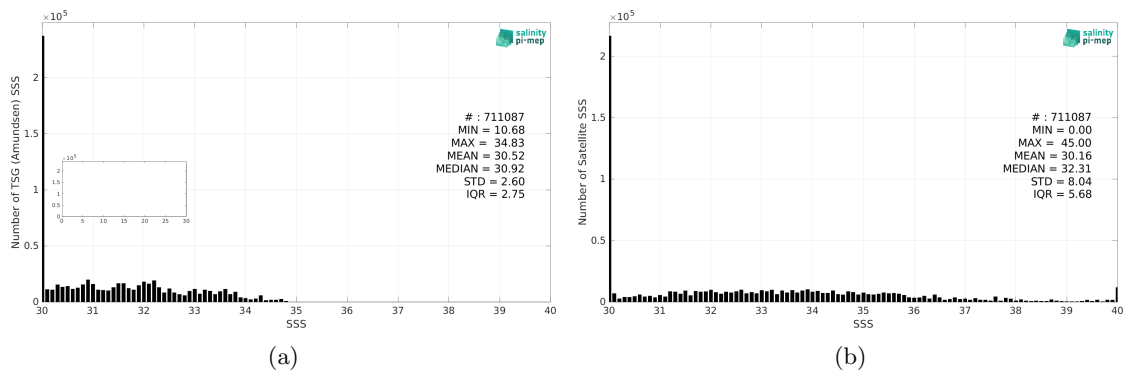
Figure 2: Histograms of SSS from TSG (Amundsen) (a) and SMAP SSS L2 v5.0 (JPL) (b) considering all match-up pairs per bins of 0.1 over the Global Ocean Pi-MEP region and for the full satellite product period.
