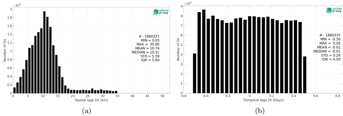
Figure 6: Histograms of the spatial (a) and temporal (b) lags between the location/time of the SASSIE measurement and the date of the corresponding SMAP SSS L2 v5.0 (JPL) SSS pixel.
