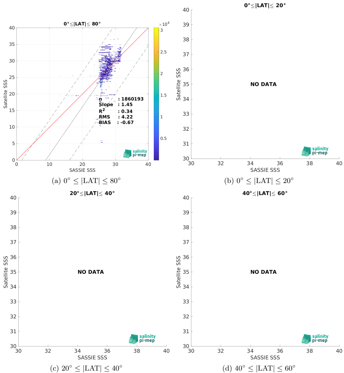
Figure 10: Contour maps of the concentration of SMAP SSS L2 v5.0 (JPL) SSS (y-axis) versus SASSIE SSS (x-axis) at match-up pairs for different latitude bands. For each plot, the red line shows x=y . The black thin and dashed lines indicate a linear fit through the data cloud and the \pm 95\% confidence levels, respectively. The number match-up pairs n , the slope and R^2 coefficient of the linear fit, the root mean square (RMS) and the mean bias between satellite and in situ data are indicated for each latitude band in each plots.
