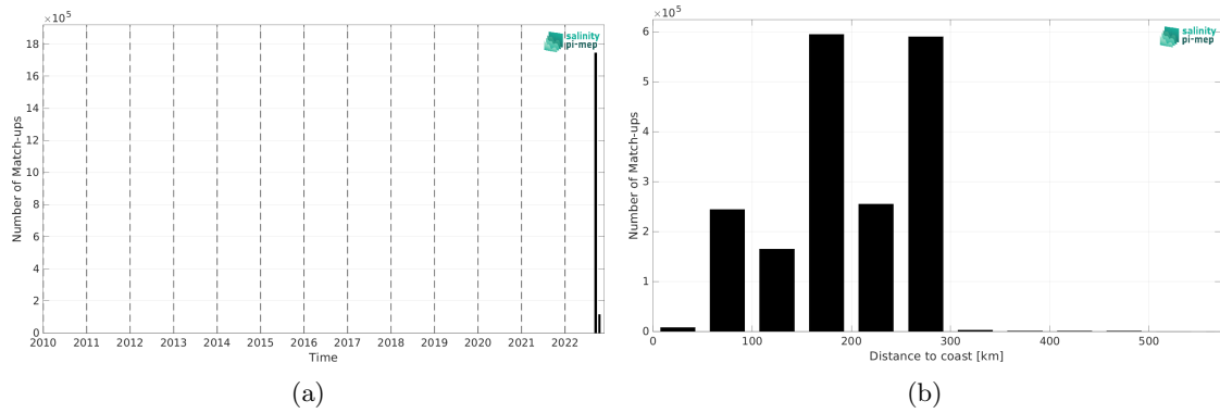
Figure 2: Number of match-ups between SASSIE and SMAP SSS L2 v5.0 (JPL) SSS as a function of time (a) and as function of the distance to coast (b) over the Global Ocean Pi-MEP region and for the full satellite product period.
