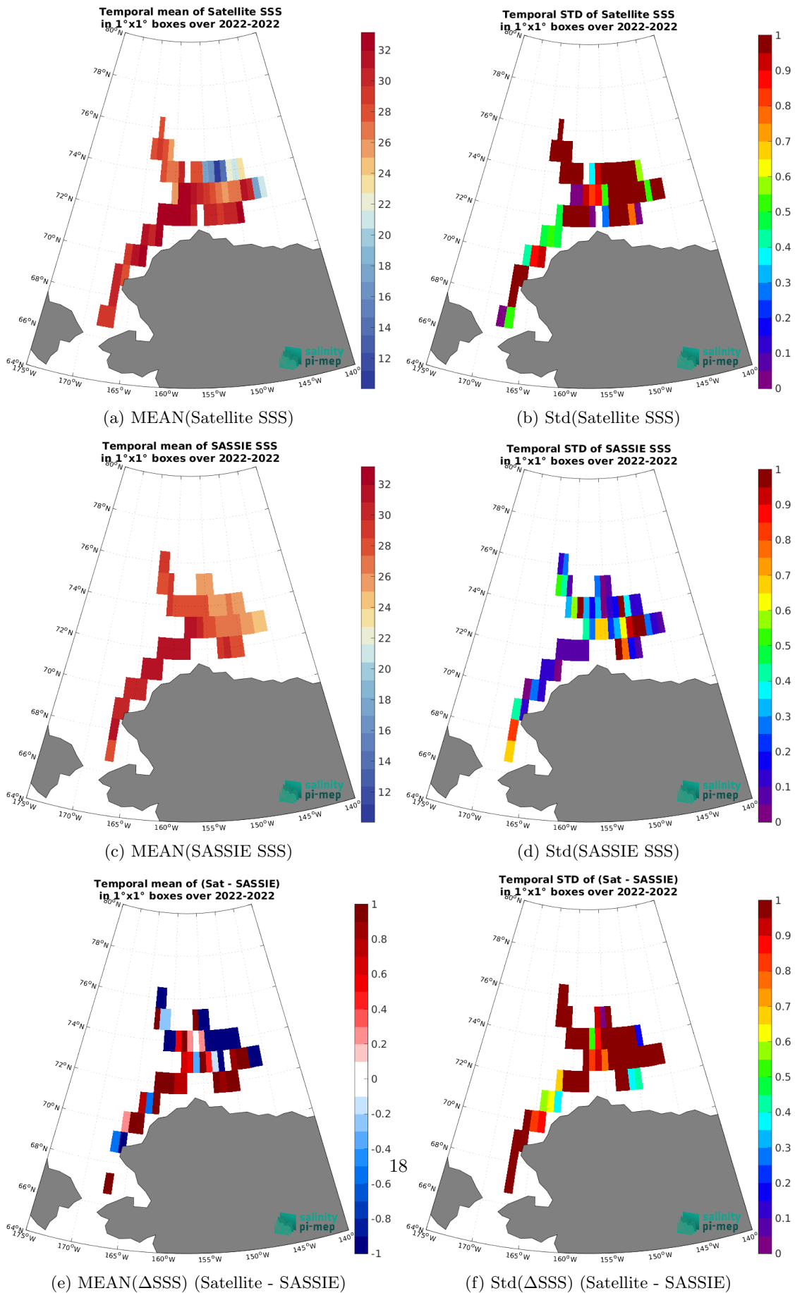
(a) MEAN(Satellite SSS) (b) Std(Satellite SSS) (c) MEAN(SASSIE SSS) (d) Std(SASSIE SSS) (e) MEAN( \Delta SSS) (Satellite - SASSIE) (f) Std( \Delta SSS) (Satellite - SASSIE) Figure 7: Temporal mean (left) and Std (right) of SSS from SMAP SSS L2 v5.0 (JPL) (top), SASSIE (middle), and of \Delta SSS (Satellite - SASSIE). Only match-up pairs are used to generate these maps.
