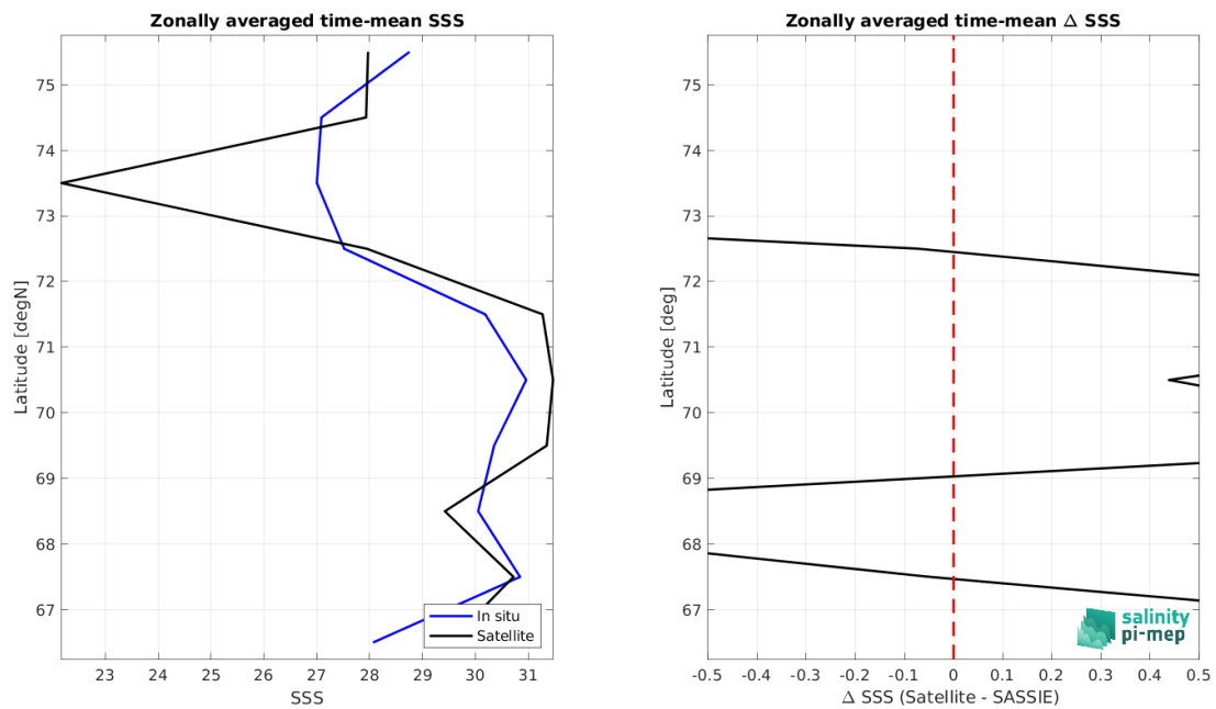
Figure 9: Left panel: Zonal mean SSS from SMAP SSS L2 v5.0 (JPL) satellite product (black) and from SASSIE (blue). Right panel: Zonal mean of \Delta SSS (Satellite - SASSIE) for all the collected Pi-MEP match-up pairs estimated over the full satellite product period.
