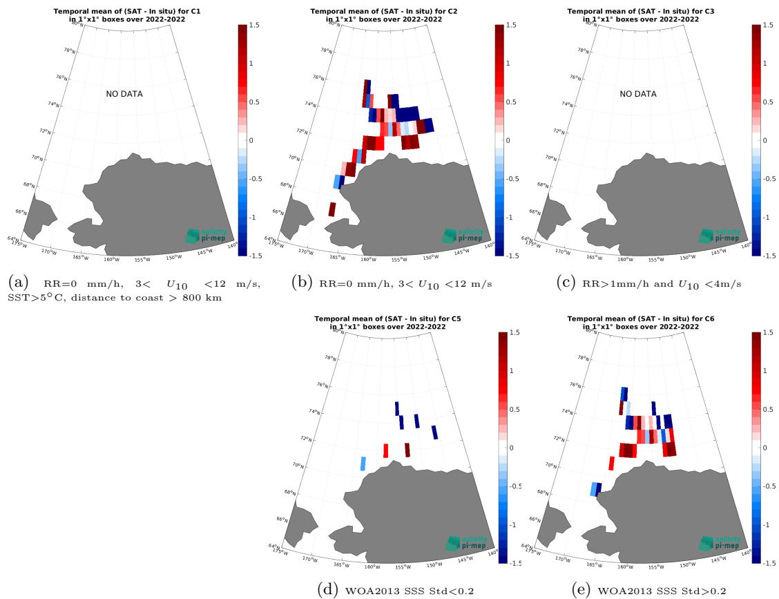
Figure 14: Temporal mean gridded over spatial boxes of size 1^\circ \times 1^\circ of \Delta\text{SSS} (SMAP SSS L2 v5.0 (JPL) - SASSIE) for 5 different subdatasets corresponding to:RR=0 mm/h, 3 < U_{10} < 12 m/s, SST>5°C, distance to coast > 800 km (a), RR=0 mm/h, 3 < U_{10} < 12 m/s (b), RR>1mm/h and U_{10} < 4 m/s (c), WOA2013 SSS Std<0.2 (d), WOA2013 SSS Std>0.2 (e).
