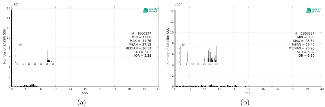
Figure 3: Histograms of SSS from SASSIE (a) and SMAP SSS L2 v5.0 (JPL) (b) considering all match-up pairs per bins of 0.1 over the Global Ocean Pi-MEP region and for the full satellite product period.
