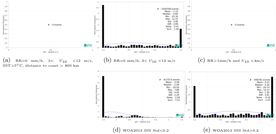
Figure 15: Normalized histogram of \Delta SSS (SMAP SSS L2 v5.0 (JPL) - SASSIE) for 5 different subdatasets corresponding to: RR=0 mm/h, 3 < U_{10} < 12 m/s, SST > 5°C, distance to coast > 800 km (a), RR=0 mm/h, 3 < U_{10} < 12 m/s (b), RR > 1mm/h and U_{10} < 4 m/s (c), WOA2013 SSS Std < 0.2 (d), WOA2013 SSS Std > 0.2 (e).
