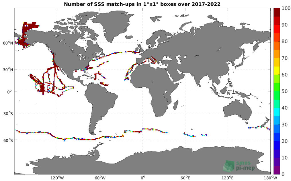
Figure 4: Number of SSS match-ups between SAILDRONE SSS and the SMAP SSS L2 v5.0 (JPL) SSS product for the Global Ocean Pi-MEP region over 1^\circ \times 1^\circ boxes and for the full satellite product period.
