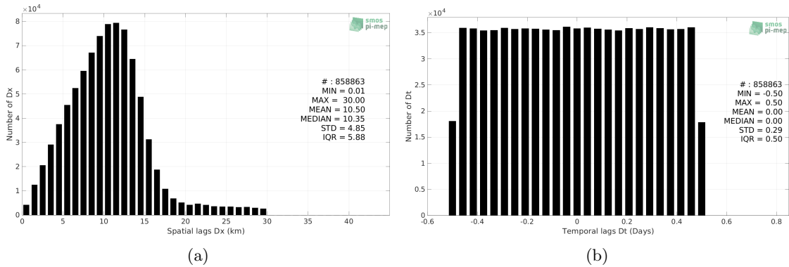
Figure 5: Histograms of the spatial (a) and temporal (b) lags between the location/time of the SAILDRONE measurement and the date of the corresponding SMAP SSS L2 v5.0 (JPL) SSS pixel.
