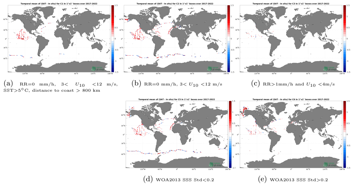
Figure 12: Temporal mean gridded over spatial boxes of size 1^\circ \times 1^\circ of \Delta SSS (SMAP SSS L2 v5.0 (JPL) - Saldrone) for 5 different subdatasets corresponding to:RR=0 mm/h, 3 < U_{10} < 12 m/s, SST > 5^\circ\text{C} , distance to coast > 800 km (a), RR=0 mm/h, 3 < U_{10} < 12 m/s (b), RR > 1 mm/h and U_{10} < 4 m/s (c), WOA2013 SSS Std < 0.2 (d), WOA2013 SSS Std > 0.2 (e).
