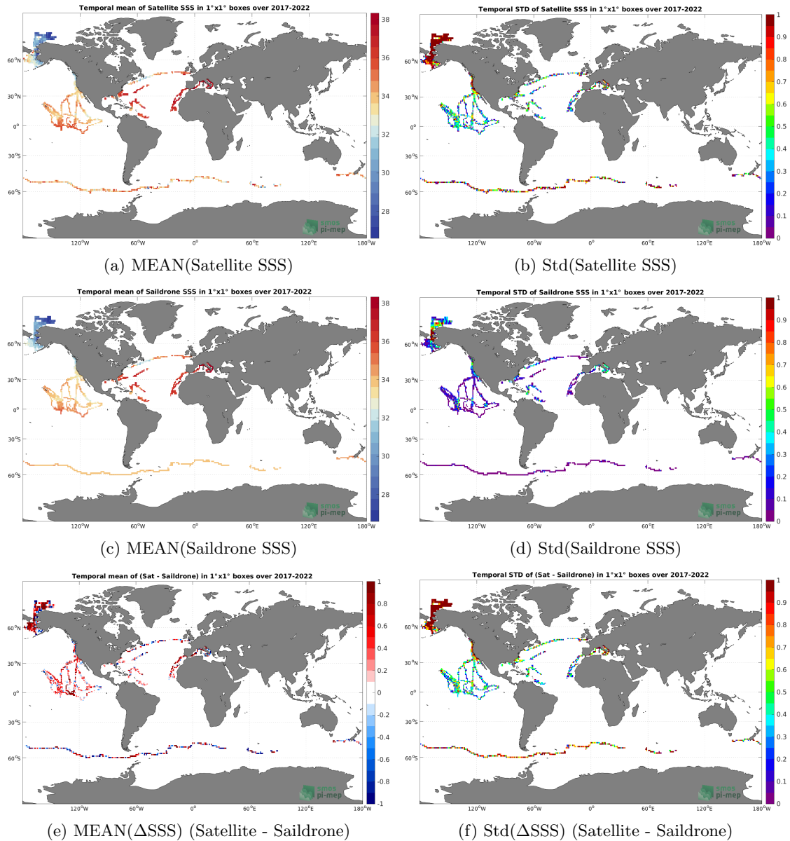
Figure 6: Temporal mean (left) and Std (right) of SSS from SMAP SSS L2 v5.0 (JPL) (top), Saildrone (middle), and of \Delta SSS (Satellite - Saildrone). Only match-up pairs are used to generate these maps.
