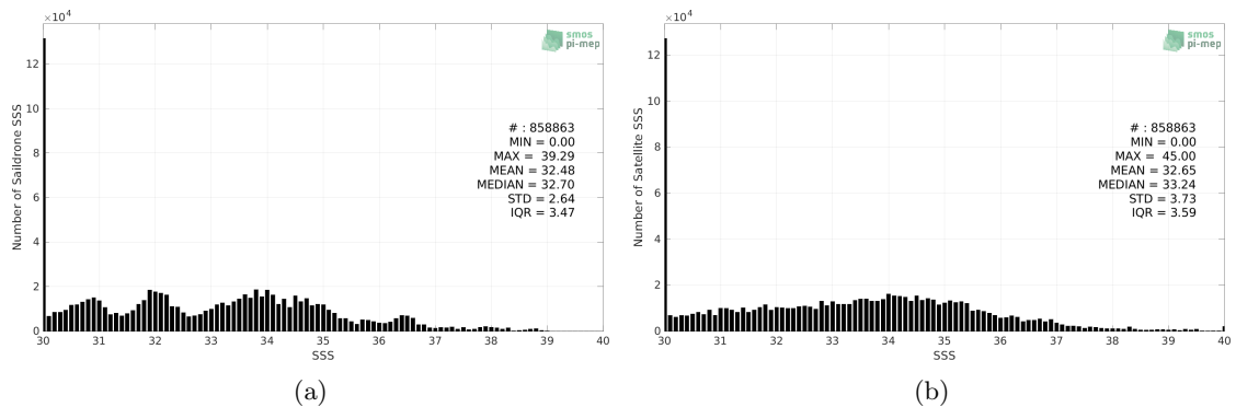
Figure 2: Histograms of SSS from Sairdrone (a) and SMAP SSS L2 v5.0 (JPL) (b) considering all match-up pairs per bins of 0.1 over the Global Ocean Pi-MEP region and for the full satellite product period.
