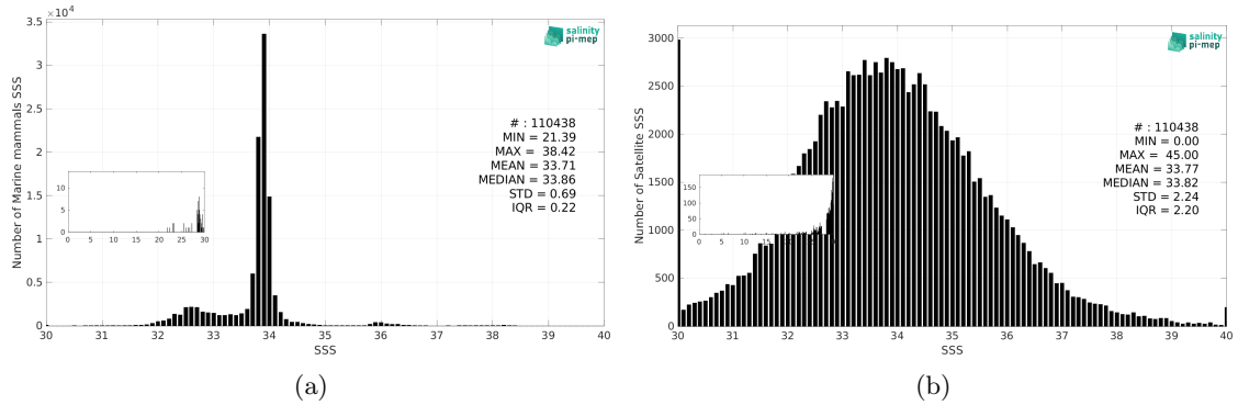
Figure 3: Histograms of SSS from Marine mammals (a) and SMAP SSS L2 v5.0 (JPL) (b) considering all match-up pairs per bins of 0.1 over the Global Ocean Pi-MEP region and for the full satellite product period.
