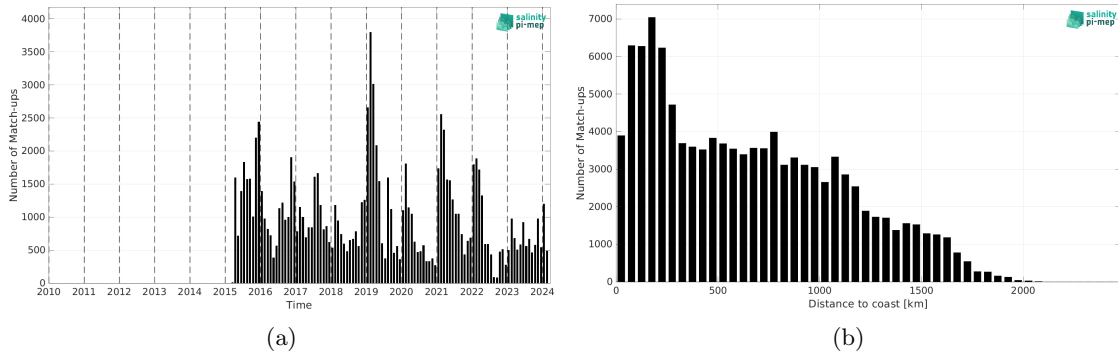
Figure 2: Number of match-ups between Marine mammals and SMAP SSS L2 v5.0 (JPL) SSS as a function of time (a) and as function of the distance to coast (b) over the Global Ocean Pi-MEP region and for the full satellite product period.
