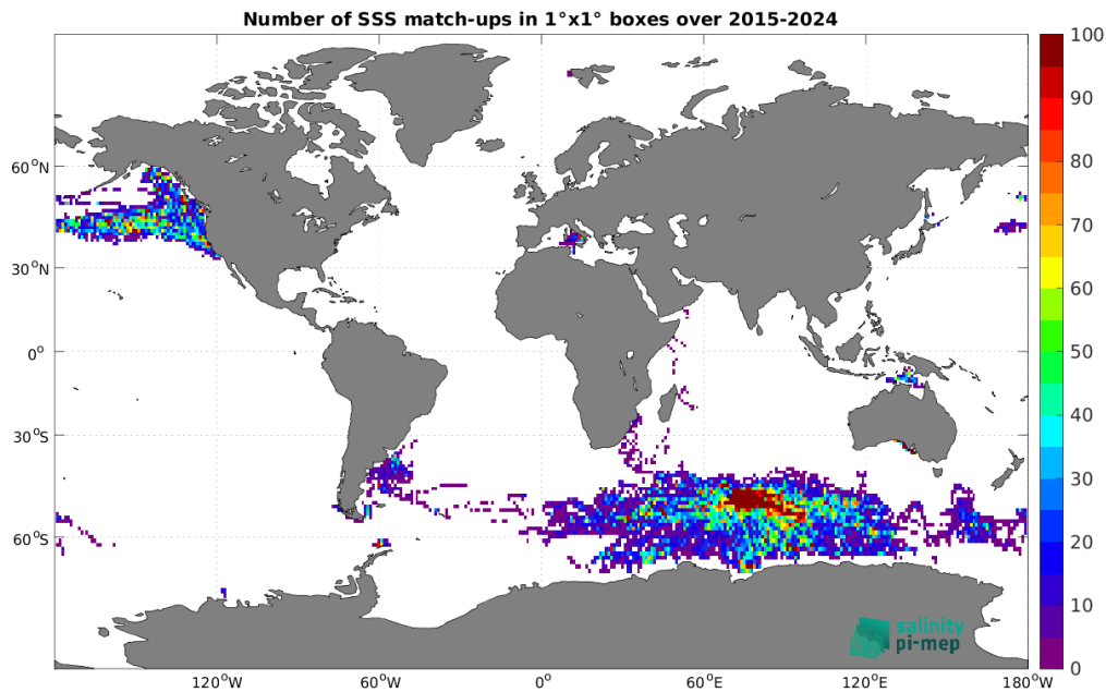
Figure 5: Number of SSS match-ups between Marine mammals SSS and the SMAP SSS L2 v5.0 (JPL) SSS product for the Global Ocean Pi-MEP region over 1°x1° boxes and for the full satellite product period.
