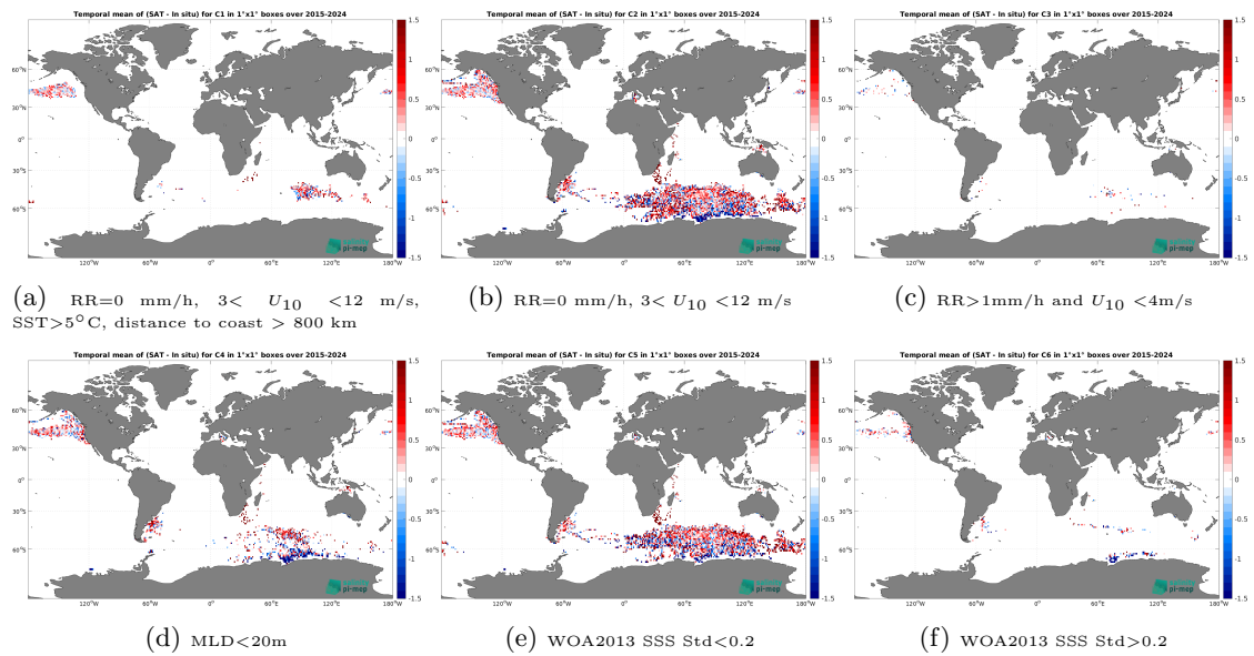
Figure 14: Temporal mean gridded over spatial boxes of size 1^\circ \times 1^\circ of \Delta SSS (SMAP SSS L2 v5.0 (JPL) - Marine mammals) for 6 different subdatasets corresponding to:RR=0 mm/h, 3 < U_{10} < 12 m/s, SST>5°C, distance to coast > 800 km (a), RR=0 mm/h, 3 < U_{10} < 12 m/s (b), RR>1mm/h and U_{10} < 4 m/s (c),MLD<20m (d),WOA2013 SSS Std<0.2 (e),WOA2013 SSS Std>0.2 (f).
