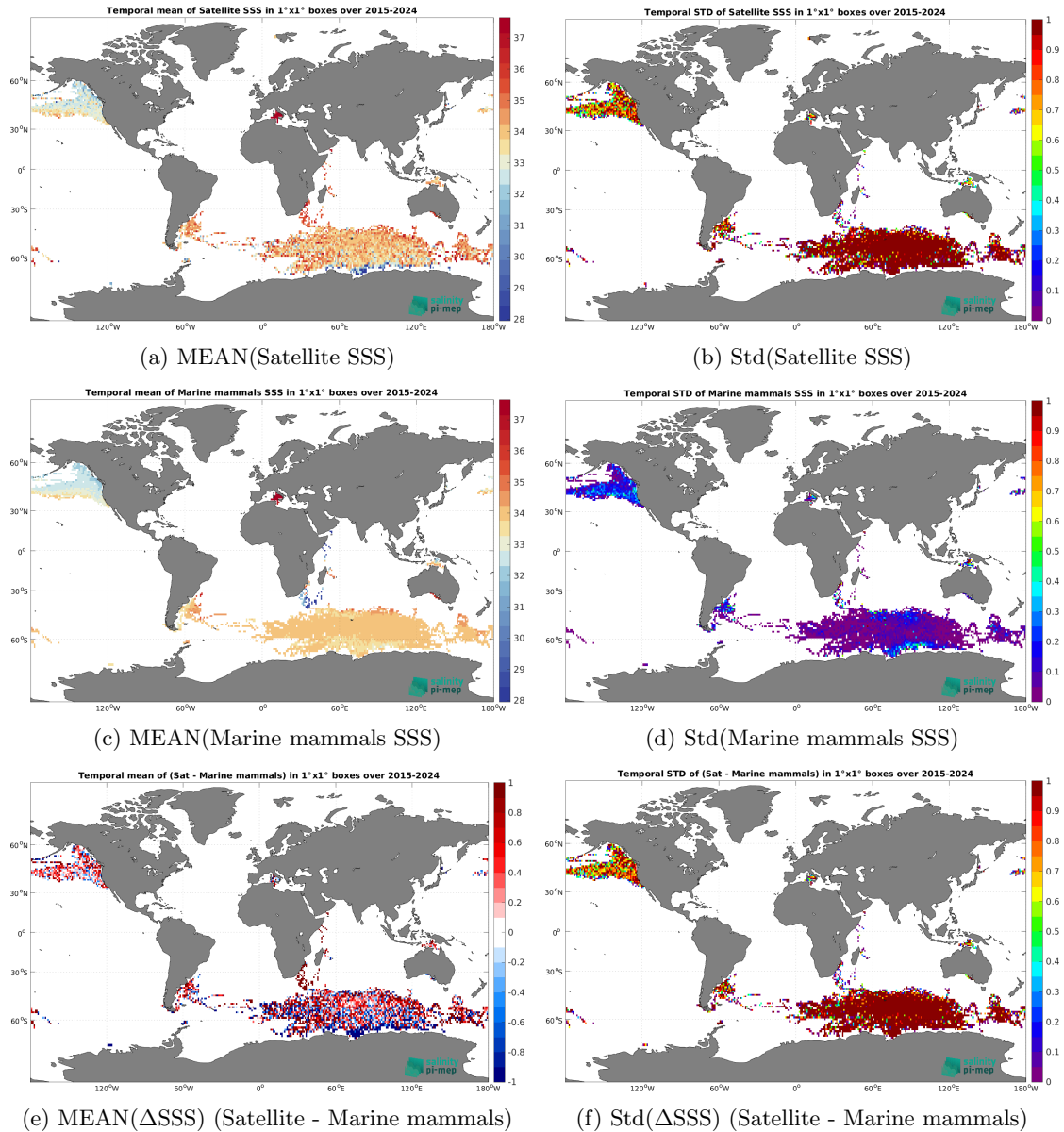
Figure 7: Temporal mean (left) and Std (right) of SSS from SMAP SSS L2 v5.0 (JPL) (top), Marine mammals (middle), and of \Delta SSS (Satellite - Marine mammals). Only match-up pairs are used to generate these maps.
