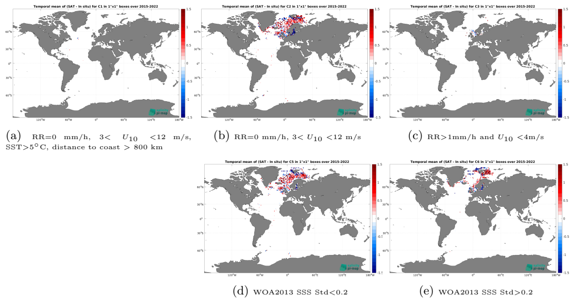
Figure 14: Temporal mean gridded over spatial boxes of size 1^\circ \times 1^\circ of \Delta SSS (SMAP SSS L2 v5.0 (JPL) - ICES) for 5 different subdatasets corresponding to: RR=0 mm/h, 3 < U_{10} < 12 m/s, SST > 5°C, distance to coast > 800 km (a), RR=0 mm/h, 3 < U_{10} < 12 m/s (b), RR > 1mm/h and U_{10} < 4 m/s (c), WOA2013 SSS Std < 0.2 (d), WOA2013 SSS Std > 0.2 (e).
