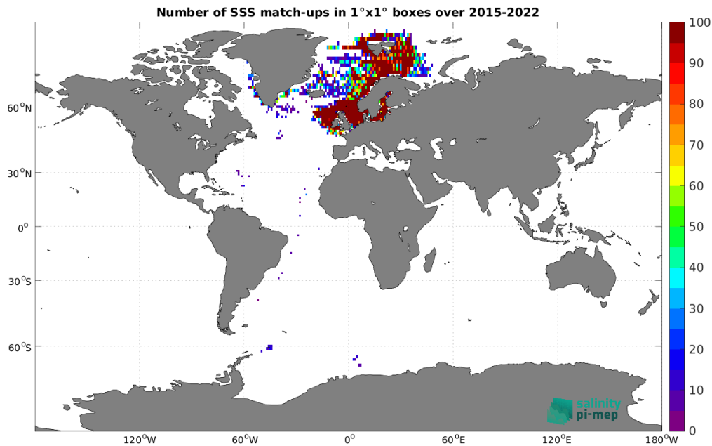
Figure 5: Number of SSS match-ups between ICES SSS and the SMAP SSS L2 v5.0 (JPL) SSS product for the Global Ocean Pi-MEP region over 1^\circ \times 1^\circ boxes and for the full satellite product period.
