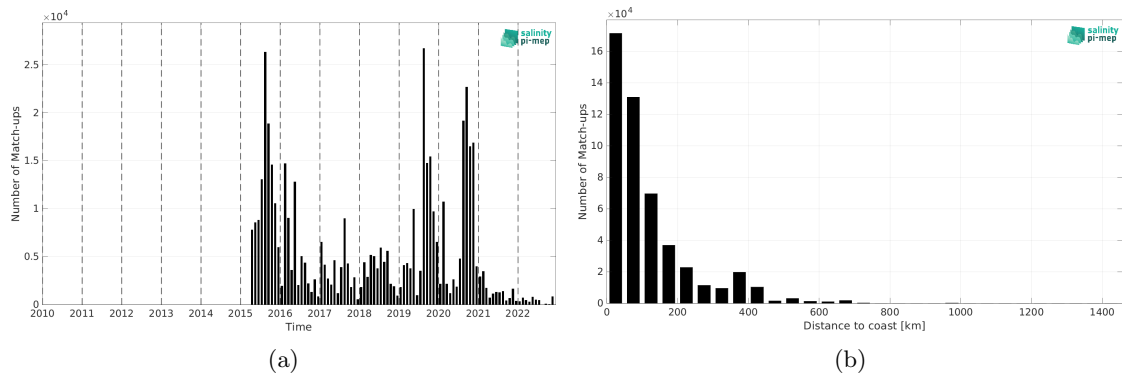
Figure 2: Number of match-ups between ICES and SMAP SSS L2 v5.0 (JPL) SSS as a function of time (a) and as function of the distance to coast (b) over the Global Ocean Pi-MEP region and for the full satellite product period.
