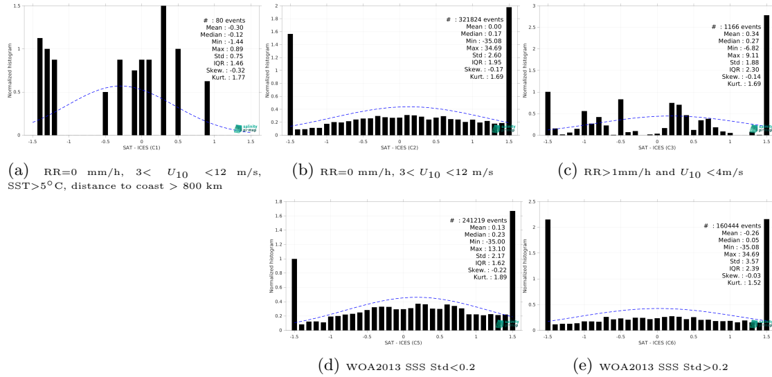
Figure 15: Normalized histogram of \Delta SSS (SMAP SSS L2 v5.0 (JPL) - ICES) for 5 different subdatasets corresponding to: RR=0 mm/h, 3 < U_{10} < 12 m/s, SST>5°C, distance to coast > 800 km (a), RR=0 mm/h, 3 < U_{10} < 12 m/s (b), RR>1mm/h and U_{10} < 4 m/s (c), WOA2013 SSS Std<0.2 (d), WOA2013 SSS Std>0.2 (e).
