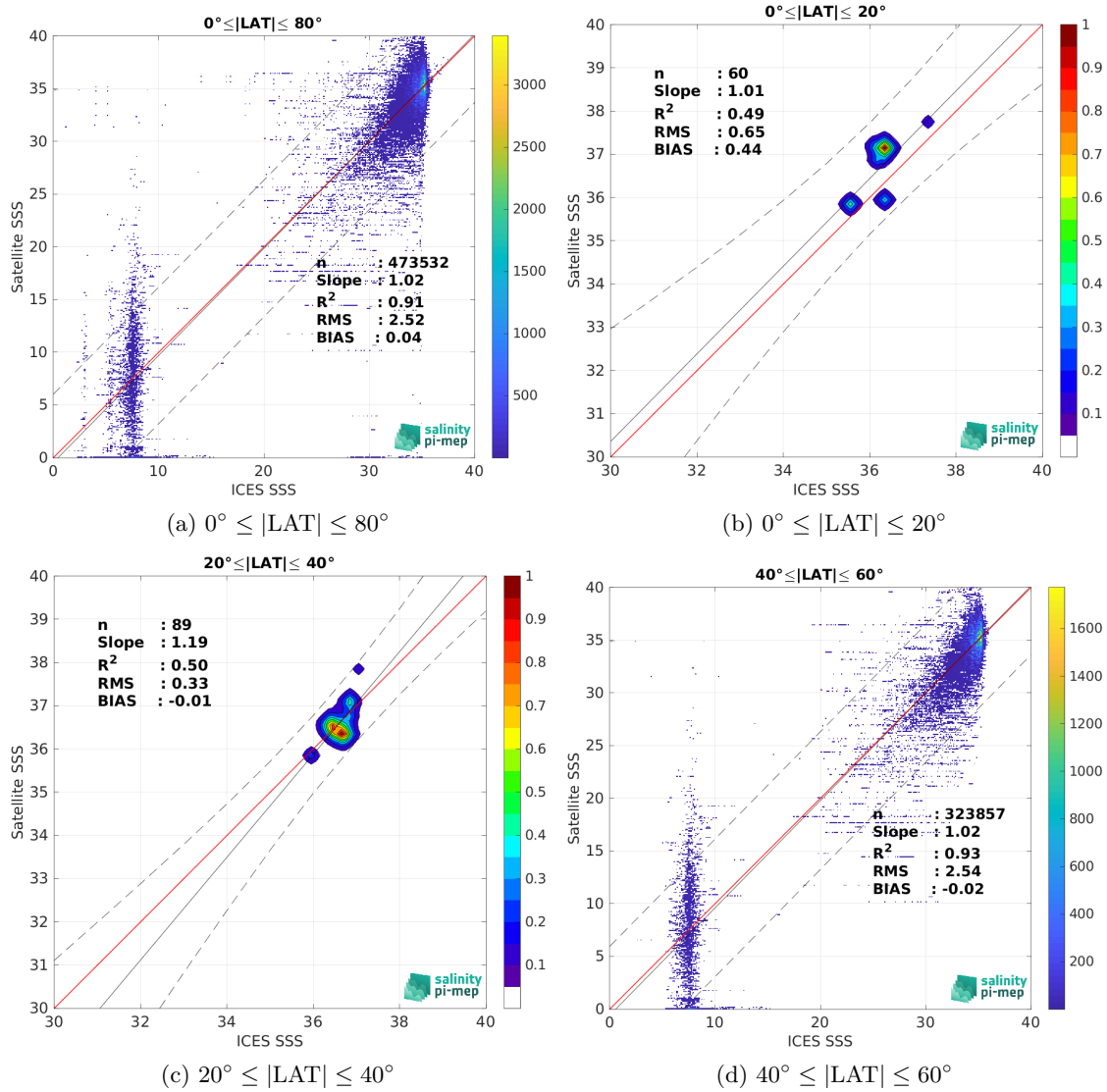
Figure 10: Contour maps of the concentration of SMAP SSS L2 v5.0 (JPL) SSS (y-axis) versus ICES SSS (x-axis) at match-up pairs for different latitude bands. For each plot, the red line shows x=y . The black thin and dashed lines indicate a linear fit through the data cloud and the \pm 95\% confidence levels, respectively. The number match-up pairs n , the slope and R^2 coefficient of the linear fit, the root mean square (RMS) and the mean bias between satellite and in situ data are indicated for each latitude band in each plots.
