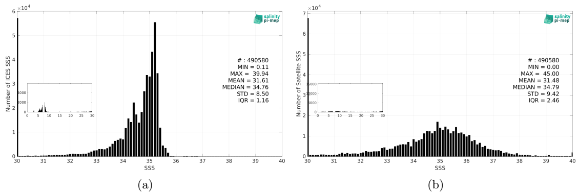
Figure 3: Histograms of SSS from ICES (a) and SMAP SSS L2 v5.0 (JPL) (b) considering all match-up pairs per bins of 0.1 over the Global Ocean Pi-MEP region and for the full satellite product period.
