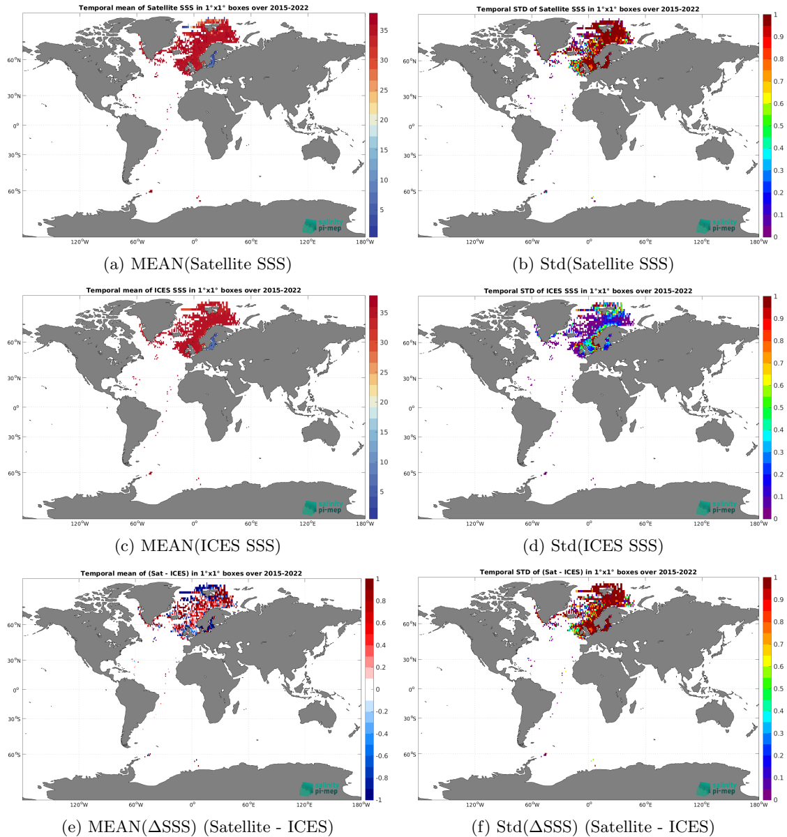
Figure 7: Temporal mean (left) and Std (right) of SSS from SMAP SSS L2 v5.0 (JPL) (top), ICES (middle), and of \Delta SSS (Satellite - ICES). Only match-up pairs are used to generate these maps.
