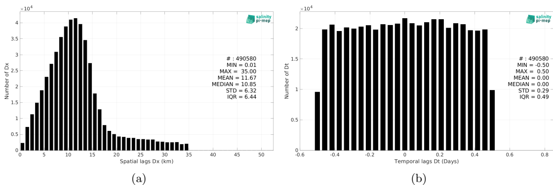
Figure 6: Histograms of the spatial (a) and temporal (b) lags between the location/time of the ICES measurement and the date of the corresponding SMAP SSS L2 v5.0 (JPL) SSS pixel.
