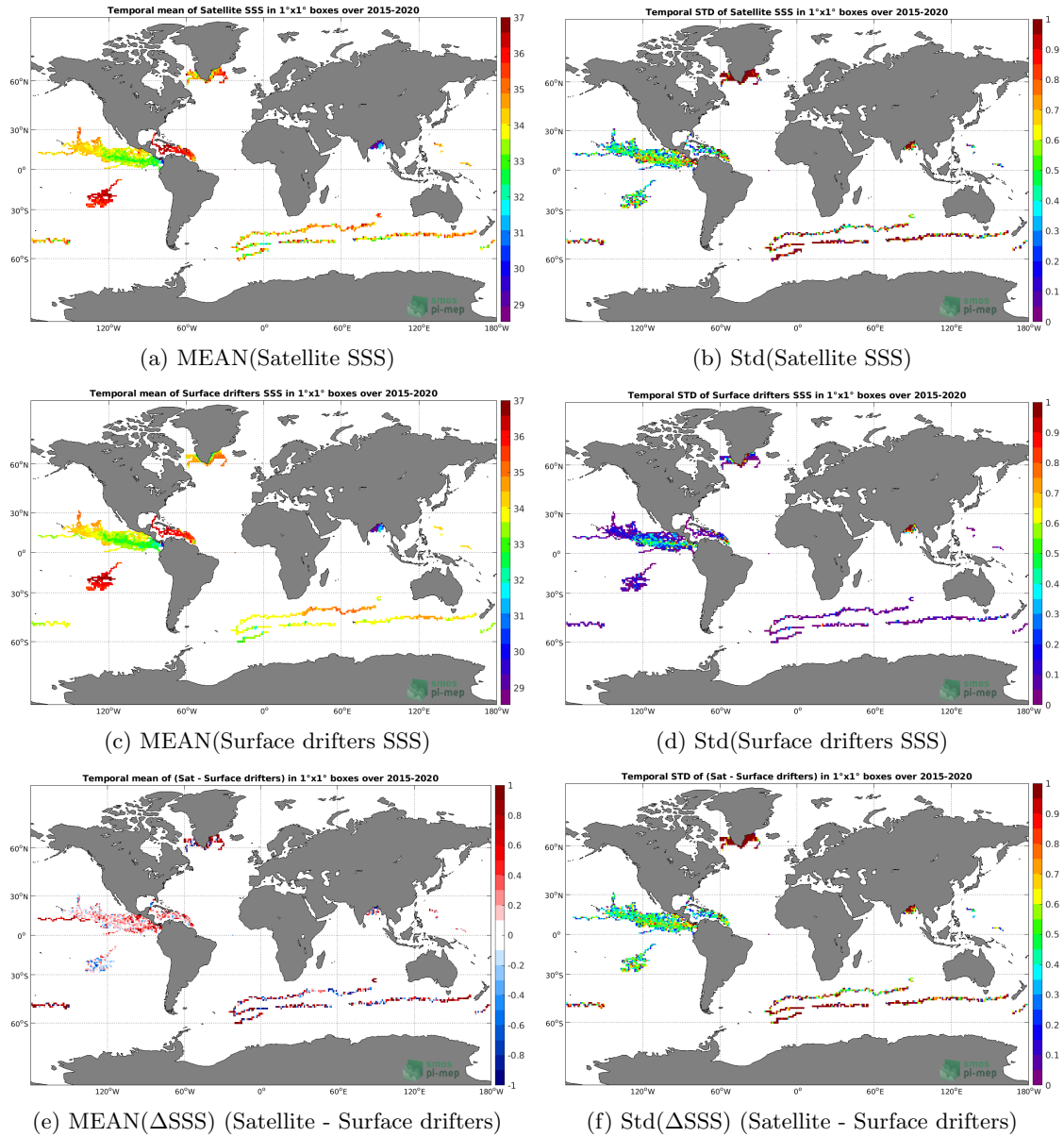
Figure 5: Temporal mean (left) and Std (right) of SSS from SMAP SSS L2 v5.0 (JPL) (top), Surface drifters (middle), and of \Delta SSS (Satellite - Surface drifters). Only match-up pairs are used to generate these maps.
