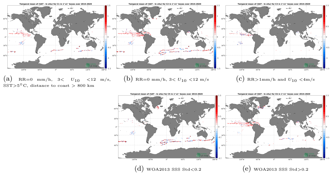
Figure 11: Temporal mean gridded over spatial boxes of size 1^\circ \times 1^\circ of \Delta SSS (SMAP SSS L2 v5.0 (JPL) - Surface drifters) for 5 different subdatasets corresponding to:RR=0 mm/h, 3 < U_{10} < 12 m/s, SST>5°C, distance to coast > 800 km (a), RR=0 mm/h, 3 < U_{10} < 12 m/s (b), RR>1mm/h and U_{10} < 4 m/s (c), WOA2013 SSS Std<0.2 (d), WOA2013 SSS Std>0.2 (e).
