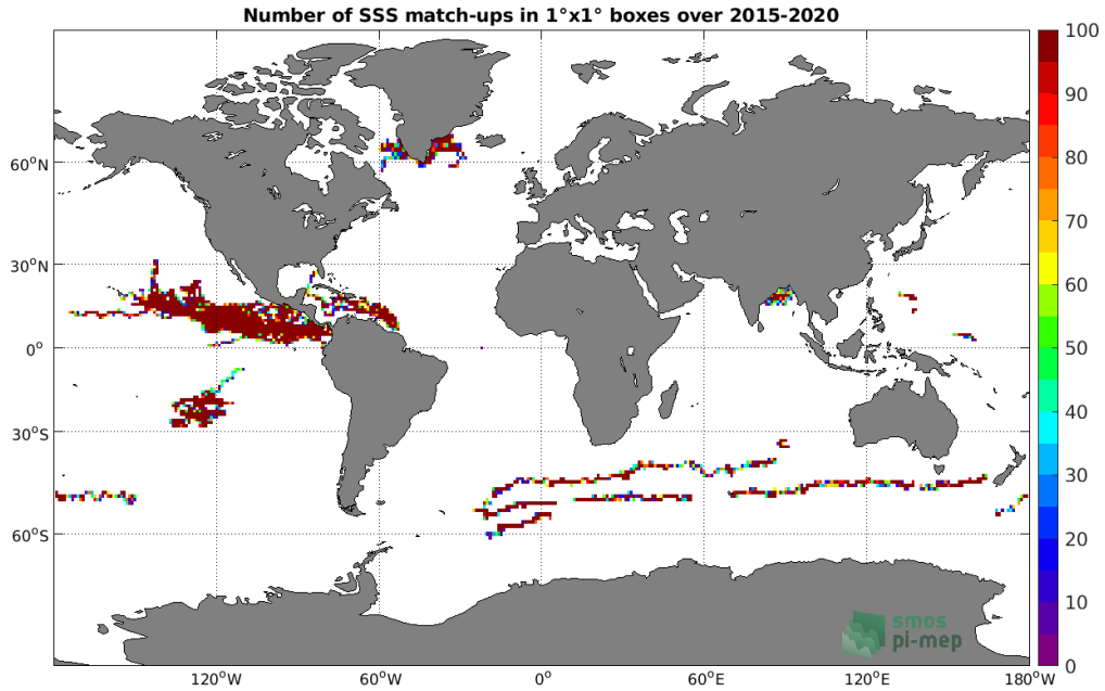
Figure 3: Number of SSS match-ups between Surface drifters SSS and the SMAP SSS L2 v5.0 (JPL) SSS product for the Global Ocean Pi-MEP region over 1^\circ \times 1^\circ boxes and for the full satellite product period.
