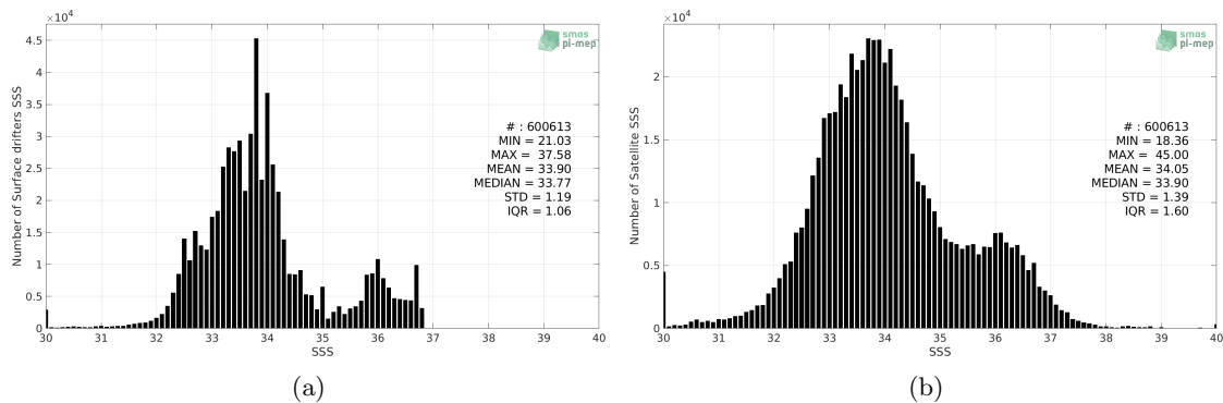
Figure 2: Histograms of SSS from Surface drifters (a) and SMAP SSS L2 v5.0 (JPL) (b) considering all match-up pairs per bins of 0.1 over the Global Ocean Pi-MEP region and for the full satellite product period.
