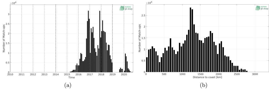
Figure 1: Number of match-ups between Surface drifters and SMAP SSS L2 v5.0 (JPL) SSS as a function of time (a) and as function of the distance to coast (b) over the Global Ocean Pi-MEP region and for the full satellite product period.
