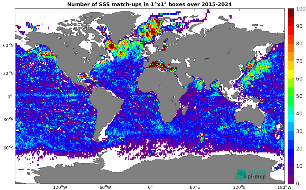
Figure 5: Number of SSS match-ups between Argo SSS and the SMAP SSS L2 v5.0 (JPL) SSS product for the Global Ocean Pi-MEP region over 1^\circ \times 1^\circ boxes and for the full satellite product period.
