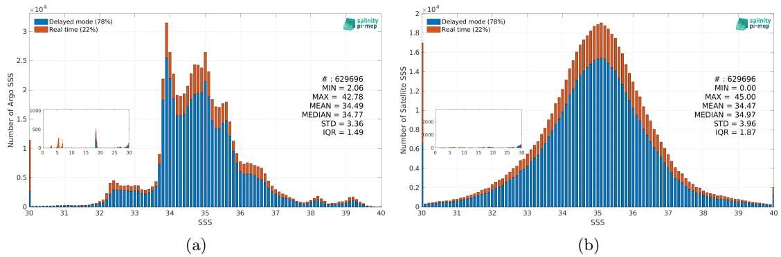
Figure 3: Histograms of SSS from Argo (a) and SMAP SSS L2 v5.0 (JPL) (b) considering all match-up pairs per bins of 0.1 over the Global Ocean Pi-MEP region and for the full satellite product period.
