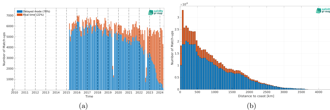
Figure 2: Number of match-ups between Argo and SMAP SSS L2 v5.0 (JPL) SSS as a function of time (a) and as function of the distance to coast (b) over the Global Ocean Pi-MEP region and for the full satellite product period.
