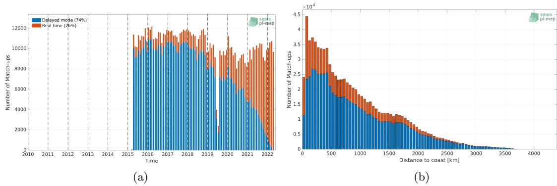
Figure 1: Number of match-ups between Argo and SMAP SSS L2 v5.0 (JPL) SSS as a function of time (a) and as function of the distance to coast (b) over the Global Ocean Pi-MEP region and for the full satellite product period.
