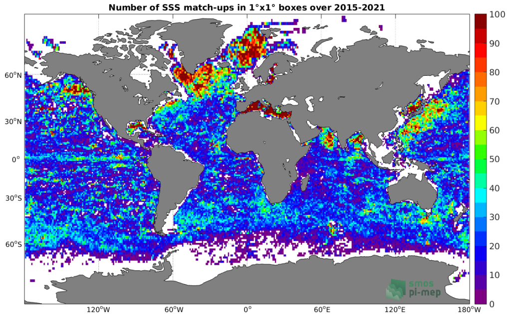
Figure 4: Number of SSS match-ups between Argo SSS and the SMAP SSS L2 v5.0 (JPL) SSS product for the Global Ocean Pi-MEP region over 1^\circ \times 1^\circ boxes and for the full satellite product period.
