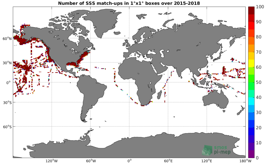
Figure 4: Number of SSS match-ups between TSG-SAMOS SSS and the SMAP-L2-JPL-V4 SSS product for the Global Ocean Pi-MEP region over 1°x1° boxes and for the full satellite product period.
