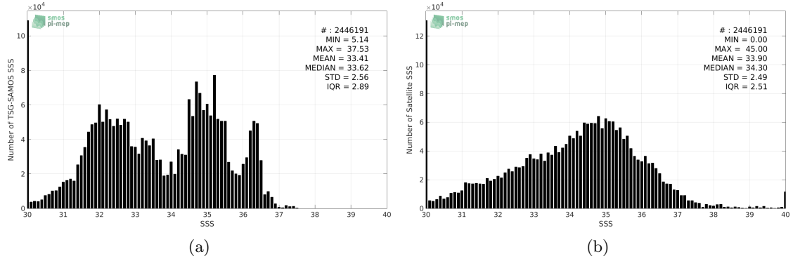
Figure 2: Histograms of SSS from TSG-SAMOS (a) and SMAP-L2-JPL-V4 (b) considering all match-up pairs per bins of 0.1 over the Global Ocean Pi-MEP region and for the full satellite product period.
