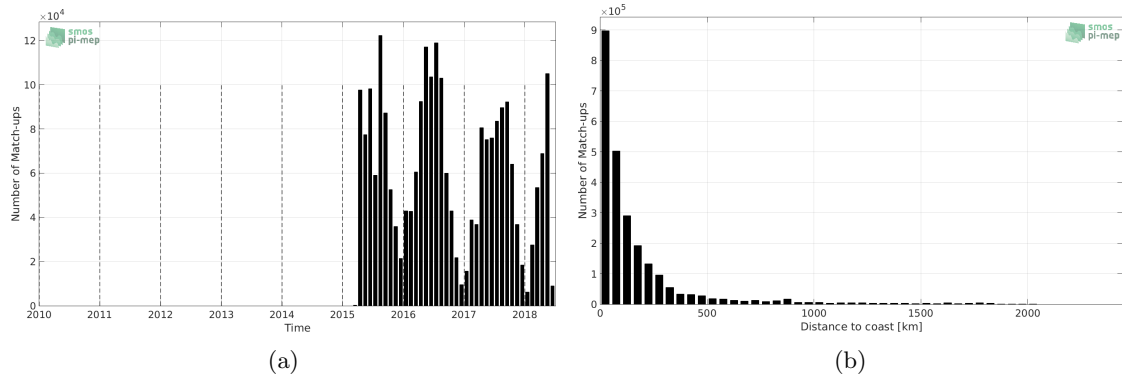
Figure 1: Number of match-ups between TSG-SAMOS and SMAP-L2-JPL-V4 SSS as a function of time (a) and as function of the distance to coast (b) over the Global Ocean Pi-MEP region and for the full satellite product period.
