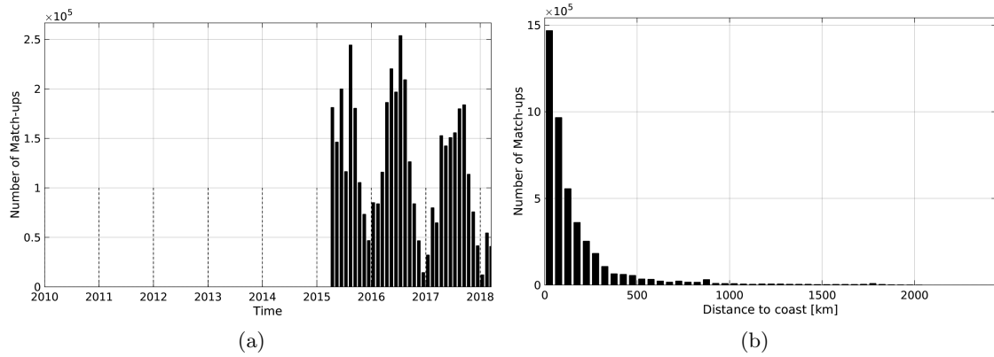
Figure 1: Number of match-ups between TSG-SAMOS and SMAP-L2-JPL-V4 SSS as a function of time (a) and as function of the distance to coast (b) over the Global Ocean Pi-MEP region and for the full satellite product period.
