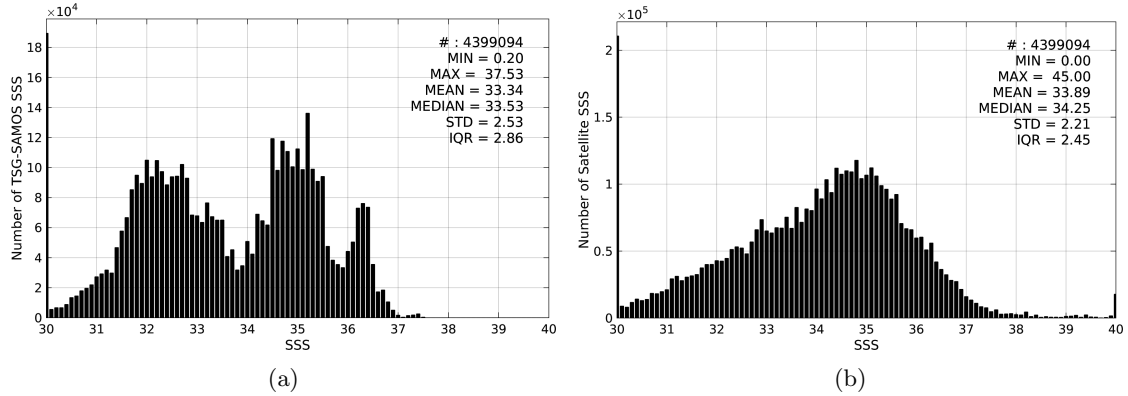
Figure 2: Histograms of SSS from TSG-SAMOS (a) and SMAP-L2-JPL-V4 (b) considering all match-up pairs per bins of 0.1 over the Global Ocean Pi-MEP region and for the full satellite product period.
