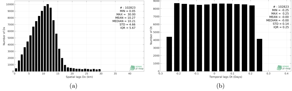
Figure 5: Histograms of the spatial (a) and temporal (b) lags between the time of the TSG-LEGOS-Survostral measurements and the date of the corresponding SMAP-L2-JPL-V4 SSS product.
