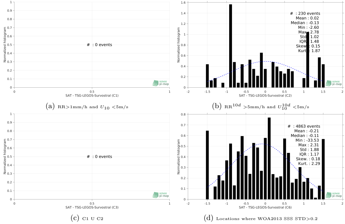
Figure 13: Normalized histogram of \Delta SSS (SMAP-L2-JPL-V4 - TSG-LEGOS-Survostral) for 6 different subdatasets corresponding to: RR > 1\text{mm/h} and U_{10} < 5\text{m/s} (a), RR^{10d} > 5\text{mm/h} and U_{10}^{10d} < 5\text{m/s} (b), C1 \cup C2 (c), Locations where WOA2013 SSS STD > 0.2 (d).
