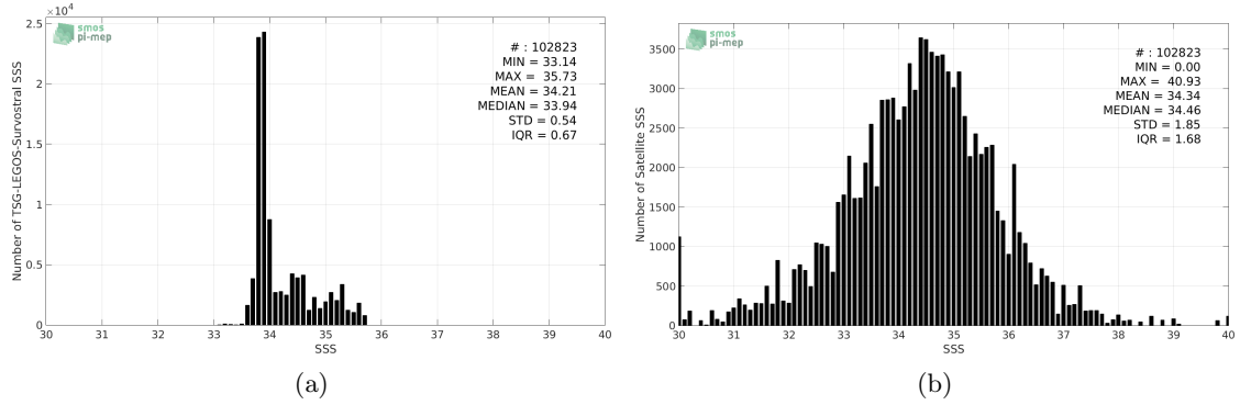
Figure 2: Histograms of SSS from TSG-LEGOS-Survostral (a) and SMAP-L2-JPL-V4 (b) considering all match-up pairs per bins of 0.1 over the Global Ocean Pi-MEP region and for the full satellite product period.
