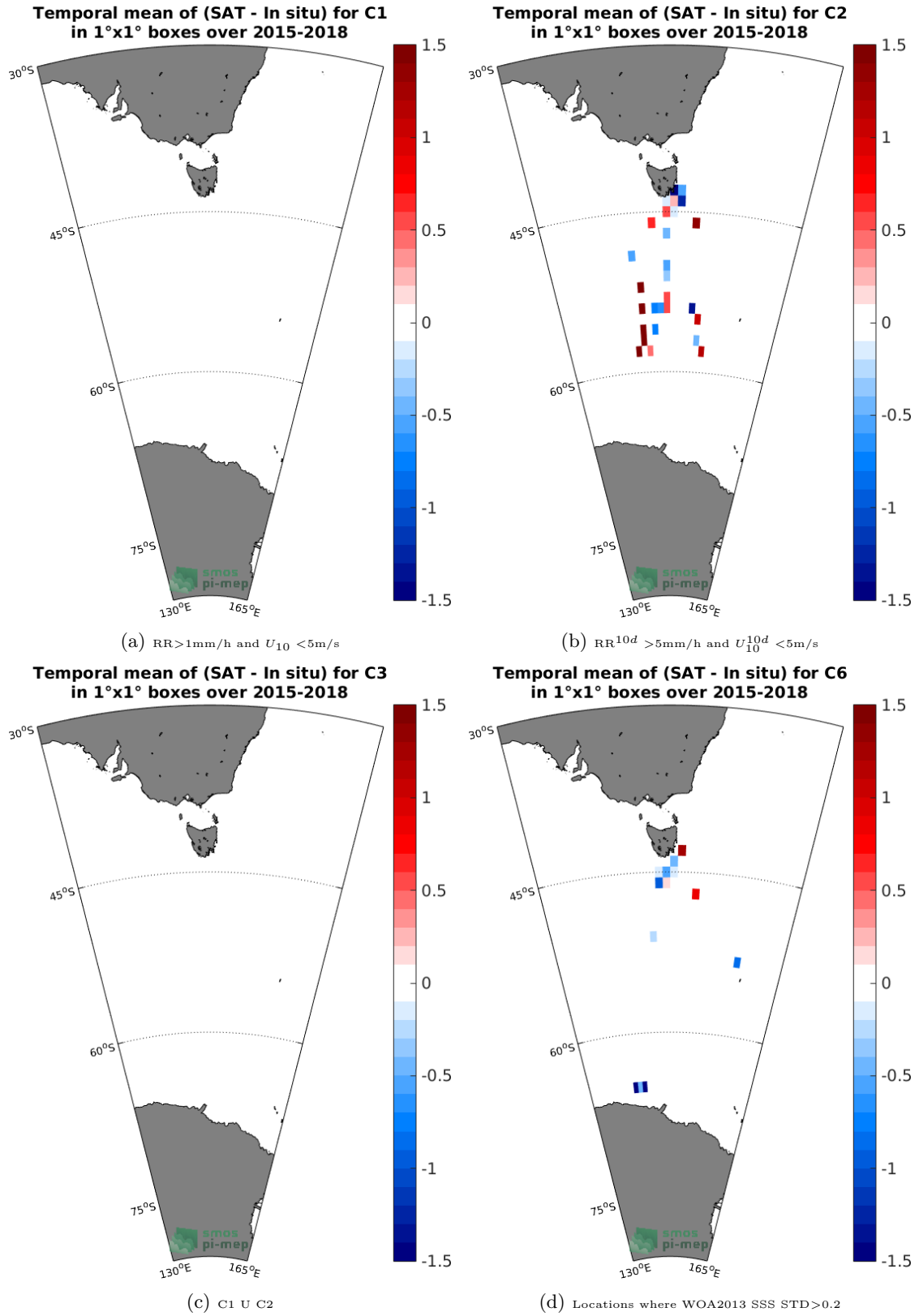
Figure 12: Temporal mean gridded over spatial boxes of size 1°x1° of \Delta\text{SSS} (SMAP-L2-JPL-V4 - TSG-LEGOS-Survostral) for 4 different subdatasets corresponding to: RR > 1\text{mm/h} and U_{10} < 5\text{m/s} (a), RR^{10d} > 5\text{mm/h} and U_{10}^{10d} < 5\text{m/s} (b), C1 U C2 (c), Locations where WOA2013 SSS STD > 0.2 (d).
