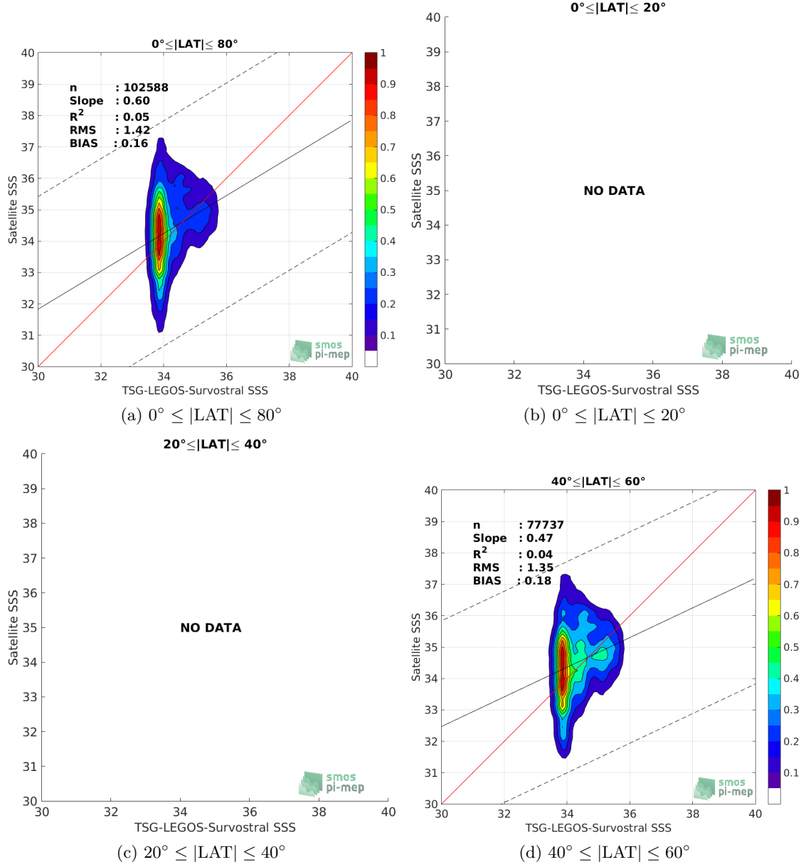
Figure 9: Contour maps of the concentration of SMAP-L2-JPL-V4 SSS (y-axis) versus TSG-LEGOS-Survostral SSS (x-axis) at match-up pairs for different latitude bands. For each plot, the red line shows x=y . The black thin and dashed lines indicate a linear fit through the data cloud and the \pm 95\% confidence levels, respectively. The number match-up pairs n , the slope and R^2 coefficient of the linear fit, the root mean square (RMS) and the mean bias between satellite and in situ data are indicated for each latitude band in each plots.
