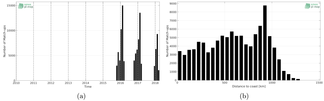
Figure 1: Number of match-ups between TSG-LEGOS-Survostral and SMAP-L2-JPL-V4 SSS as a function of time (a) and as function of the distance to coast (b) over the Global Ocean Pi-MEP region and for the full satellite product period.
