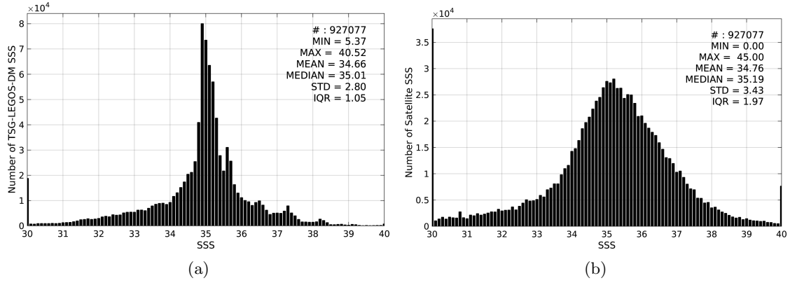
Figure 2: Histograms of SSS from TSG-LEGOS-DM (a) and SMAP-L2-JPL-V4 (b) considering all match-up pairs per bins of 0.1 over the Global Ocean Pi-MEP region and for the full satellite product period.
