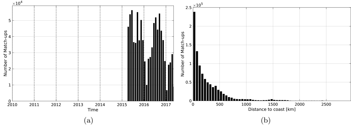
Figure 1: Number of match-ups between TSG-LEGOS-DM and SMAP-L2-JPL-V4 SSS as a function of time (a) and as function of the distance to coast (b) over the Global Ocean Pi-MEP region and for the full satellite product period.
