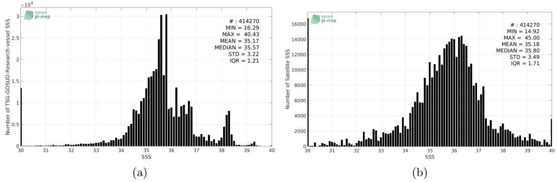
Figure 2: Histograms of SSS from TSG-GOSUD-Research-vessel (a) and SMAP-L2-JPL-V4 (b) considering all match-up pairs per bins of 0.1 over the Global Ocean Pi-MEP region and for the full satellite product period.
