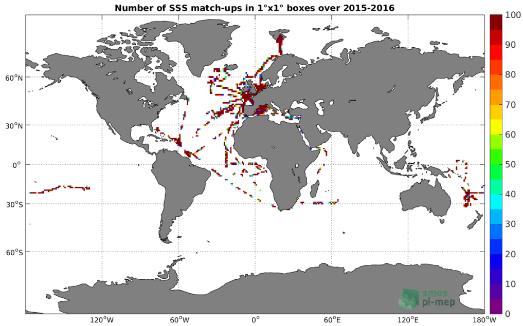
Figure 4: Number of SSS match-ups between TSG-GOSUD-Research-vessel SSS and the SMAP-L2-JPL-V4 SSS product for the Global Ocean Pi-MEP region over 1^\circ \times 1^\circ boxes and for the full satellite product period.
