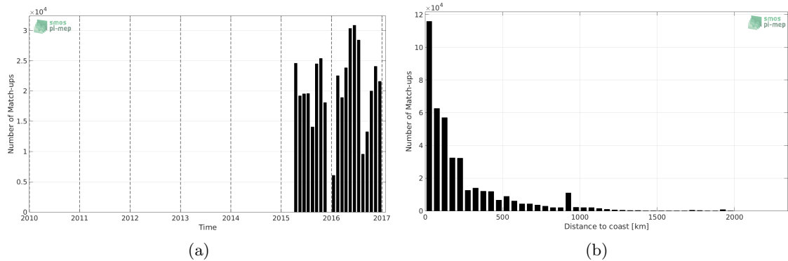
Figure 1: Number of match-ups between TSG-GOSUD-Research-vessel and SMAP-L2-JPL-V4 SSS as a function of time (a) and as function of the distance to coast (b) over the Global Ocean Pi-MEP region and for the full satellite product period.
