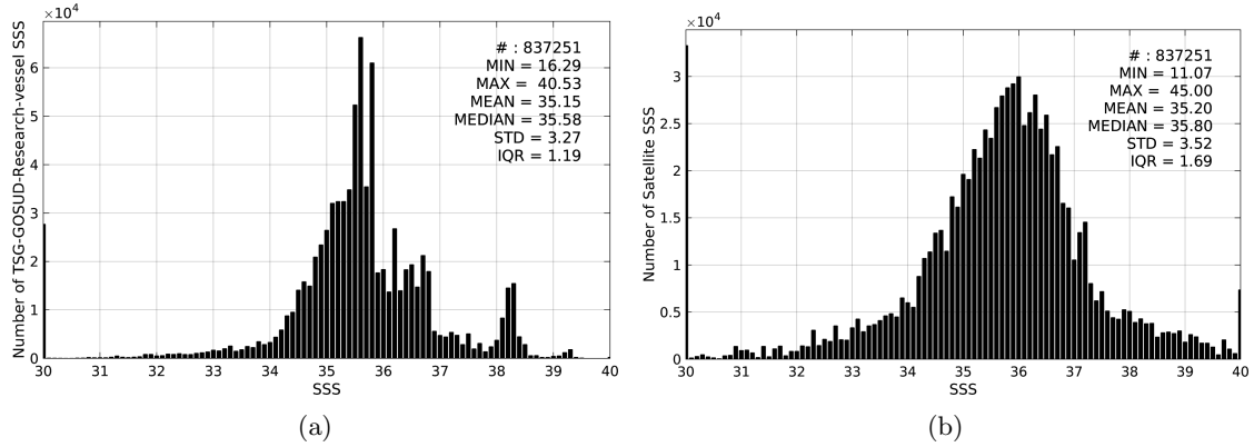
Figure 2: Histograms of SSS from TSG-GOSUD-Research-vessel (a) and SMAP-L2-JPL-V4 (b) considering all match-up pairs per bins of 0.1 over the Global Ocean Pi-MEP region and for the full satellite product period.
