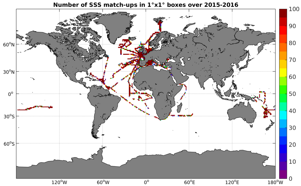
Figure 4: Number of SSS match-ups between TSG-GOSUD-Research-vessel SSS and the SMAP-L2-JPL-V4 SSS product for the Global Ocean Pi-MEP region over 1^\circ \times 1^\circ boxes and for the full satellite product period.
