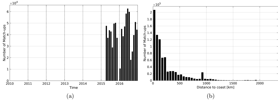
Figure 1: Number of match-ups between TSG-GOSUD-Research-vessel and SMAP-L2-JPL-V4 SSS as a function of time (a) and as function of the distance to coast (b) over the Global Ocean Pi-MEP region and for the full satellite product period.
