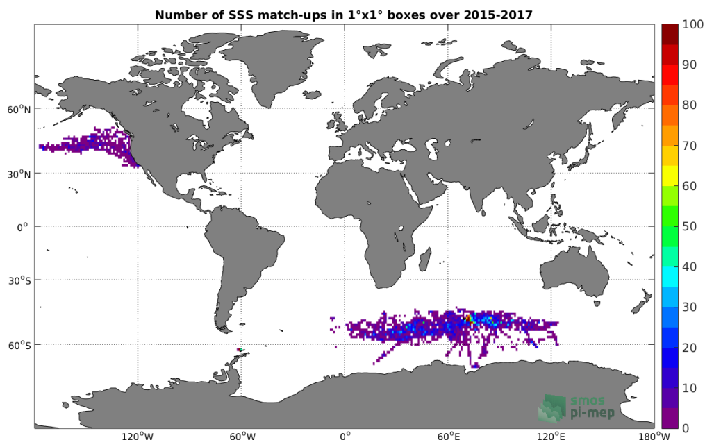
Figure 4: Number of SSS match-ups between Sea mammals SSS and the SMAP-L2-JPL-V4 SSS product for the Global Ocean Pi-MEP region over 1°x1° boxes and for the full satellite product period.
