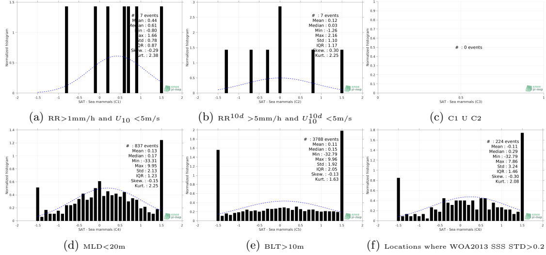
Figure 13: Normalized histogram of \Delta SSS (SMAP-L2-JPL-V4 - Sea mammals) for 6 different sub-datasets corresponding to: RR > 1\text{mm/h} and U_{10} < 5\text{m/s} (a), RR^{10d} > 5\text{mm/h} and U_{10}^{10d} < 5\text{m/s} (b), C1 U C2 (c), MLD < 20\text{m} (d), BLT > 10\text{m} (e), Locations where WOA2013 SSS STD > 0.2 (f).
