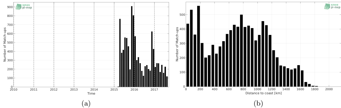
Figure 1: Number of match-ups between Sea mammals and SMAP-L2-JPL-V4 SSS as a function of time (a) and as function of the distance to coast (b) over the Global Ocean Pi-MEP region and for the full satellite product period.
