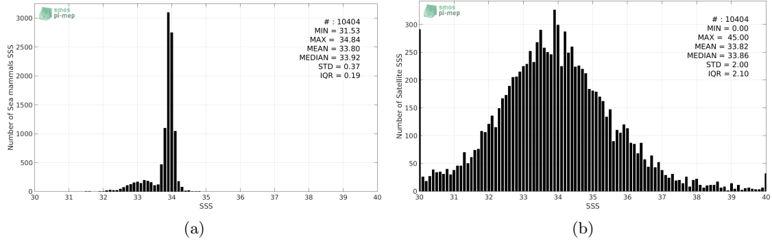
Figure 2: Histograms of SSS from Sea mammals (a) and SMAP-L2-JPL-V4 (b) considering all match-up pairs per bins of 0.1 over the Global Ocean Pi-MEP region and for the full satellite product period.
