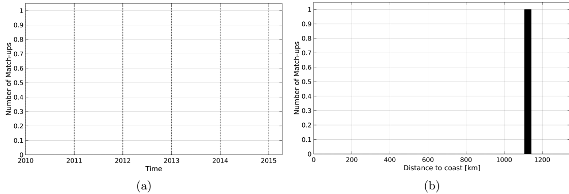
Figure 1: Number of match-ups between Surface drifters and SMAP-L2-JPL-V4 SSS as a function of time (a) and as function of the distance to coast (b) over the Global Ocean Pi-MEP region and for the full satellite product period.
