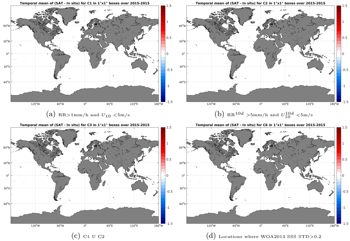
Figure 11: Temporal mean gridded over spatial boxes of size 1^\circ \times 1^\circ of \Delta SSS (SMAP-L2-JPL-V4 - Surface drifters) for 4 different subdatasets corresponding to: RR > 1\text{mm/h} and U_{10} < 5\text{m/s} (a), RR^{10d} > 5\text{mm/h} and U_{10}^{10d} < 5\text{m/s} (b), C1 U C2 (c), Locations where WOA2013 SSS STD > 0.2 (d).
