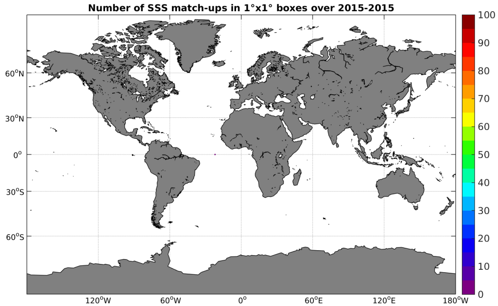
Figure 3: Number of SSS match-ups between Surface drifters SSS and the SMAP-L2-JPL-V4 SSS product for the Global Ocean Pi-MEP region over 1°x1° boxes and for the full satellite product period.
