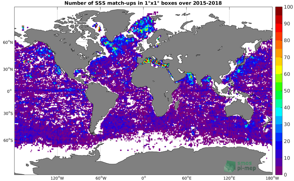
Figure 4: Number of SSS match-ups between Argo SSS and the SMAP-L2-JPL-V4 SSS product for the Global Ocean Pi-MEP region over 1^\circ \times 1^\circ boxes and for the full satellite product period.
