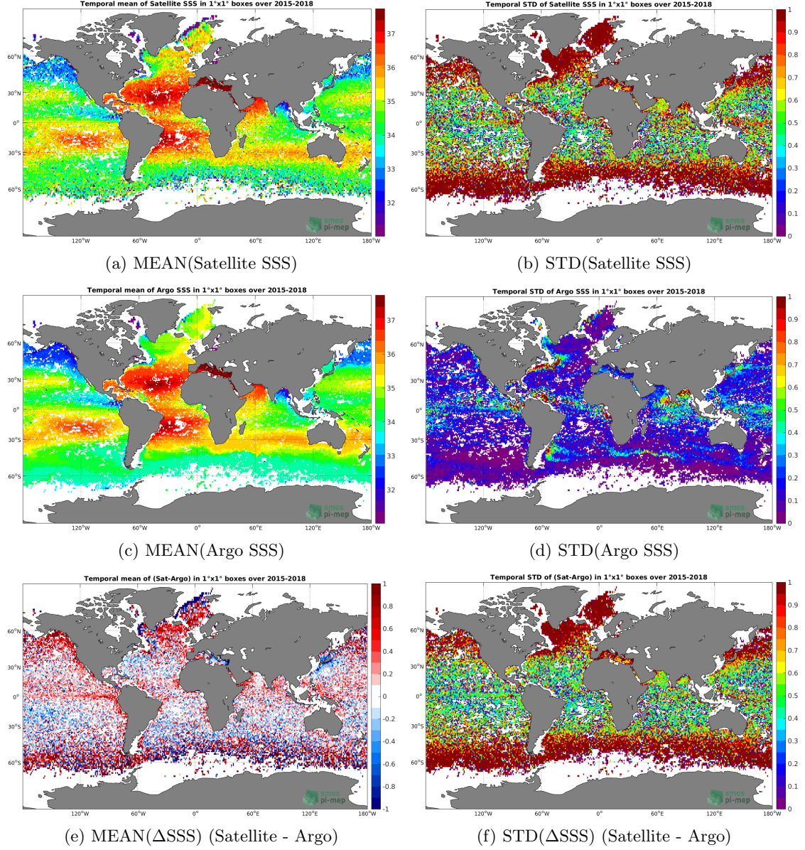
Figure 6: Temporal mean (left) and STD (right) of SSS from SMAP-L2-JPL-V4 (top), Argo (middle), and of \Delta\text{SSS} (Satellite - Argo). Only match-up pairs are used to generate these maps.
