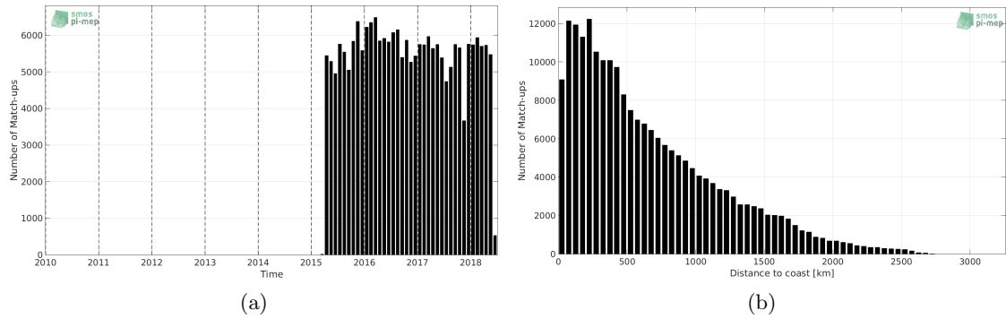
Figure 1: Number of match-ups between Argo and SMAP-L2-JPL-V4 SSS as a function of time (a) and as function of the distance to coast (b) over the Global Ocean Pi-MEP region and for the full satellite product period.
