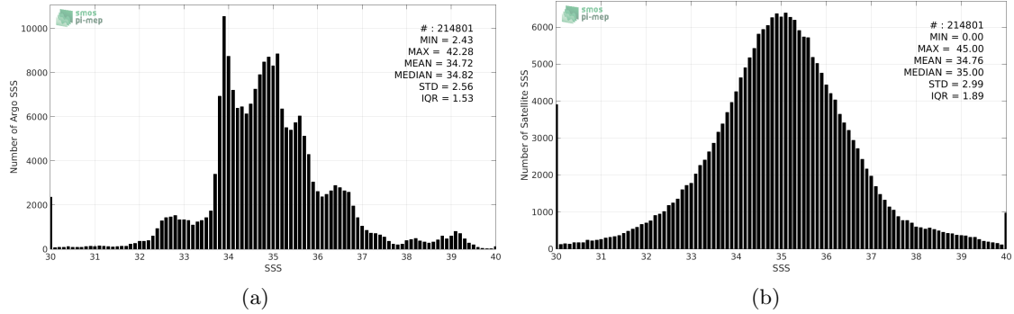
Figure 2: Histograms of SSS from Argo (a) and SMAP-L2-JPL-V4 (b) considering all match-up pairs per bins of 0.1 over the Global Ocean Pi-MEP region and for the full satellite product period.
