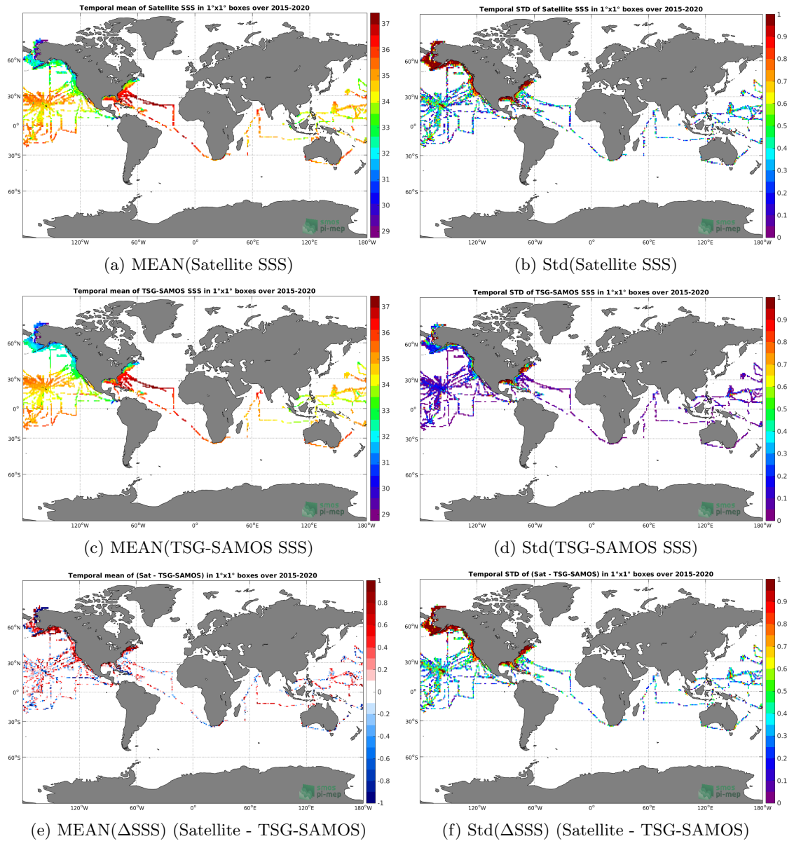
Figure 6: Temporal mean (left) and Std (right) of SSS from SMAP-L2-JPL-V4.3 (top), TSG-SAMOS (middle), and of \Delta SSS (Satellite - TSG-SAMOS). Only match-up pairs are used to generate these maps.
