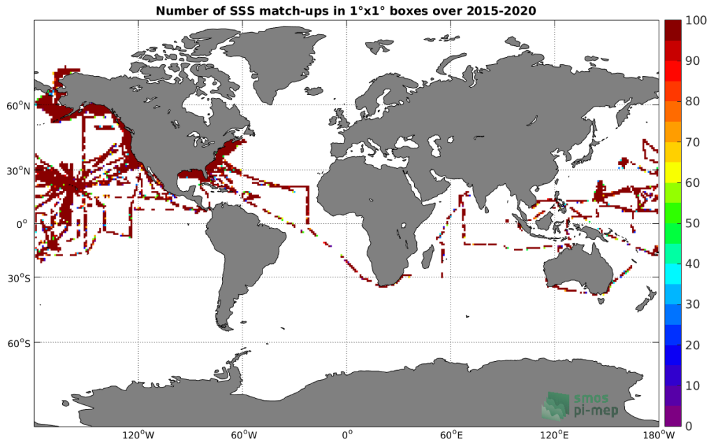
Figure 4: Number of SSS match-ups between TSG-SAMOS SSS and the SMAP-L2-JPL-V4.3 SSS product for the Global Ocean Pi-MEP region over 1°x1° boxes and for the full satellite product period.
