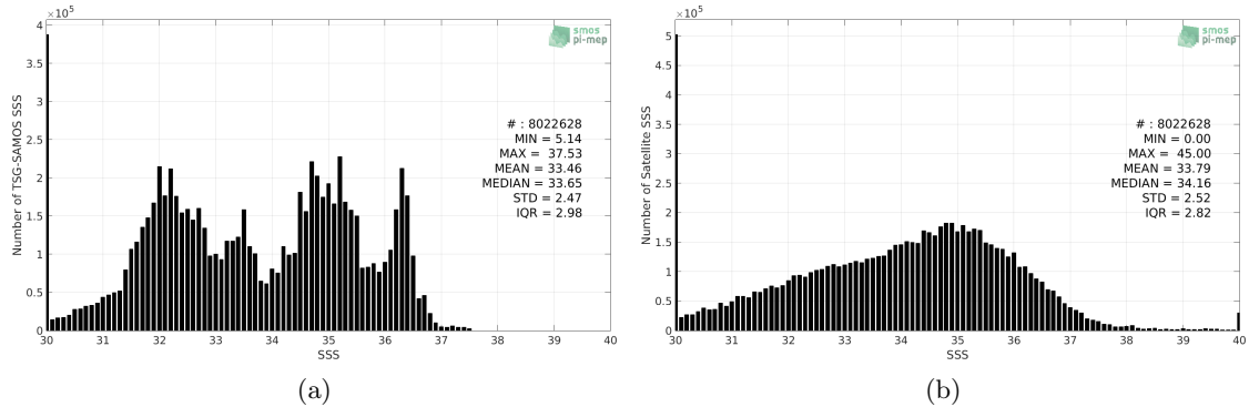
Figure 2: Histograms of SSS from TSG-SAMOS (a) and SMAP-L2-JPL-V4.3 (b) considering all match-up pairs per bins of 0.1 over the Global Ocean Pi-MEP region and for the full satellite product period.
