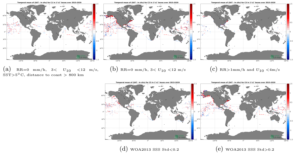
Figure 12: Temporal mean gridded over spatial boxes of size 1^\circ \times 1^\circ of \Delta SSS (SMAP-L2-JPL-V4.3 - TSG-SAMOS) for 5 different subdatasets corresponding to:RR=0 mm/h, 3 < U_{10} < 12 m/s, SST >5^\circ C, distance to coast > 800 km (a), RR=0 mm/h, 3 < U_{10} < 12 m/s (b), RR >1 mm/h and U_{10} < 4 m/s (c), WOA2013 SSS Std <0.2 (d), WOA2013 SSS Std >0.2 (e).
