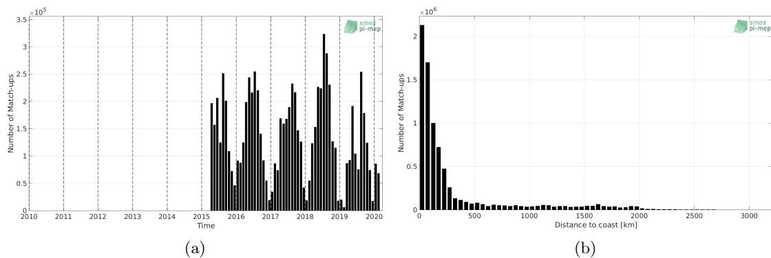
Figure 1: Number of match-ups between TSG-SAMOS and SMAP-L2-JPL-V4.3 SSS as a function of time (a) and as function of the distance to coast (b) over the Global Ocean Pi-MEP region and for the full satellite product period.
