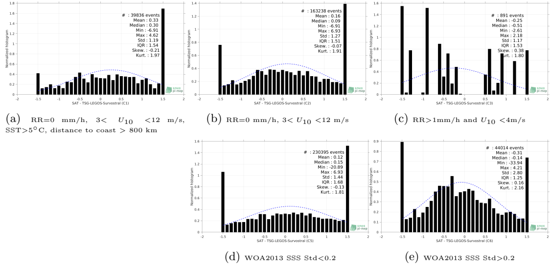
Figure 13: Normalized histogram of \Delta SSS (SMAP-L2-JPL-V4.3 - TSG-LEGOS-Survostral) for 5 different subdatasets corresponding to: RR=0 mm/h, 3 < U_{10} < 12 m/s, SST > 5°C, distance to coast > 800 km (a), RR=0 mm/h, 3 < U_{10} < 12 m/s (b), RR > 1mm/h and U_{10} < 4 m/s (c), WOA2013 SSS Std < 0.2 (d), WOA2013 SSS Std > 0.2 (e).
