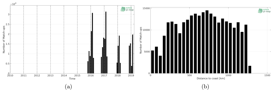
Figure 1: Number of match-ups between TSG-LEGOS-Survostral and SMAP-L2-JPL-V4.3 SSS as a function of time (a) and as function of the distance to coast (b) over the Global Ocean Pi-MEP region and for the full satellite product period.
