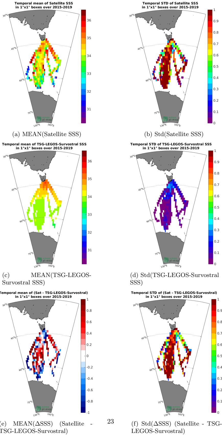
Figure 6: Temporal mean (left) and Std (right) of SSS from SMAP-L2-JPL-V4.3 (top), TSG-LEGOS-Survostral (middle), and of \Delta SSS (Satellite - TSG-LEGOS-Survostral). Only match-up pairs are used to generate these maps.
