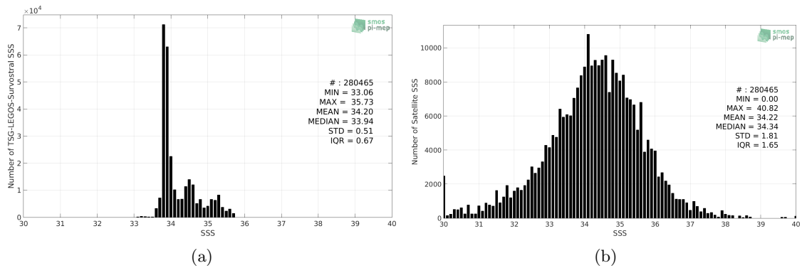
Figure 2: Histograms of SSS from TSG-LEGOS-Survostral (a) and SMAP-L2-JPL-V4.3 (b) considering all match-up pairs per bins of 0.1 over the Global Ocean Pi-MEP region and for the full satellite product period.
