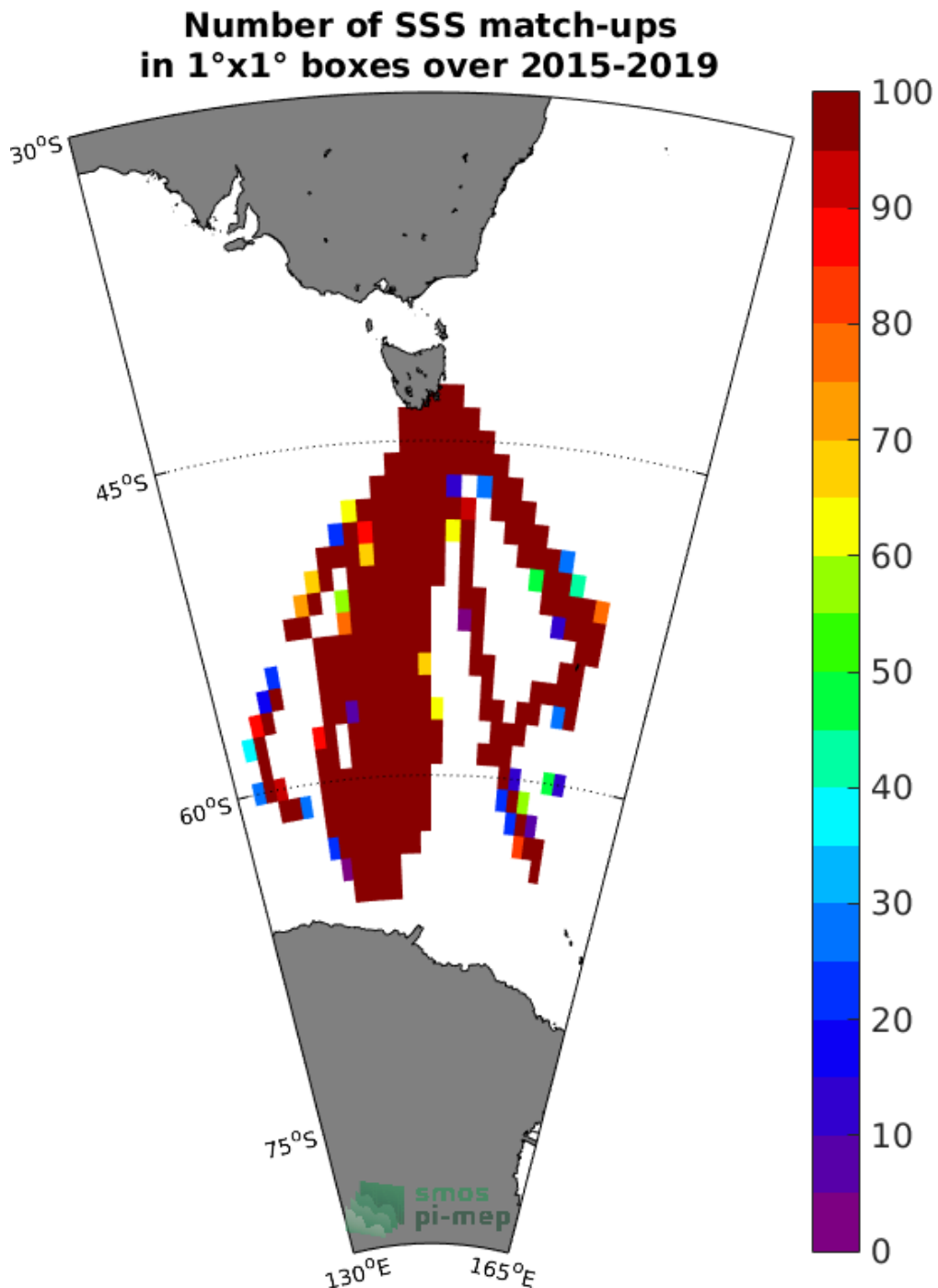
Figure 4: Number of SSS match-ups between TSG-LEGOS-Survostral SSS and the SMAP-L2-JPL-V4.3 SSS product for the Global Ocean Pi-MEP region over 1°x1° boxes and for the full satellite product period.
