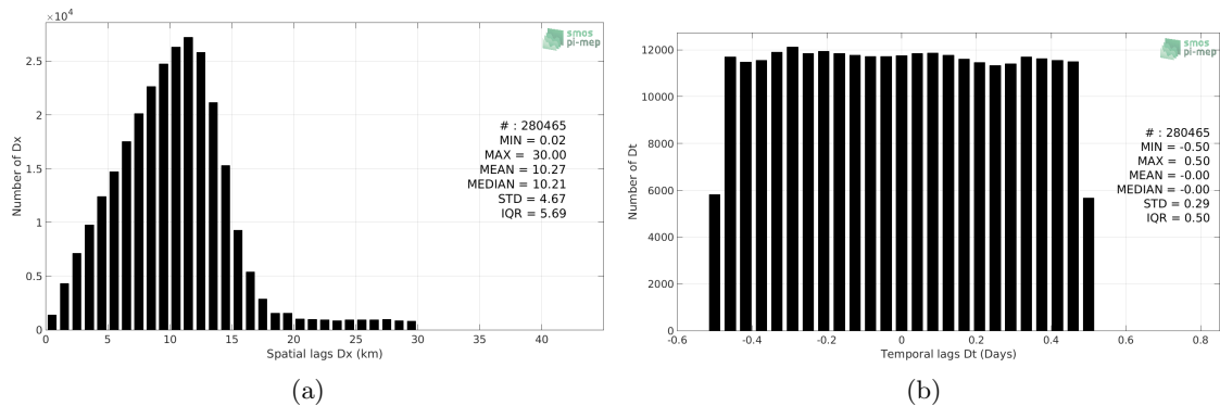
Figure 5: Histograms of the spatial (a) and temporal (b) lags between the time of the TSG-LEGOS-Survostral measurements and the date of the corresponding SMAP-L2-JPL-V4.3 SSS product.
