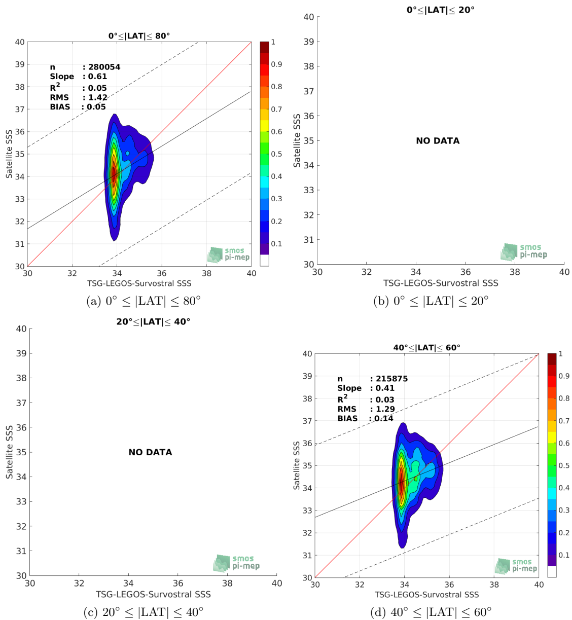
Figure 9: Contour maps of the concentration of SMAP-L2-JPL-V4.3 SSS (y-axis) versus TSG-LEGOS-Survostral SSS (x-axis) at match-up pairs for different latitude bands. For each plot, the red line shows x=y . The black thin and dashed lines indicate a linear fit through the data cloud and the \pm 95\% confidence levels, respectively. The number match-up pairs n , the slope and R^2 coefficient of the linear fit, the root mean square (RMS) and the mean bias between satellite and in situ data are indicated for each latitude band in each plots.
