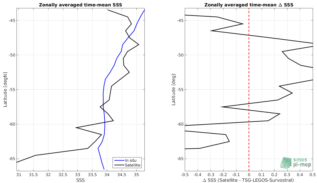
Figure 8: Left panel: Zonal mean SSS from SMAP-L2-JPL-V4.3 satellite product (black) and from TSG-LEGOS-Survostral (blue). Right panel: Zonal mean of \Delta SSS (Satellite - TSG-LEGOS-Survostral) for all the collected Pi-MEP match-up pairs estimated over the full satellite product period.
