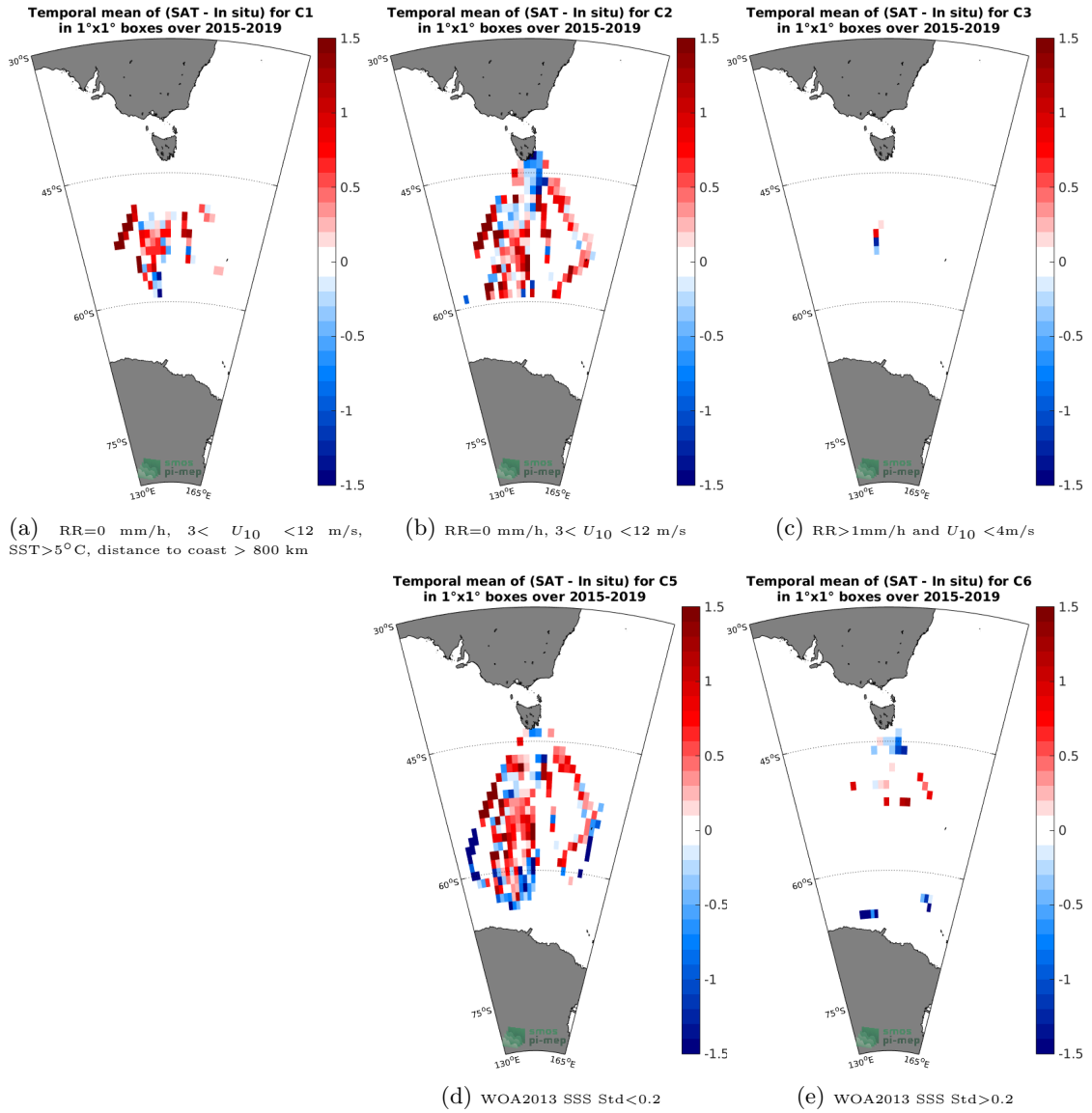
Figure 12: Temporal mean gridded over spatial boxes of size 1°x1° of \Delta SSS (SMAP-L2-JPL-V4.3 - TSG-LEGOS-Survostral) for 5 different subdatasets corresponding to:RR=0 mm/h, 3 < U_{10} < 12 m/s, SST>5°C, distance to coast > 800 km (a), RR=0 mm/h, 3 < U_{10} < 12 m/s (b), RR>1mm/h and U_{10} < 4 m/s (c), WOA2013 SSS Std<0.2 (d), WOA2013 SSS Std>0.2 (e).
