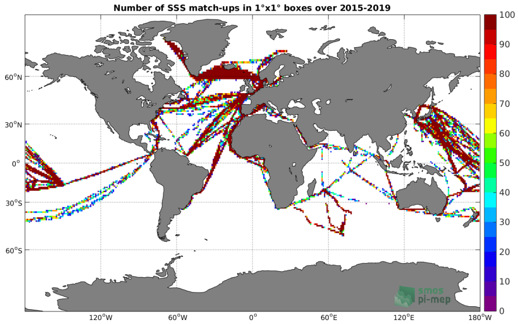
Figure 4: Number of SSS match-ups between TSG-LEGOS-DM SSS and the SMAP-L2-JPL-V4.3 SSS product for the Global Ocean Pi-MEP region over 1°x1° boxes and for the full satellite product period.
