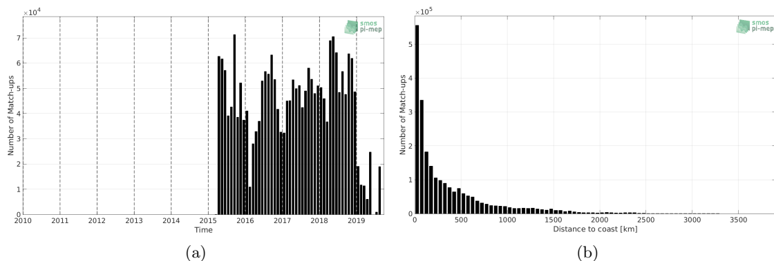
Figure 1: Number of match-ups between TSG-LEGOS-DM and SMAP-L2-JPL-V4.3 SSS as a function of time (a) and as function of the distance to coast (b) over the Global Ocean Pi-MEP region and for the full satellite product period.
