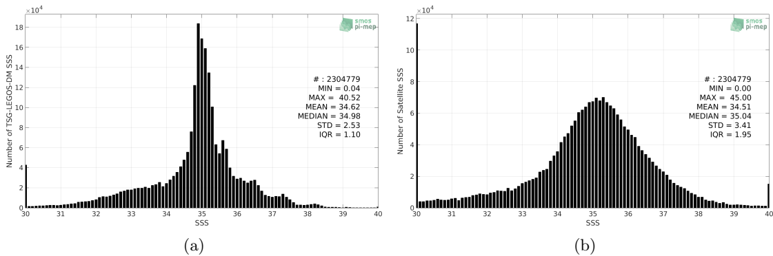
Figure 2: Histograms of SSS from TSG-LEGOS-DM (a) and SMAP-L2-JPL-V4.3 (b) considering all match-up pairs per bins of 0.1 over the Global Ocean Pi-MEP region and for the full satellite product period.
