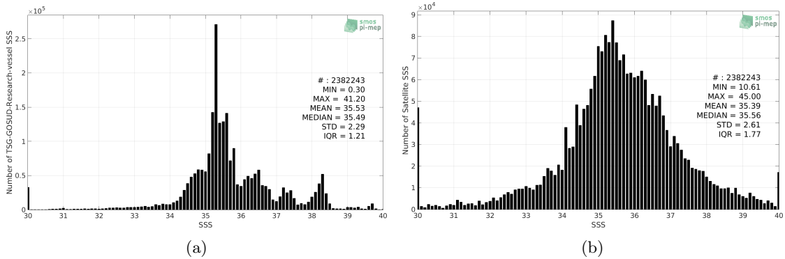
Figure 2: Histograms of SSS from TSG-GOSUD-Research-vessel (a) and SMAP-L2-JPL-V4.3 (b) considering all match-up pairs per bins of 0.1 over the Global Ocean Pi-MEP region and for the full satellite product period.
