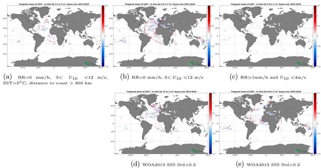
Figure 12: Temporal mean gridded over spatial boxes of size 1^\circ \times 1^\circ of \Delta SSS (SMAP-L2-JPL-V4.3 - TSG-GOSUD-Research-vessel) for 5 different subdatasets corresponding to:RR=0 mm/h, 3 < U_{10} < 12 m/s, SST >5^\circ C, distance to coast > 800 km (a), RR=0 mm/h, 3 < U_{10} < 12 m/s (b), RR >1 mm/h and U_{10} < 4 m/s (c), WOA2013 SSS Std <0.2 (d), WOA2013 SSS Std >0.2 (e).
