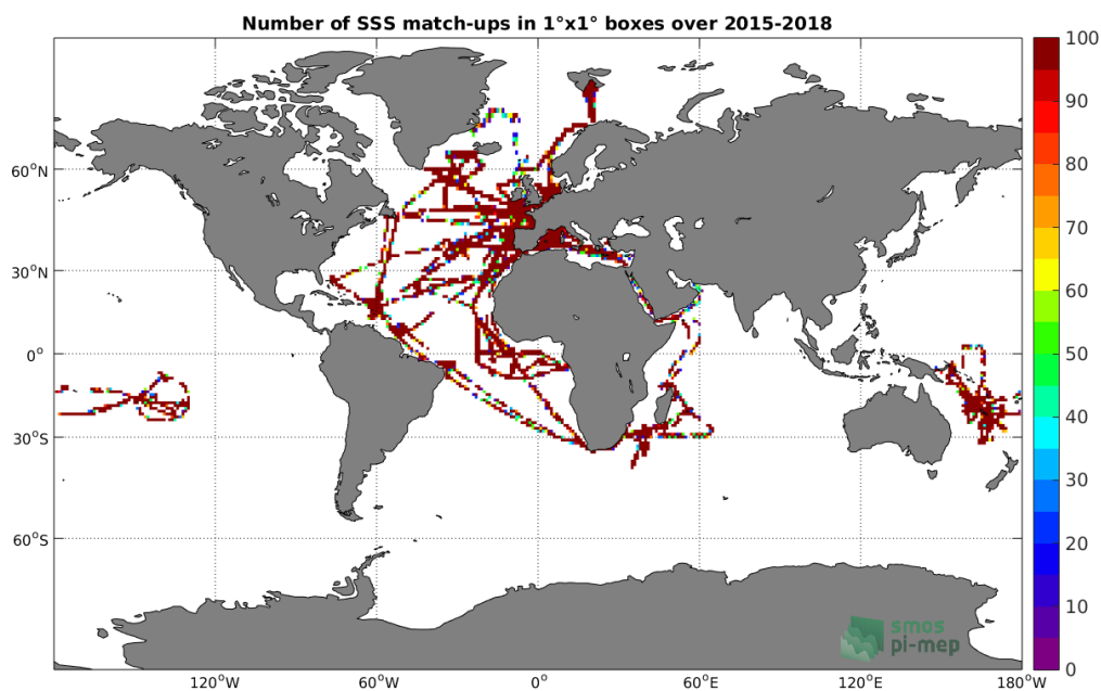
Figure 4: Number of SSS match-ups between TSG-GOSUD-Research-vessel SSS and the SMAP-L2-JPL-V4.3 SSS product for the Global Ocean Pi-MEP region over 1^\circ \times 1^\circ boxes and for the full satellite product period.
