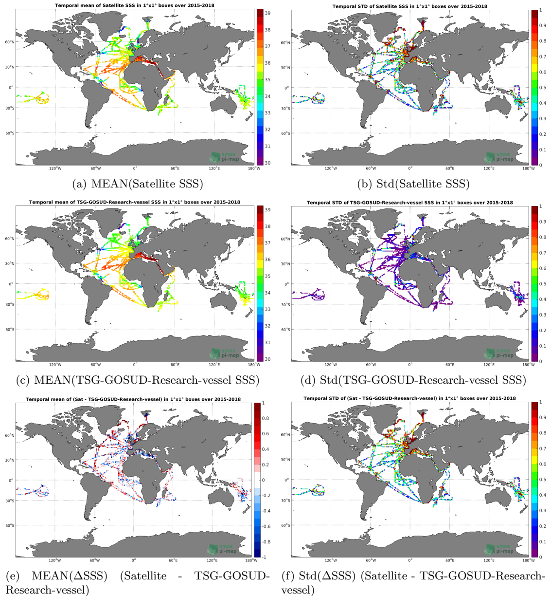
Figure 6: Temporal mean (left) and Std (right) of SSS from SMAP-L2-JPL-V4.3 (top), TSG-GOSUD-Research-vessel (middle), and of \Delta SSS (Satellite - TSG-GOSUD-Research-vessel). Only match-up pairs are used to generate these maps.
