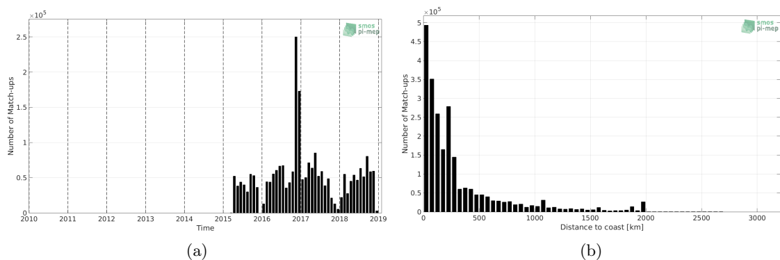
Figure 1: Number of match-ups between TSG-GOSUD-Research-vessel and SMAP-L2-JPL-V4.3 SSS as a function of time (a) and as function of the distance to coast (b) over the Global Ocean Pi-MEP region and for the full satellite product period.
