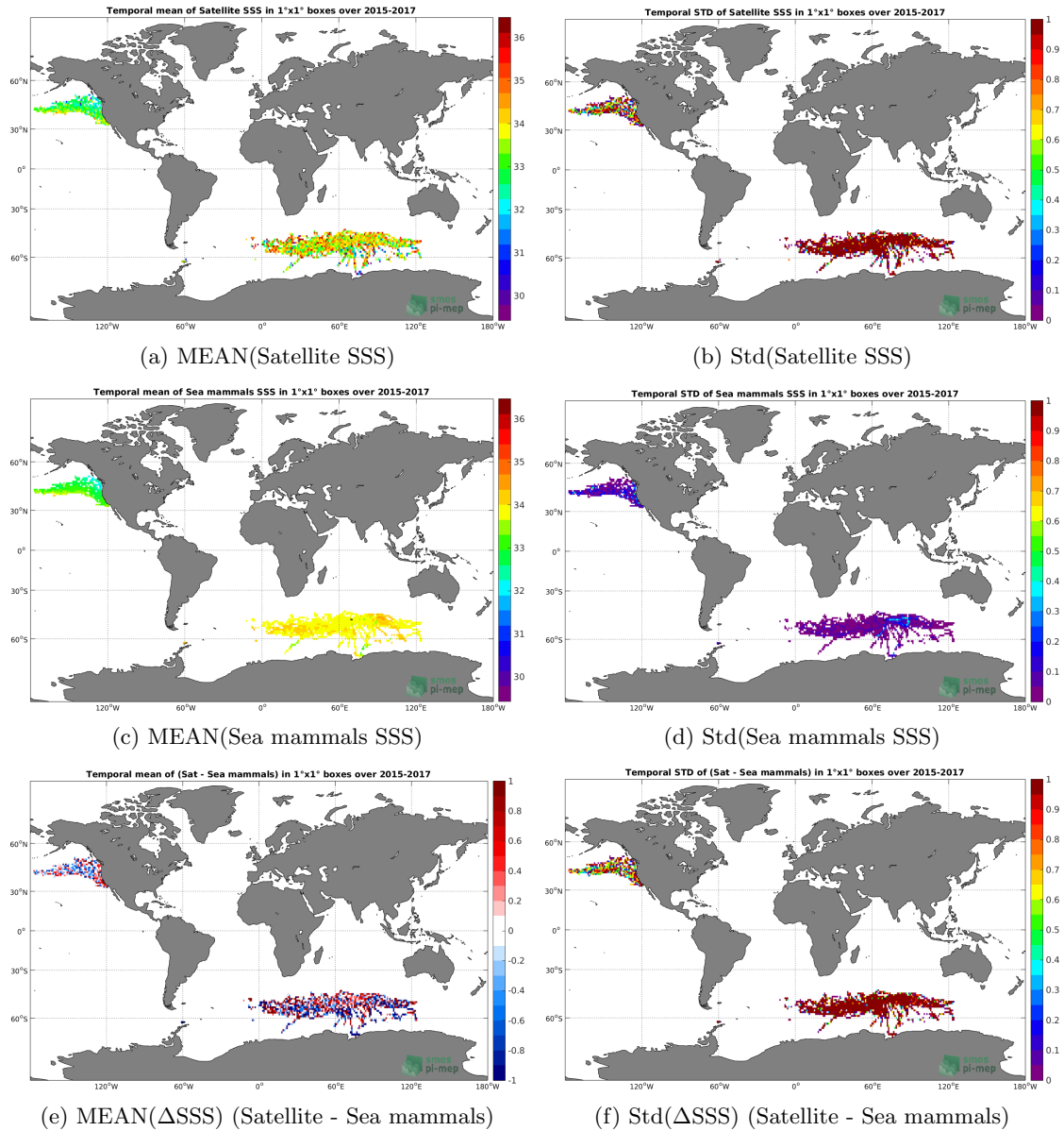
Figure 6: Temporal mean (left) and Std (right) of SSS from SMAP-L2-JPL-V4.3 (top), Sea mammals (middle), and of \Delta SSS (Satellite - Sea mammals). Only match-up pairs are used to generate these maps.
