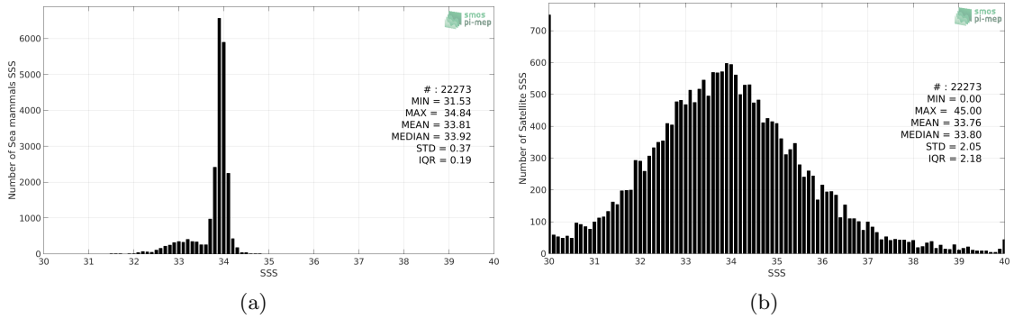
Figure 2: Histograms of SSS from Sea mammals (a) and SMAP-L2-JPL-V4.3 (b) considering all match-up pairs per bins of 0.1 over the Global Ocean Pi-MEP region and for the full satellite product period.
