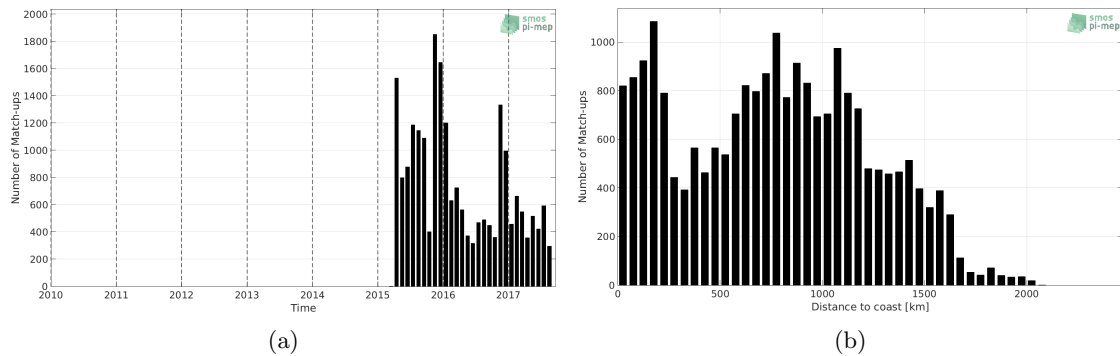
Figure 1: Number of match-ups between Sea mammals and SMAP-L2-JPL-V4.3 SSS as a function of time (a) and as function of the distance to coast (b) over the Global Ocean Pi-MEP region and for the full satellite product period.
