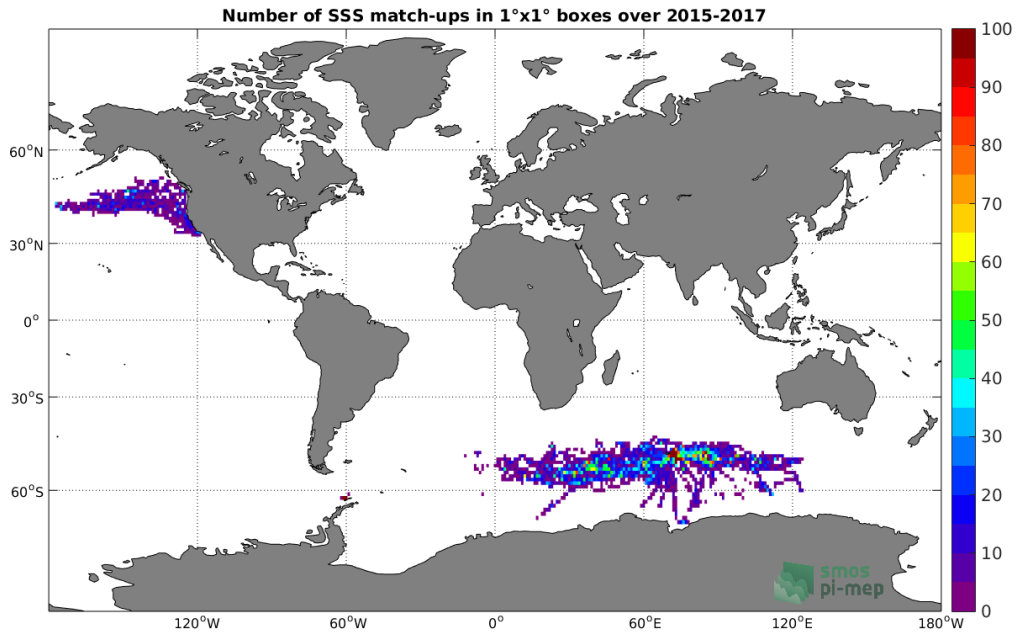
Figure 4: Number of SSS match-ups between Sea mammals SSS and the SMAP-L2-JPL-V4.3 SSS product for the Global Ocean Pi-MEP region over 1°x1° boxes and for the full satellite product period.
