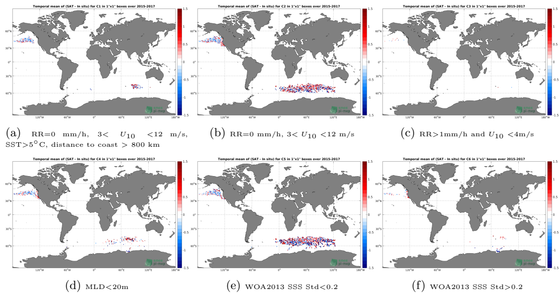
Figure 12: Temporal mean gridded over spatial boxes of size 1^\circ \times 1^\circ of \Delta SSS (SMAP-L2-JPL-V4.3 - Sea mammals) for 6 different subdatasets corresponding to:RR=0 mm/h, 3 < U_{10} < 12 m/s, SST >5^\circ\text{C} , distance to coast > 800 km (a), RR=0 mm/h, 3 < U_{10} < 12 m/s (b), RR >1 mm/h and U_{10} < 4 m/s (c),MLD <20 m (d),WOA2013 SSS Std <0.2 (e),WOA2013 SSS Std >0.2 (f).
