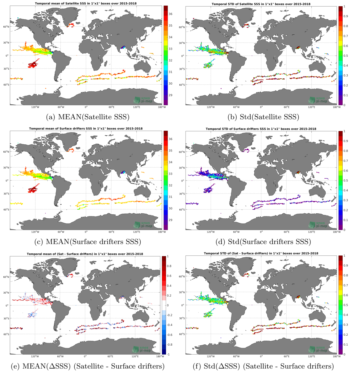
Figure 5: Temporal mean (left) and Std (right) of SSS from SMAP-L2-JPL-V4.3 (top), Surface drifters (middle), and of \Delta SSS (Satellite - Surface drifters). Only match-up pairs are used to generate these maps.
