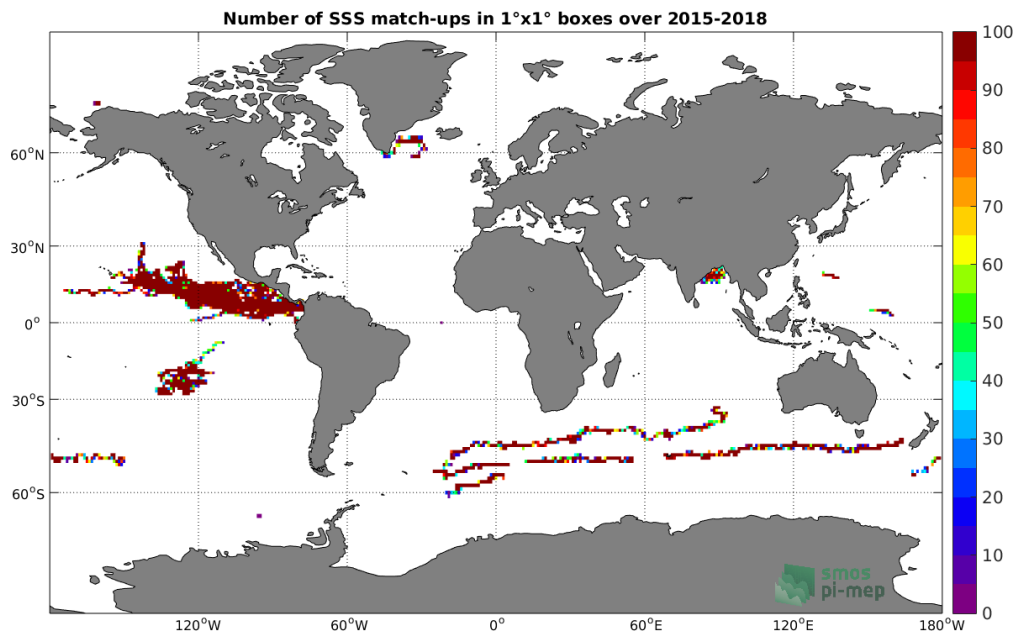
Figure 3: Number of SSS match-ups between Surface drifters SSS and the SMAP-L2-JPL-V4.3 SSS product for the Global Ocean Pi-MEP region over 1°x1° boxes and for the full satellite product period.
