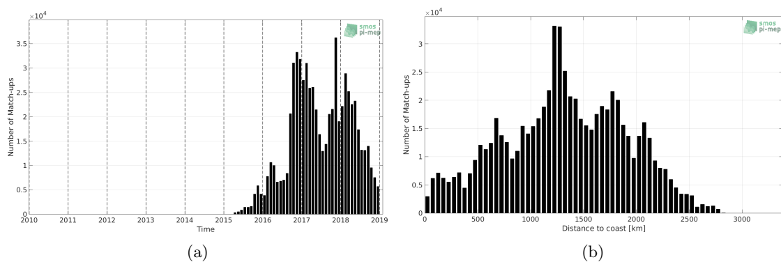
Figure 1: Number of match-ups between Surface drifters and SMAP-L2-JPL-V4.3 SSS as a function of time (a) and as function of the distance to coast (b) over the Global Ocean Pi-MEP region and for the full satellite product period.
