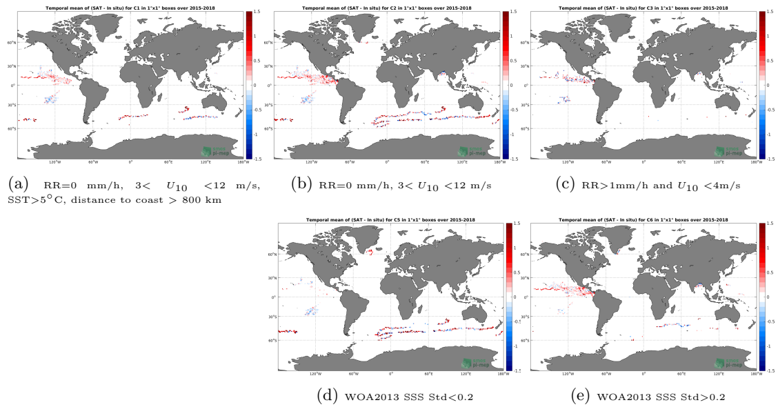
Figure 11: Temporal mean gridded over spatial boxes of size 1^\circ \times 1^\circ of \Delta SSS (SMAP-L2-JPL-V4.3 - Surface drifters) for 5 different subdatasets corresponding to: RR=0 mm/h, 3 < U_{10} < 12 m/s, SST > 5^\circ C, distance to coast > 800 km (a), RR=0 mm/h, 3 < U_{10} < 12 m/s (b), RR > 1 mm/h and U_{10} < 4 m/s (c), WOA2013 SSS Std < 0.2 (d), WOA2013 SSS Std > 0.2 (e).
