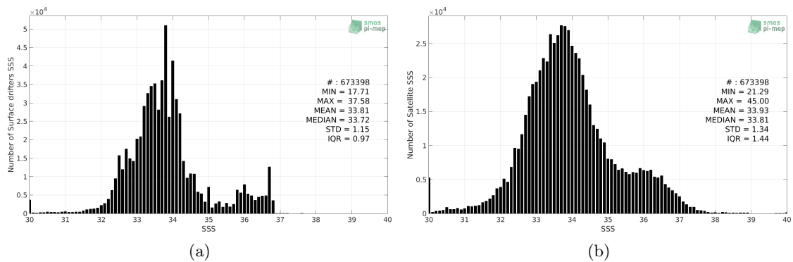
Figure 2: Histograms of SSS from Surface drifters (a) and SMAP-L2-JPL-V4.3 (b) considering all match-up pairs per bins of 0.1 over the Global Ocean Pi-MEP region and for the full satellite product period.
