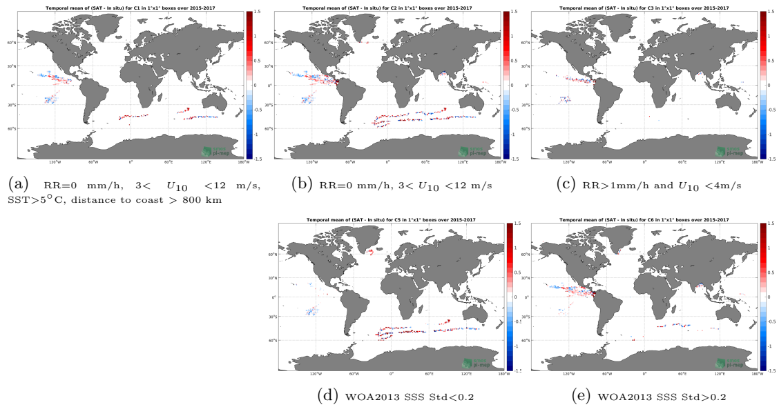
Figure 11: Temporal mean gridded over spatial boxes of size 1^\circ \times 1^\circ of \Delta SSS (SMAP-L2-JPL-V4.3 - Surface drifters) for 5 different subdatasets corresponding to:RR=0 mm/h, 3 < U_{10} < 12 m/s, SST > 5^\circ\text{C} , distance to coast > 800 km (a), RR=0 mm/h, 3 < U_{10} < 12 m/s (b), RR > 1 mm/h and U_{10} < 4 m/s (c), WOA2013 SSS Std < 0.2 (d), WOA2013 SSS Std > 0.2 (e).
