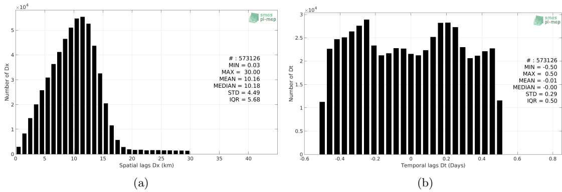
Figure 5: Histograms of the spatial (a) and temporal (b) lags between the time of the Argo measurements and the date of the corresponding SMAP-L2-JPL-V4.3 SSS product.
