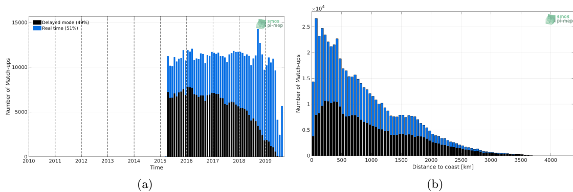
Figure 1: Number of match-ups between Argo and SMAP-L2-JPL-V4.3 SSS as a function of time (a) and as function of the distance to coast (b) over the Global Ocean Pi-MEP region and for the full satellite product period.
