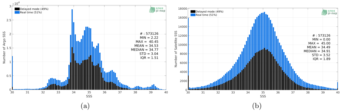
Figure 2: Histograms of SSS from Argo (a) and SMAP-L2-JPL-V4.3 (b) considering all match-up pairs per bins of 0.1 over the Global Ocean Pi-MEP region and for the full satellite product period.
