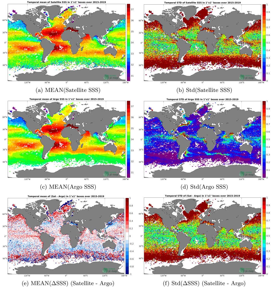
Figure 6: Temporal mean (left) and Std (right) of SSS from SMAP-L2-JPL-V4.3 (top), Argo (middle), and of \Delta SSS (Satellite - Argo). Only match-up pairs are used to generate these maps.
