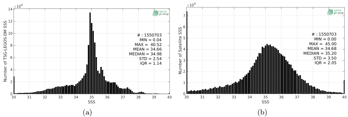
Figure 2: Histograms of SSS from TSG-LEGOS-DM (a) and SMAP-L2-JPL-V4.2 (b) considering all match-up pairs per bins of 0.1 over the Global Ocean Pi-MEP region and for the full satellite product period.
