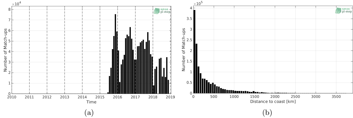
Figure 1: Number of match-ups between TSG-LEGOS-DM and SMAP-L2-JPL-V4.2 SSS as a function of time (a) and as function of the distance to coast (b) over the Global Ocean Pi-MEP region and for the full satellite product period.
