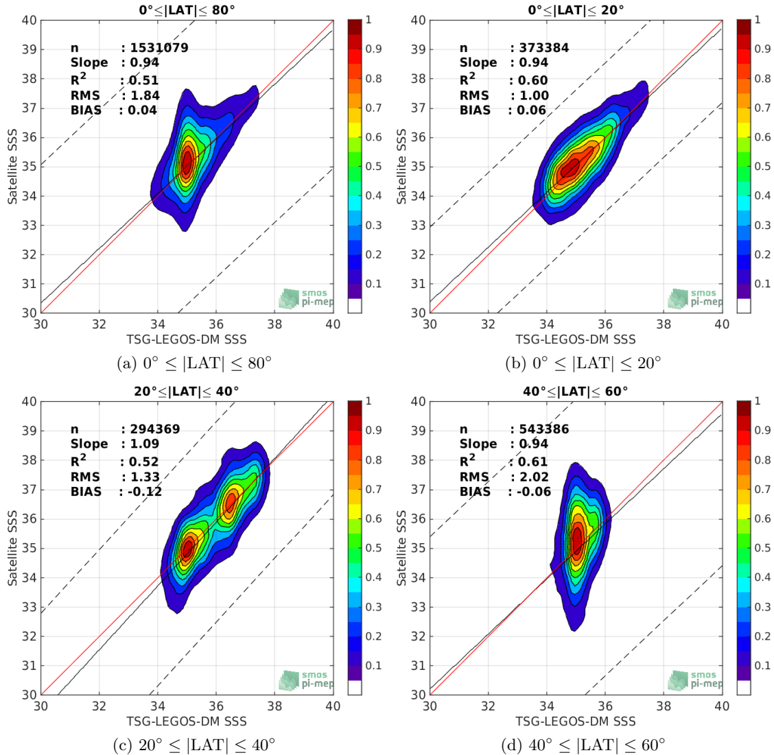
Figure 9: Contour maps of the concentration of SMAP-L2-JPL-V4.2 SSS (y-axis) versus TSG-LEGOS-DM SSS (x-axis) at match-up pairs for different latitude bands. For each plot, the red line shows x=y . The black thin and dashed lines indicate a linear fit through the data cloud and the \pm 95\% confidence levels, respectively. The number match-up pairs n , the slope and R^2 coefficient of the linear fit, the root mean square (RMS) and the mean bias between satellite and in situ data are indicated for each latitude band in each plots.
