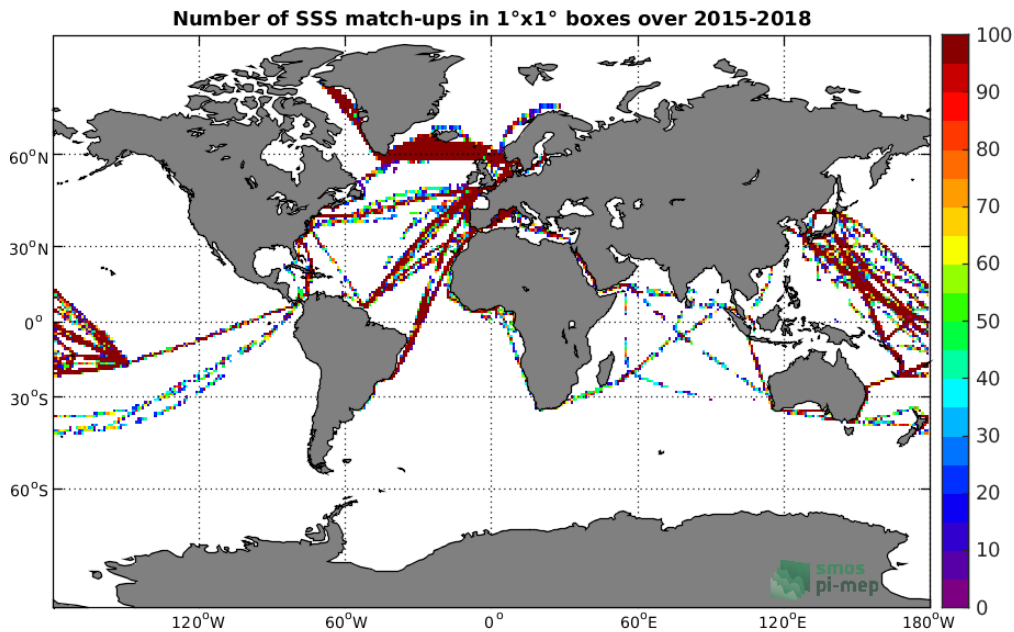
Figure 4: Number of SSS match-ups between TSG-LEGOS-DM SSS and the SMAP-L2-JPL-V4.2 SSS product for the Global Ocean Pi-MEP region over 1^\circ \times 1^\circ boxes and for the full satellite product period.
