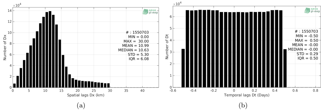
Figure 5: Histograms of the spatial (a) and temporal (b) lags between the time of the TSG-LEGOS-DM measurements and the date of the corresponding SMAP-L2-JPL-V4.2 SSS product.
