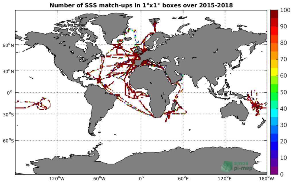
Figure 4: Number of SSS match-ups between TSG-GOSUD-Research-vessel SSS and the SMAP-L2-JPL-V4.2 SSS product for the Global Ocean Pi-MEP region over 1^\circ \times 1^\circ boxes and for the full satellite product period.
