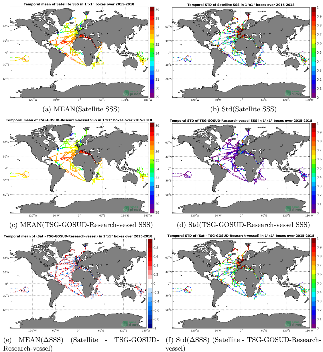
Figure 6: Temporal mean (left) and Std (right) of SSS from SMAP-L2-JPL-V4.2 (top), TSG-GOSUD-Research-vessel (middle), and of \Delta SSS (Satellite - TSG-GOSUD-Research-vessel). Only match-up pairs are used to generate these maps.
