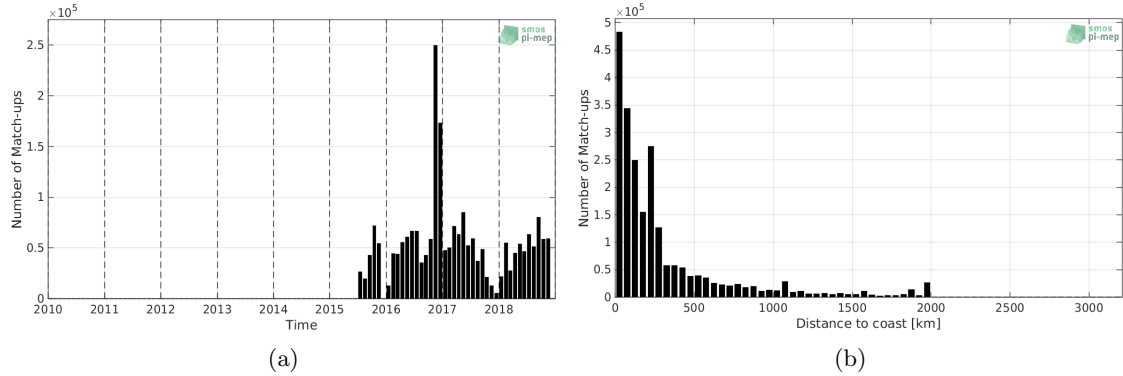
Figure 1: Number of match-ups between TSG-GOSUD-Research-vessel and SMAP-L2-JPL-V4.2 SSS as a function of time (a) and as function of the distance to coast (b) over the Global Ocean Pi-MEP region and for the full satellite product period.
