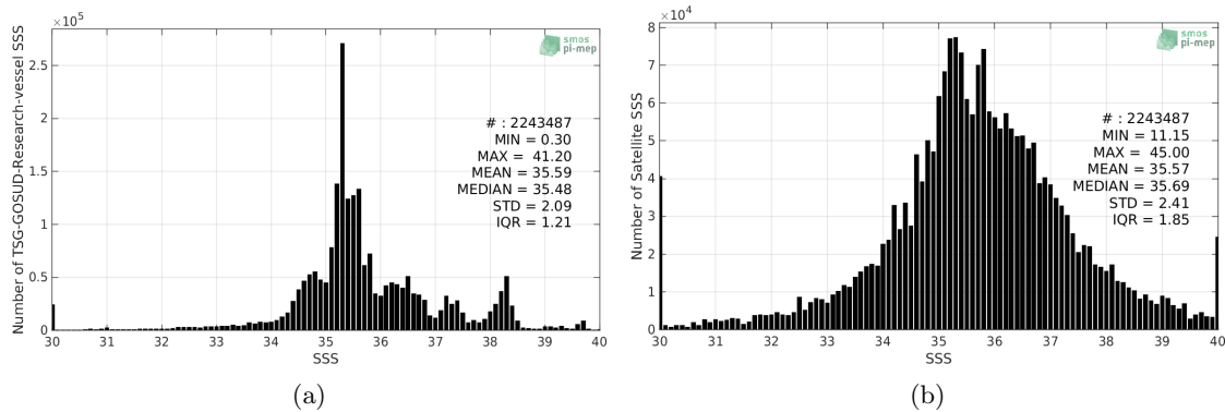
Figure 2: Histograms of SSS from TSG-GOSUD-Research-vessel (a) and SMAP-L2-JPL-V4.2 (b) considering all match-up pairs per bins of 0.1 over the Global Ocean Pi-MEP region and for the full satellite product period.
