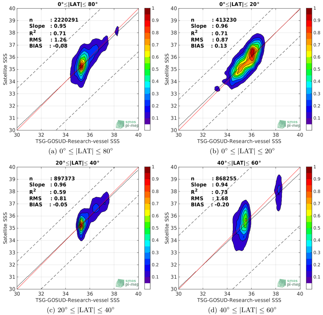
Figure 9: Contour maps of the concentration of SMAP-L2-JPL-V4.2 SSS (y-axis) versus TSG-GOSUD-Research-vessel SSS (x-axis) at match-up pairs for different latitude bands. For each plot, the red line shows x=y . The black thin and dashed lines indicate a linear fit through the data cloud and the \pm 95\% confidence levels, respectively. The number match-up pairs n , the slope and R^2 coefficient of the linear fit, the root mean square (RMS) and the mean bias between satellite and in situ data are indicated for each latitude band in each plots.
