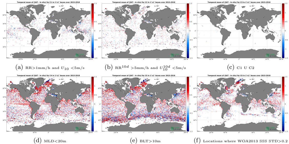
Figure 12: Temporal mean gridded over spatial boxes of size 1^\circ \times 1^\circ of \Delta\text{SSS} (SMAP-L2-JPL-V4.2 - Argo) for 6 different subdatasets corresponding to: \text{RR} > 1\text{mm/h} and U_{10} < 5\text{m/s} (a), \text{RR}^{10d} > 5\text{mm/h} and U_{10}^{10d} < 5\text{m/s} (b), C1 U C2 (c), \text{MLD} < 20\text{m} (d), \text{BLT} > 10\text{m} (e), Locations where WOA2013 SSS \text{STD} > 0.2 (f).
