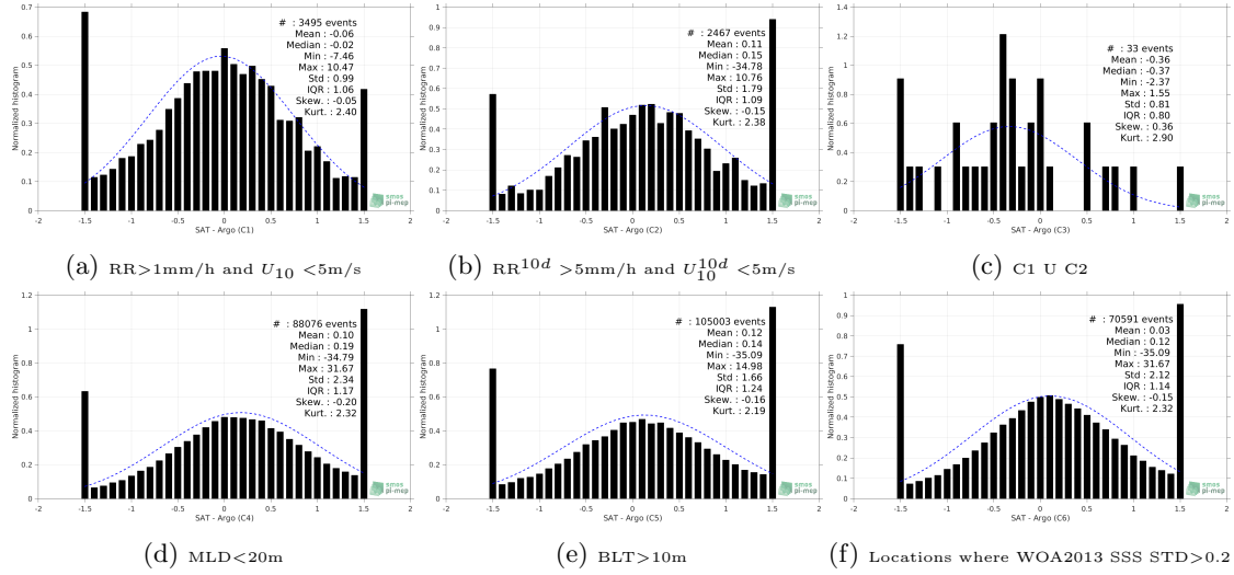
Figure 13: Normalized histogram of \Delta SSS (SMAP-L2-JPL-V4.2 - Argo) for 6 different sub-datasets corresponding to: RR > 1mm/h and U_{10} < 5 m/s (a), RR 10d > 5mm/h and U_{10}^{10d} < 5 m/s (b), C1 U C2 (c), MLD < 20m (d), BLT > 10m (e), Locations where WOA2013 SSS STD > 0.2 (f).
