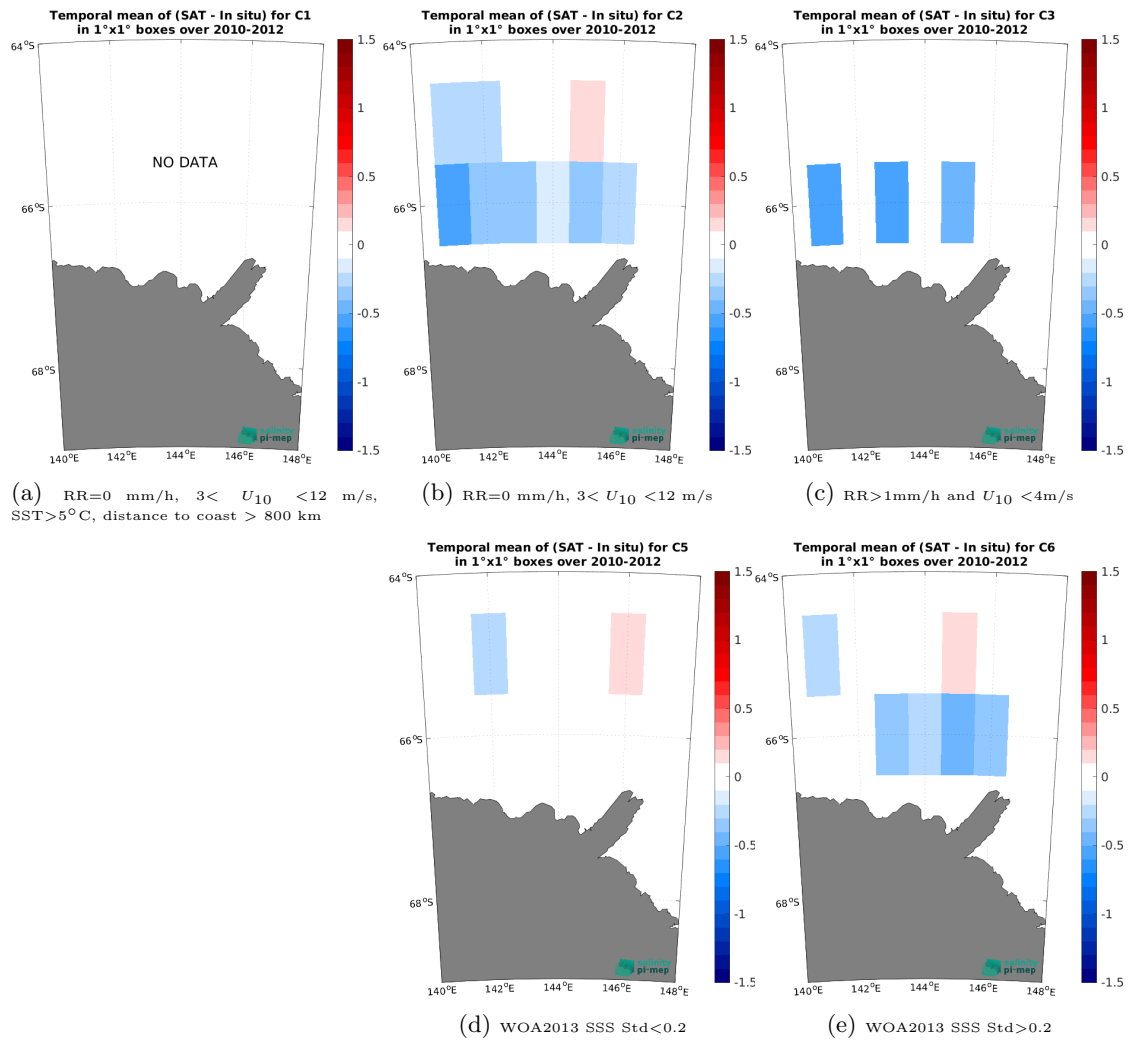
Figure 14: Temporal mean gridded over spatial boxes of size 1^\circ \times 1^\circ of \Delta SSS (ISAS v7 - Monthly (Ifremer-LOPS-CMEMS) - TSG (LEGOS-Surv-Adel)) for 5 different subdatasets corresponding to: RR=0 mm/h, 3 < U_{10} < 12 m/s, SST>5°C, distance to coast > 800 km (a), RR=0 mm/h, 3 < U_{10} < 12 m/s (b), RR>1mm/h and U_{10} < 4 m/s (c), WOA2013 SSS Std<0.2 (d), WOA2013 SSS Std>0.2 (e).
