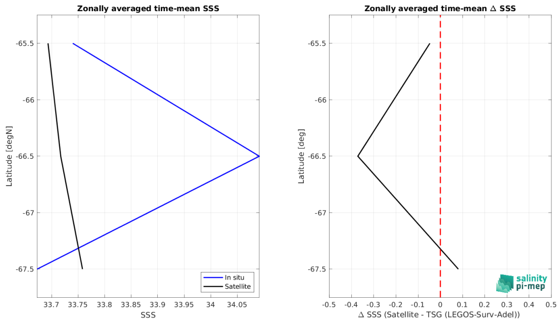
Figure 9: Left panel: Zonal mean SSS from ISAS v7 - Monthly (Ifremer-LOPS-CMEMS) satellite product (black) and from TSG (LEGOS-Surv-Adel) (blue). Right panel: Zonal mean of \Delta SSS (Satellite - TSG (LEGOS-Surv-Adel)) for all the collected Pi-MEP match-up pairs estimated over the full satellite product period.
