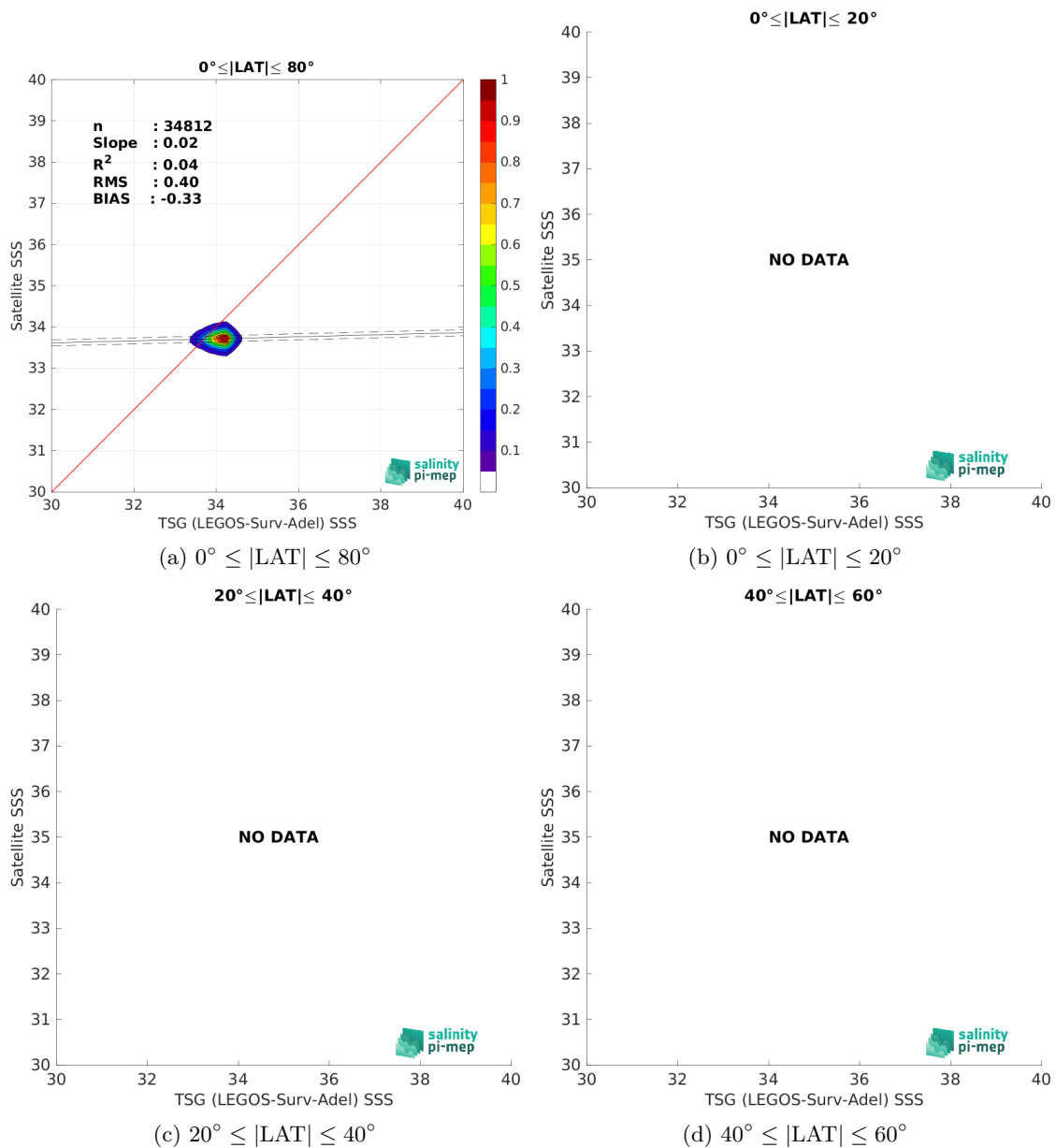
Figure 10: Contour maps of the concentration of ISAS v7 - Monthly (Ifremer-LOPS-CMEMS) SSS (y-axis) versus TSG (LEGOS-Surv-Adel) SSS (x-axis) at match-up pairs for different latitude bands. For each plot, the red line shows x=y . The black thin and dashed lines indicate a linear fit through the data cloud and the \pm 95\% confidence levels, respectively. The number match-up pairs n , the slope and R^2 coefficient of the linear fit, the root mean square (RMS) and the mean bias between satellite and in situ data are indicated for each latitude band in each plots.
