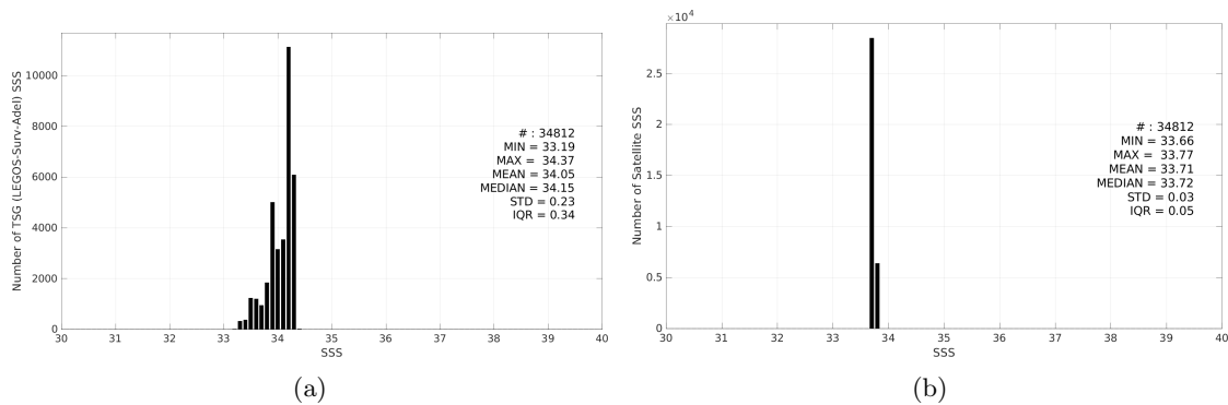
Figure 3: Histograms of SSS from TSG (LEGOS-Surv-Adel) (a) and ISAS v7 - Monthly (Ifremer-LOPS-CMEMS) (b) considering all match-up pairs per bins of 0.1 over the Global Ocean Pi-MEP region and for the full satellite product period.
