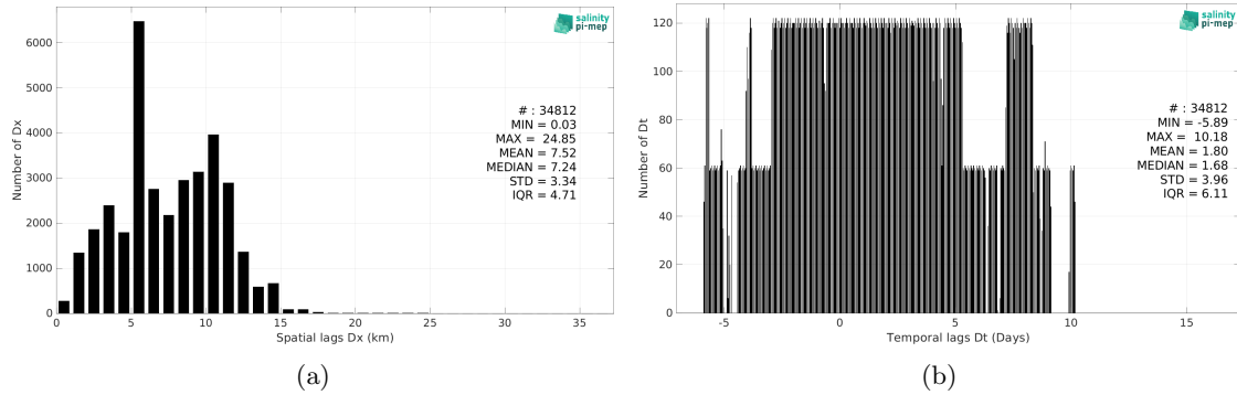
Figure 6: Histograms of the spatial (a) and temporal (b) lags between the location/time of the TSG (LEGOS-Surv-Adel) measurement and the date of the corresponding ISAS v7 - Monthly (Ifremer-LOPS-CMEMS) SSS pixel.
