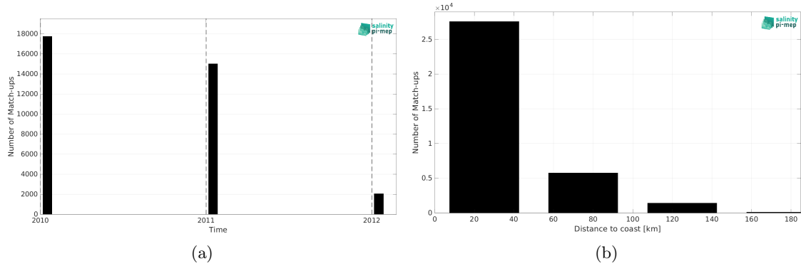
Figure 2: Number of match-ups between TSG (LEGOS-Surv-Adel) and ISAS v7 - Monthly (Ifremer-LOPS-CMEMS) SSS as a function of time (a) and as function of the distance to coast (b) over the Global Ocean Pi-MEP region and for the full satellite product period.
