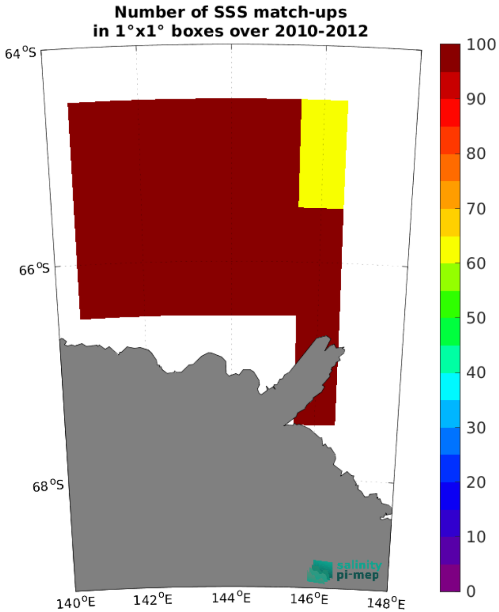
Figure 5: Number of SSS match-ups between TSG (LEGOS-Surv-Adel) SSS and the ISAS v7 - Monthly (Ifremer-LOPS-CMEMS) SSS product for the Global Ocean Pi-MEP region over 1°x1° boxes and for the full satellite product period.
