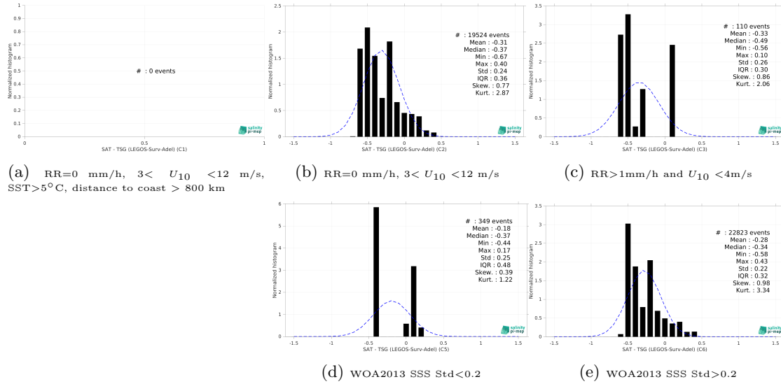
Figure 15: Normalized histogram of \Delta SSS (ISAS v7 - Monthly (Ifremer-LOPS-CMEMS) - TSG (LEGOS-Surv-Adel)) for 5 different subdatasets corresponding to: RR=0 mm/h, 3 < U_{10} < 12 m/s, SST > 5°C, distance to coast > 800 km (a), RR=0 mm/h, 3 < U_{10} < 12 m/s (b), RR > 1mm/h and U_{10} < 4 m/s (c), WOA2013 SSS Std < 0.2 (d), WOA2013 SSS Std > 0.2 (e).
