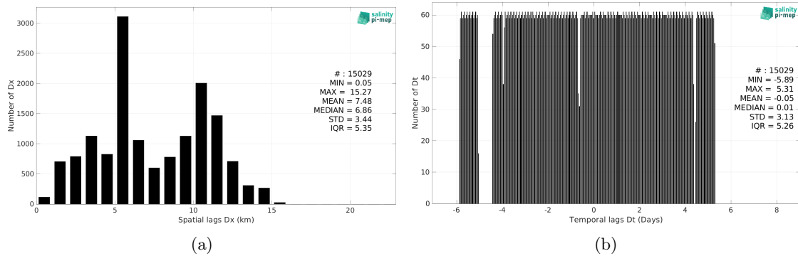
Figure 6: Histograms of the spatial (a) and temporal (b) lags between the location/time of the TSG (LEGOS-Surv-Adel) measurement and the date of the corresponding ISAS SSS pixel.
