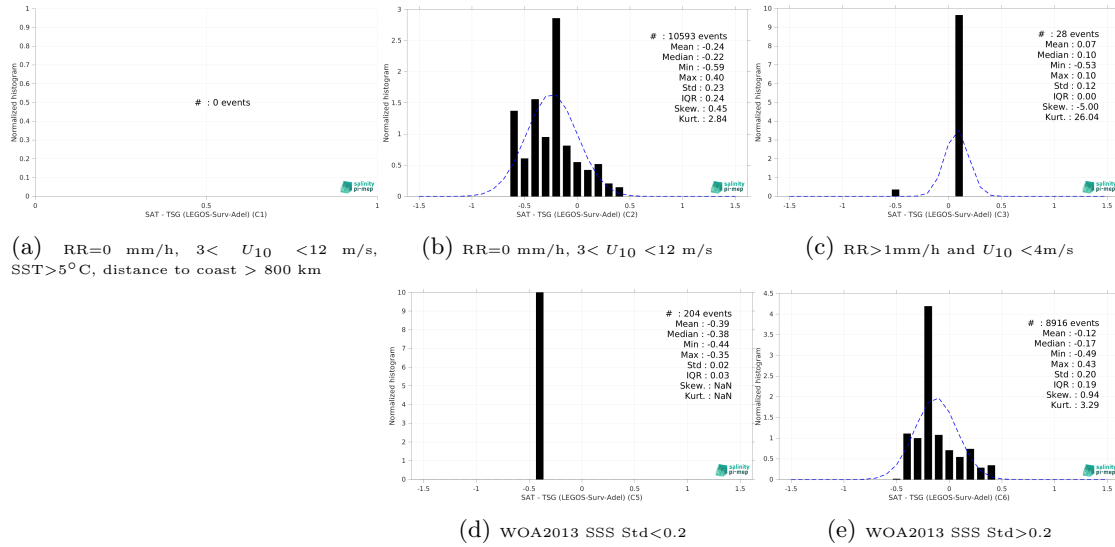
Figure 15: Normalized histogram of \Delta SSS (ISAS - TSG (LEGOS-Surv-Adel)) for 5 different subdatasets corresponding to: RR=0 mm/h, 3 < U_{10} < 12 m/s, SST > 5°C, distance to coast > 800 km (a), RR=0 mm/h, 3 < U_{10} < 12 m/s (b), RR > 1mm/h and U_{10} < 4 m/s (c), WOA2013 SSS Std < 0.2 (d), WOA2013 SSS Std > 0.2 (e).
