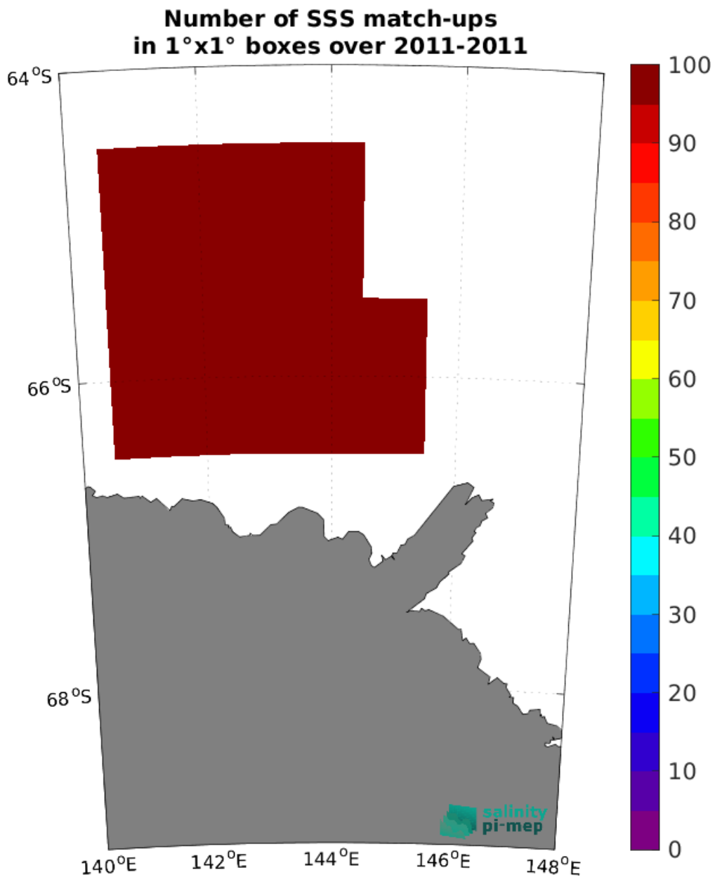
Figure 5: Number of SSS match-ups between TSG (LEGOS-Surv-Adel) SSS and the ISAS SSS product for the Global Ocean Pi-MEP region over 1^\circ \times 1^\circ boxes and for the full satellite product period.
