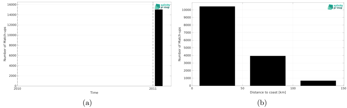
Figure 2: Number of match-ups between TSG (LEGOS-Surv-Adel) and ISAS SSS as a function of time (a) and as function of the distance to coast (b) over the Global Ocean Pi-MEP region and for the full satellite product period.
