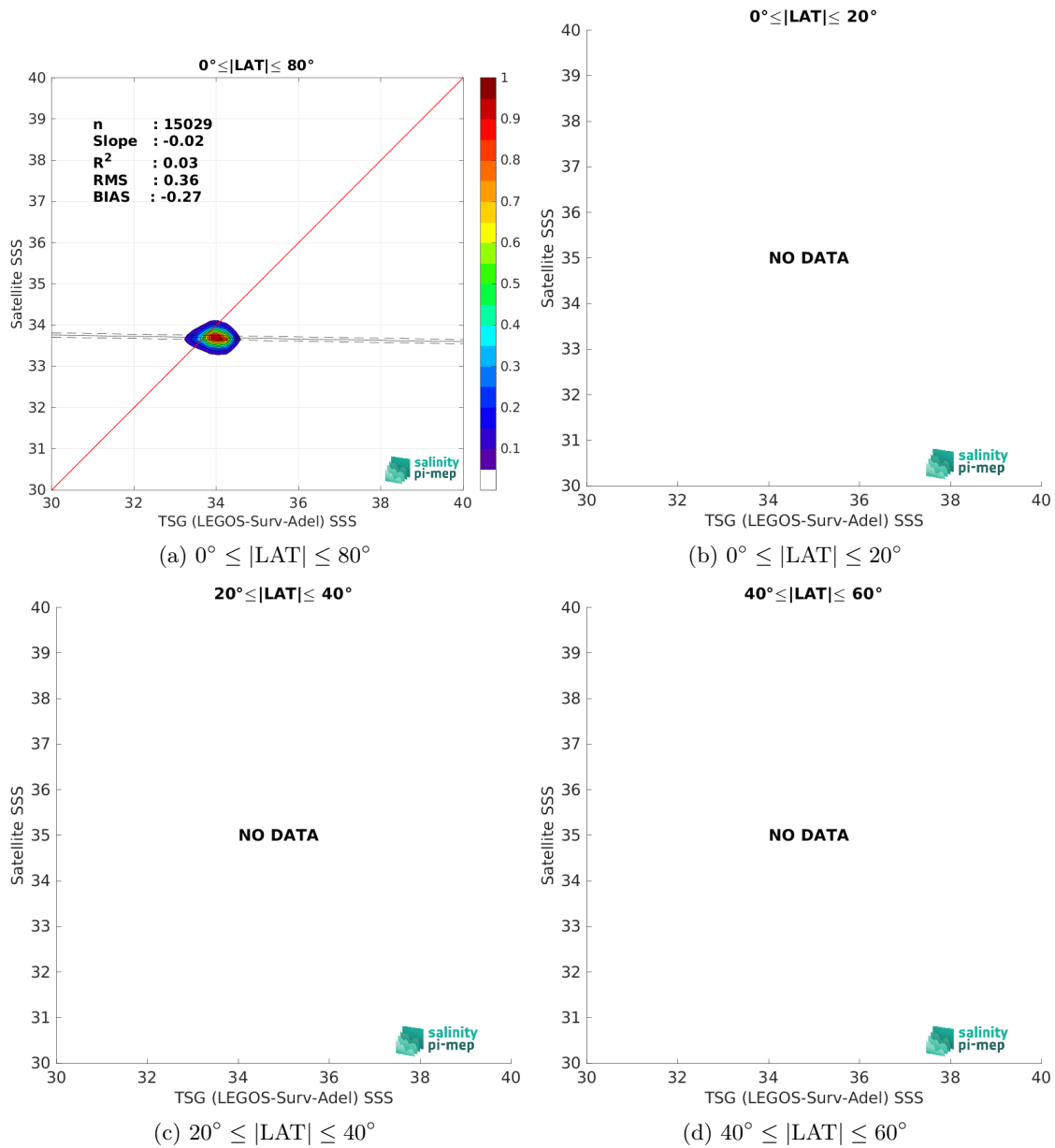
Figure 10: Contour maps of the concentration of ISAS SSS ( y -axis) versus TSG (LEGOS-Surv-Adel) SSS ( x -axis) at match-up pairs for different latitude bands. For each plot, the red line shows x=y . The black thin and dashed lines indicate a linear fit through the data cloud and the \pm 95\% confidence levels, respectively. The number match-up pairs n , the slope and R^2 coefficient of the linear fit, the root mean square (RMS) and the mean bias between satellite and in situ data are indicated for each latitude band in each plots.
