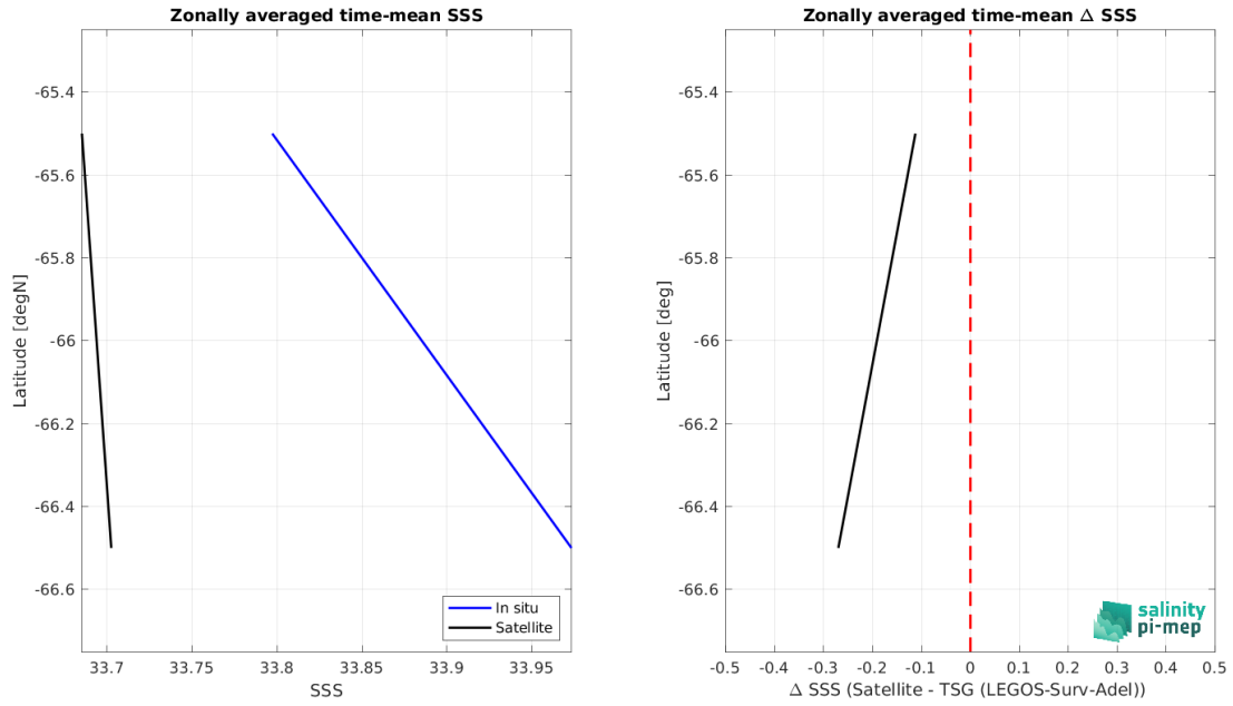
Figure 9: Left panel: Zonal mean SSS from ISAS satellite product (black) and from TSG (LEGOS-Surv-Adel) (blue). Right panel: Zonal mean of \Delta SSS (Satellite - TSG (LEGOS-Surv-Adel)) for all the collected Pi-MEP match-up pairs estimated over the full satellite product period.
