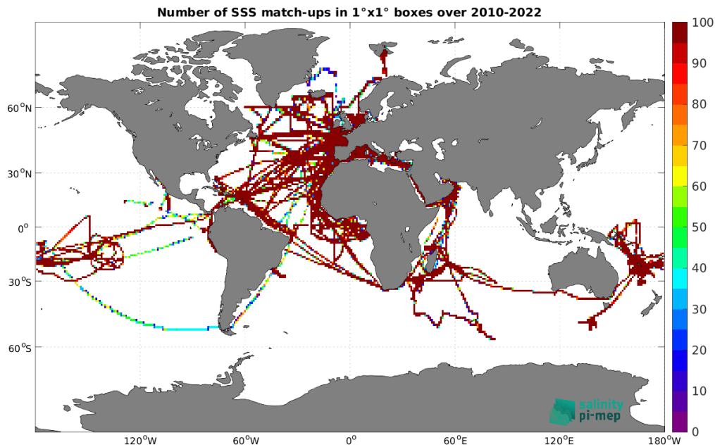
Figure 5: Number of SSS match-ups between TSG (GOSUD-Research-vessel) SSS and the ISAS v7 - Monthly (Ifremer-LOPS-CMEMS) SSS product for the Global Ocean Pi-MEP region over 1^\circ \times 1^\circ boxes and for the full satellite product period.
