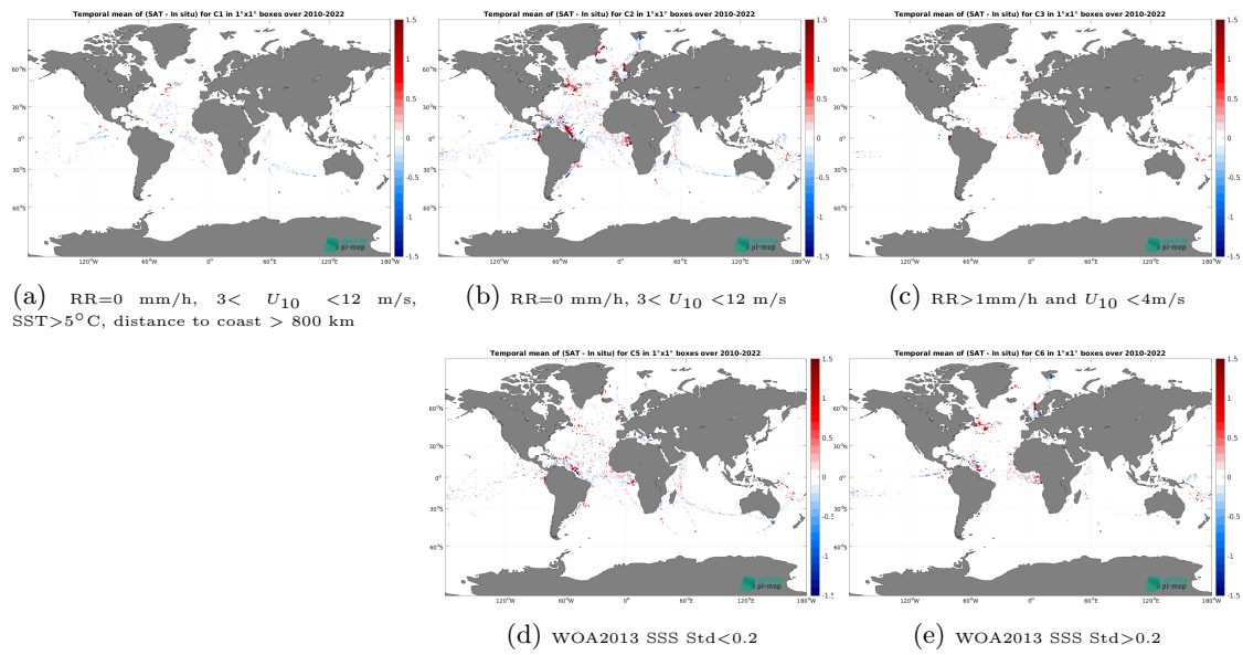
Figure 14: Temporal mean gridded over spatial boxes of size 1^\circ \times 1^\circ of \Delta SSS (ISAS v7 - Monthly (Ifremer-LOPS-CMEMS) - TSG (GOSUD-Research-vessel)) for 5 different subdatasets corresponding to:RR=0 mm/h, 3 < U_{10} < 12 m/s, SST >5^\circ C, distance to coast > 800 km (a), RR=0 mm/h, 3 < U_{10} < 12 m/s (b), RR >1 mm/h and U_{10} < 4 m/s (c), WOA2013 SSS Std <0.2 (d), WOA2013 SSS Std >0.2 (e).
