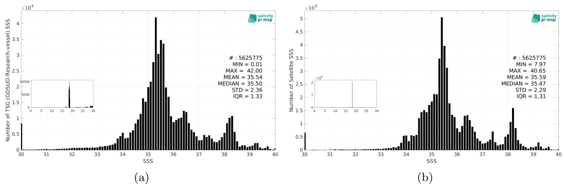
Figure 3: Histograms of SSS from TSG (GOSUD-Research-vessel) (a) and ISAS v7 - Monthly (Ifremer-LOPS-CMEMS) (b) considering all match-up pairs per bins of 0.1 over the Global Ocean Pi-MEP region and for the full satellite product period.
