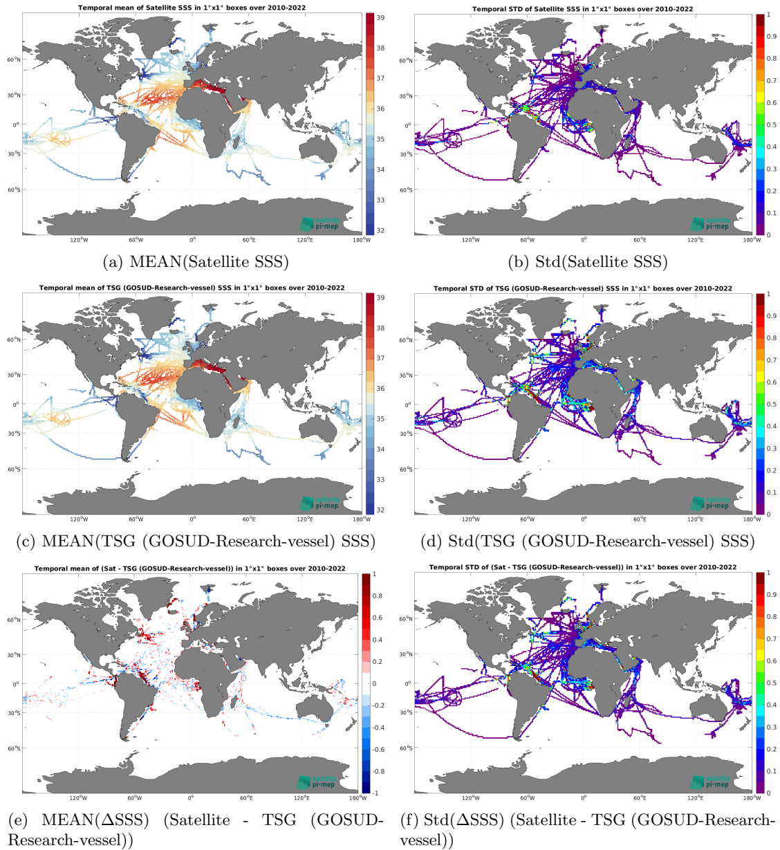
Figure 7: Temporal mean (left) and Std (right) of SSS from ISAS v7 - Monthly (Ifremer-LOPS-CMEMS) (top), TSG (GOSUD-Research-vessel) (middle), and of \Delta SSS (Satellite - TSG (GOSUD-Research-vessel)). Only match-up pairs are used to generate these maps.
