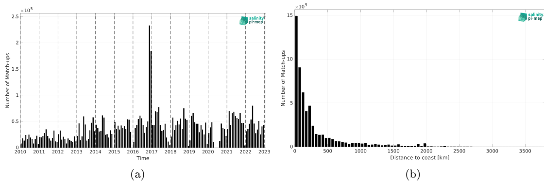
Figure 2: Number of match-ups between TSG (GOSUD-Research-vessel) and ISAS v7 - Monthly (Ifremer-LOPS-CMEMS) SSS as a function of time (a) and as function of the distance to coast (b) over the Global Ocean Pi-MEP region and for the full satellite product period.
