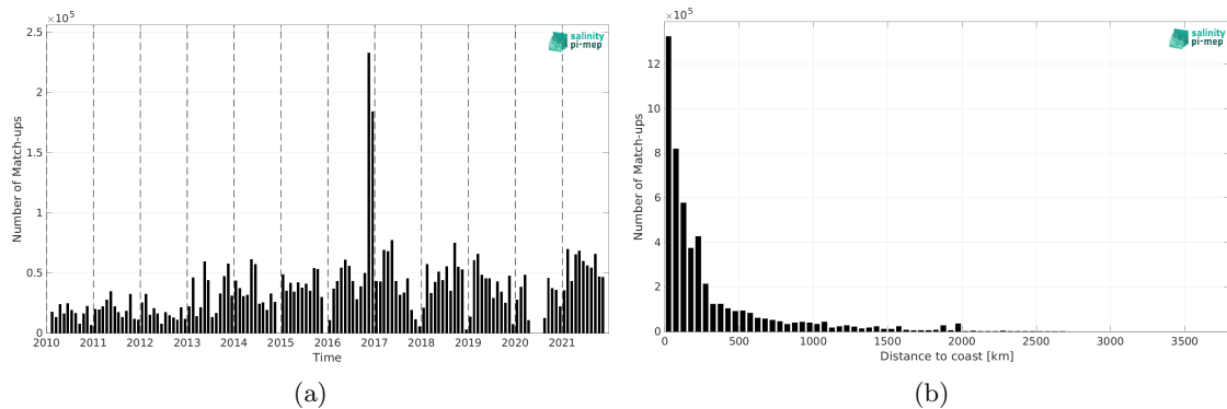
Figure 2: Number of match-ups between TSG (GOSUD-Research-vessel) and ISAS SSS as a function of time (a) and as function of the distance to coast (b) over the Global Ocean Pi-MEP region and for the full satellite product period.
