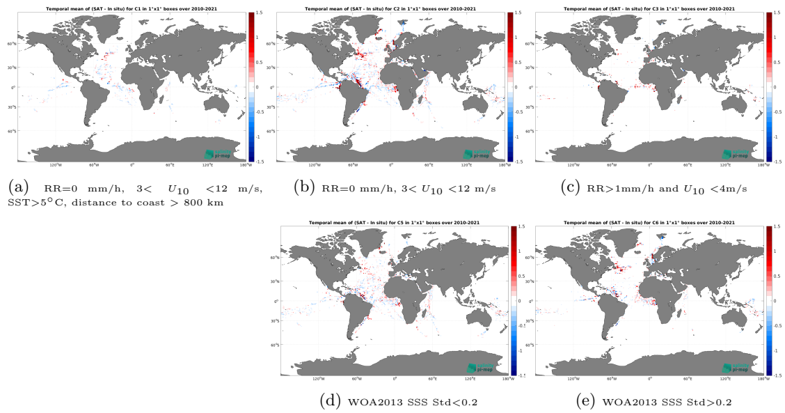
Figure 14: Temporal mean gridded over spatial boxes of size 1^\circ \times 1^\circ of \Delta SSS (ISAS - TSG (GOSUD-Research-vessel)) for 5 different subdatasets corresponding to:RR=0 mm/h, 3 < U_{10} < 12 m/s, SST >5^\circ C, distance to coast > 800 km (a), RR=0 mm/h, 3 < U_{10} < 12 m/s (b), RR >1 mm/h and U_{10} < 4 m/s (c), WOA2013 SSS Std <0.2 (d), WOA2013 SSS Std >0.2 (e).
