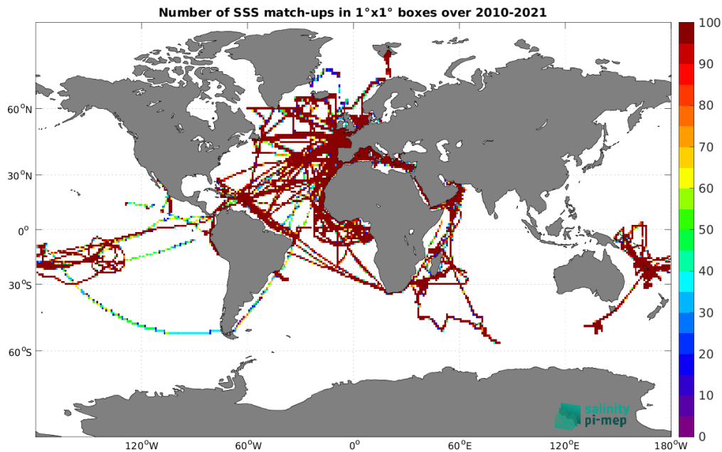
Figure 5: Number of SSS match-ups between TSG (GOSUD-Research-vessel) SSS and the ISAS SSS product for the Global Ocean Pi-MEP region over 1^\circ \times 1^\circ boxes and for the full satellite product period.
